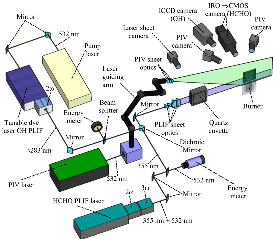
Fig. 1 Photograph and scheme of the experimental setup
