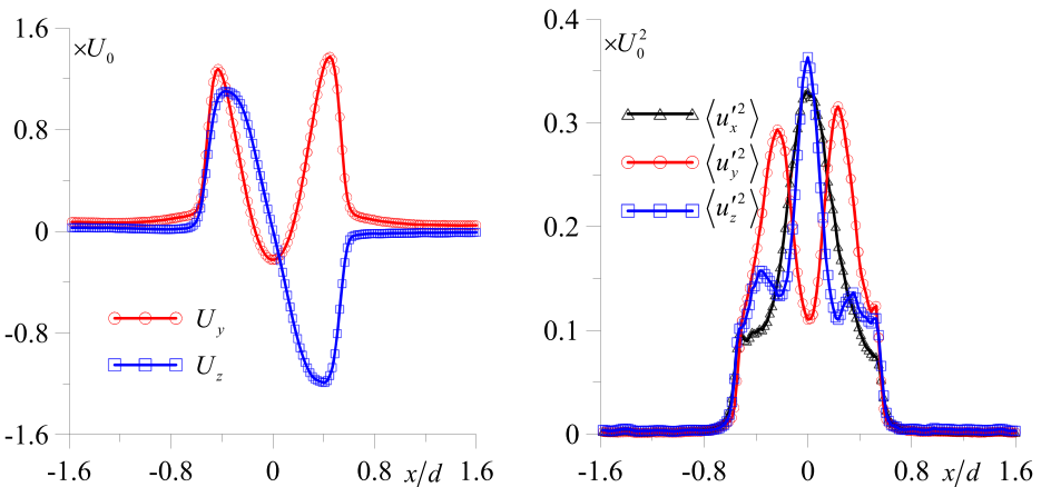
Fig. 18 Distribution of the mean velocity and deviations of the velocity fluctuations near the nozzle exit ( y/d \approx 0.1 ) of the high-swirl jet
