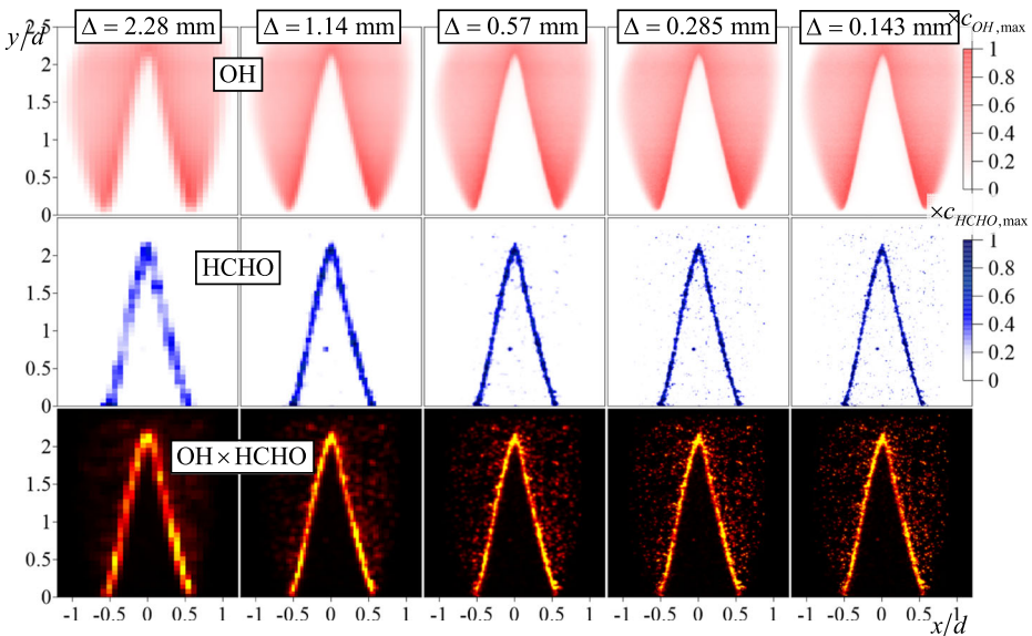
Fig. 20 Effect of the spatial resolution ( \Delta is the window size) on the instantaneous snapshots of the PLIF data for the Bunsen flame. c_{\text{HCHO,max}} = 1830 , c_{\text{OH,max}} = 31800
