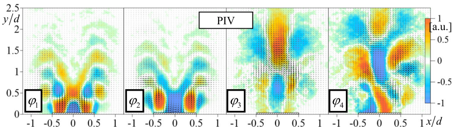
Fig. 8 Spatial distributions of the first four POD modes for the non-reacting swirling jet
