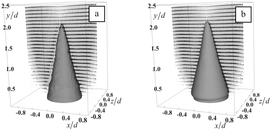
Fig. 4 3D visualization of the flame front for the Bunsen flame. (a) OH × HCHO PLIF signal, (b) positive divergence of the velocity field ( \text{div}U = 4 U_0/d )
