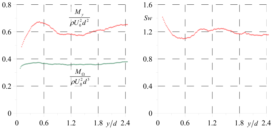
Fig. 19 Axial fluxes of the jet’s angular and axial momenta and the swirl rate long the high-swirl jet
