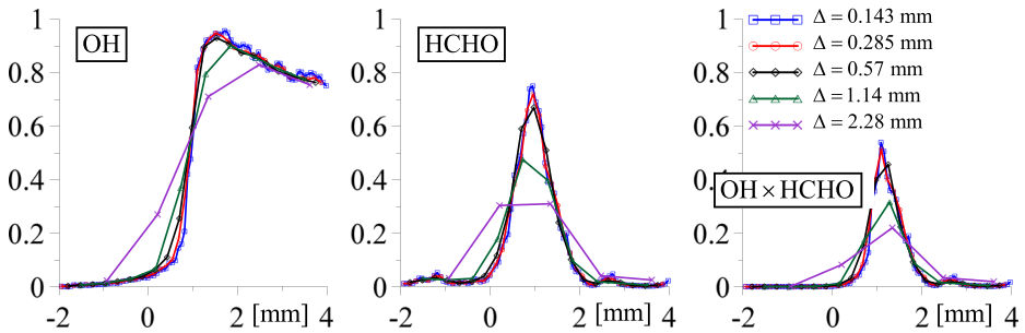
Fig. 21 Profiles of the PLIF intensity across the front of the Bunsen flame for various spatial resolutions
