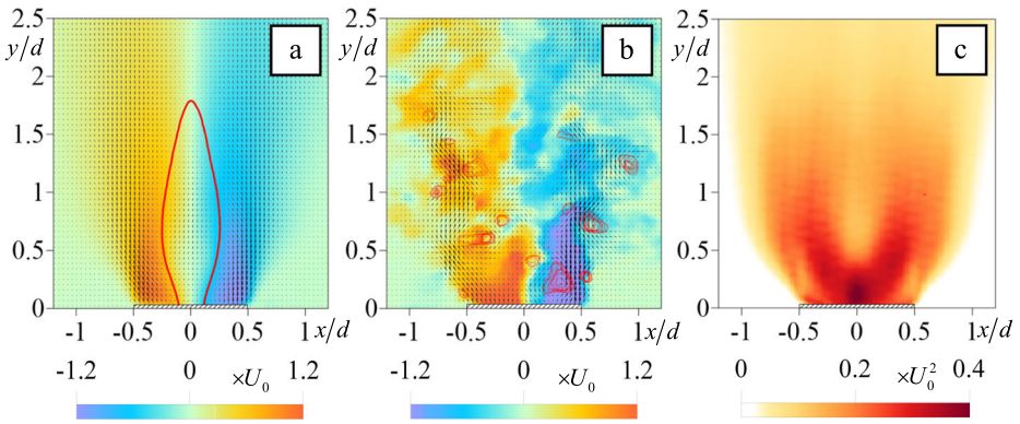
Fig. 5 Distributions of the (a) time-averaged (solid line shows a contour of U_y=0 ) and (b) instantaneous (solid lines show contours of Q^{2D}=4(2+n)U_0^2d^{-2} , where n is a positive integer) velocity fields and (c) the turbulent kinetic energy in the non-reacting swirling jet
