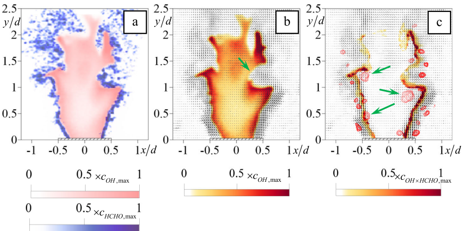
Fig. 15 Instantaneous snapshot of the PIV and PLIF data for the fuel-lean premixed flame ( \Phi = 0.7 ). (a) OH PLIF and HCHO PLIF, (b) PIV and OH PLIF, (c) PIV and OH \times HCHO PLIF (the solid lines correspond to Q^{2D} > 4(2 + n)U_0^2 d^{-2} ). c_{HCHO,max} = 1360 , c_{OH,max} = 10,200
