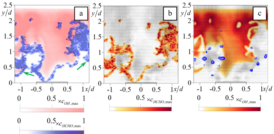
Fig. 10 Instantaneous snapshot of the PIV and PLIF data for the fuel-rich lifted flame ( \Phi = 2.5 ). (a) OH PLIF and HCHO PLIF, (b) PIV and HCHO PLIF, (c) PIV and OH PLIF (solid lines correspond to Q^{2D} > 3.1(2+n)U_0^2d^{-2} ). c_{HCHO,max} = 1360 , c_{OH,max} = 25,600
