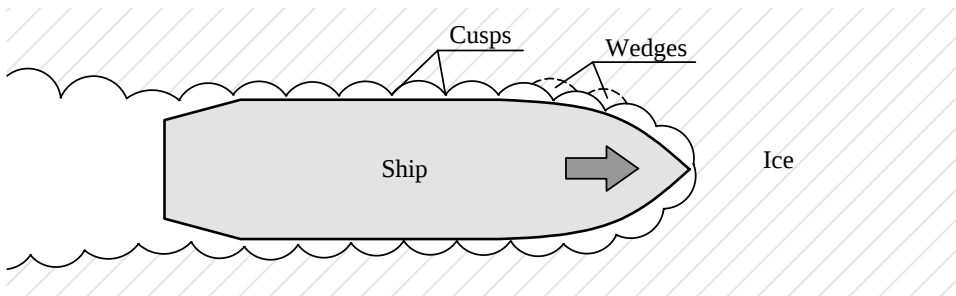
Figure 2.1: As the vessel advances, it mainly interacts with the ice sheet through a series of cusps. Each cusp fails in bending, generating wedges. This process results in an ice edge pattern that is typical for the edge tracking models.
