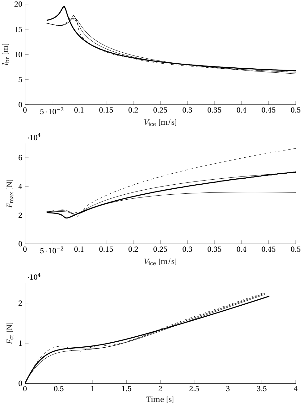
Figure 5.3: The effect of C_{bc} on the predictions of \mathcal{M}_{eHD} . The bold curve is \mathcal{M}_{HD} . The dashed curve shows \mathcal{M}_{eHD}(\{C_m = 6.26, \xi_d = 1.06, C_{bc} = 0\}) \neq \mathcal{M}_{HS} . All subsequent solid curves are evaluations at C_{bc} = \{4, 8\} \times 10^{-6} \text{ m}^2 respectively. For the bottom graph V_{ice} = 0.04 \text{ m/s} .
