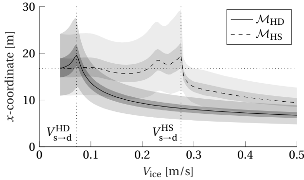
Figure 4.21: The sensitivity of l_{\text{br}}(V_{\text{ice}}) to defects for both models. The solid and dashed line indicate the location of the deterministic breaking lengths as previously shown in Fig. 4.17. Therefore, on these lines \sigma_{\text{norm}}(l_{\text{br}}(V_{\text{ice}})) = 1 . The dark grey shading indicates the segment of the ice wherein \sigma_{\text{norm}}(x) \geq 0.99 and light gray \sigma_{\text{norm}}(x) \geq 0.90 for both models. The horizontal dotted line indicates the static breaking length l_{\text{br},s} computed with Eq. (4.19).
