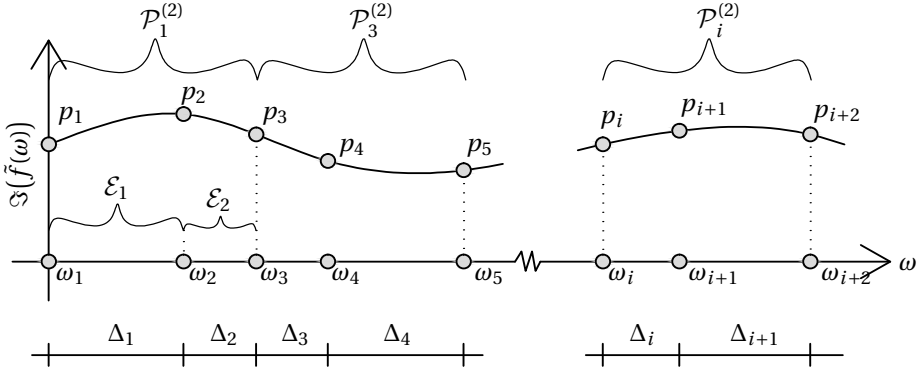
Figure B.1: \Im(\tilde{f}(\omega)) is approximated using N_p second order polynomials \mathcal{P}_i^{(2)} that are indexed with i . Each polynomial is constructed using the elements \mathcal{E}_i and \mathcal{E}_{i+1} that depend on the set of points \{p_i, p_{i+1}, p_{i+2}\} .
