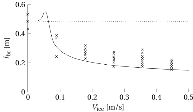
Figure 4.9: The breaking length as a function of the ice velocity l_{\text{br}}(V_{\text{ice}}) . The crosses represent the experimental data. The curve shows the values predicted by the proposed model. The dotted line is the static breaking length.
