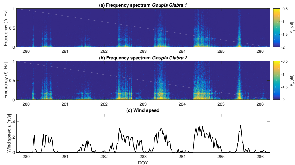
Figure 5. Frequency spectra of Goupia glabra trees nos. 1 and 2 over time from DOY 280 to 286 (9 to 15 October 2015).
