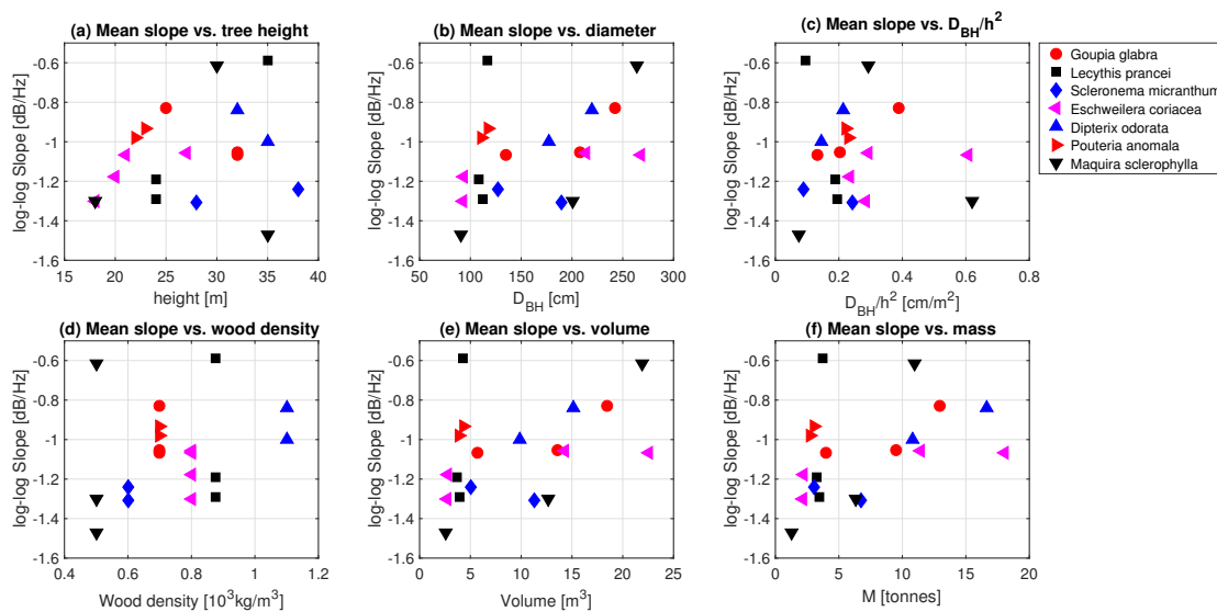
Figure 6. Mean slope between 0.2 and 1 Hz for each tree, plotted against (a) height; (b) diameter at breast height ( D_{BH} ); (c) D_{BH}/h^2 ; (d) wood density; (e) cylindric volume; and (f) cylindric mass.
