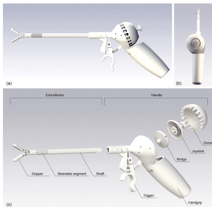
Figure 2. Design of 3D-GriP. (a) Side view; (b) Back view; (c) Exploded view with the names of the parts indicated.
