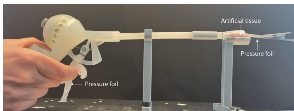
Figure 11. Set-up of the grasping force measurement.
