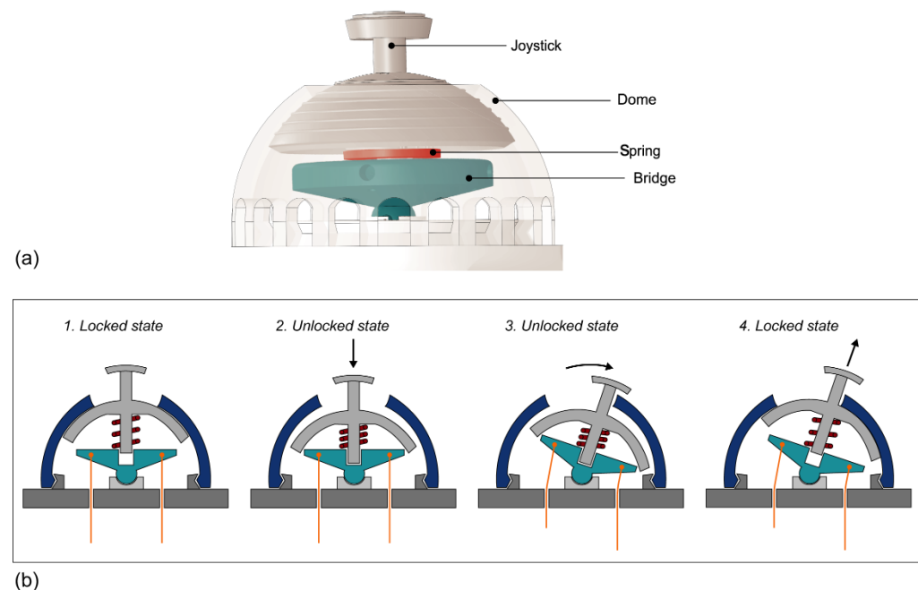
Figure 5. Working principle of the steering mechanism. (a) Three-dimensional (3D) render of the assembled joystick, showing the joystick, the dome (transparent to show the underlying components), bridge (blue), and spring (red). (b) Schematic drawing of the working principle of the friction lock showing the bridge (blue), spring (red), and cables (orange). (1)–(4) show the actions taken to move and lock the steerable segment.
