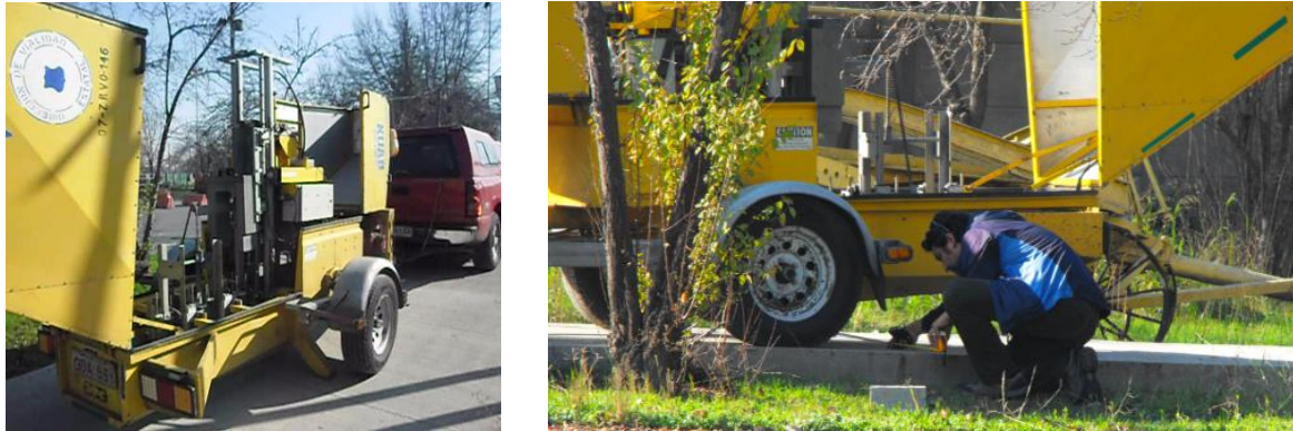
Fig 6.5.3. Application of load repetitions with the FWD on an uncracked joint
