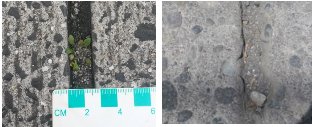
Fig. 7.3.1. Joint contamination at the apron of Eindhoven airport, the Netherlands (left) – contamination and joint spalling of an urban street, Cabrerio city, Chile (right)
