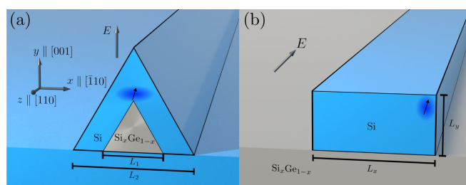
FIG. 1. Design of valley-free fins in Si/Si x Ge 1-x heterostructures. (a) Equilateral triangular fin with inner and outer side lengths L_1 and L_2 , respectively. The wave function is localized in the Si shell by uniaxial strain and the electric field E . The fin is assumed to be grown on a Si substrate, but the results are similar for a Ge substrate. (b) Rectangular Si slab with side lengths L_x and L_y on Si x Ge 1-x substrate. The electrons are confined at the corners by E in the x - y plane. The blue dots show the position of the QD hosting the spin qubit. We assume infinitely long systems in the z direction. The coordinate system in (a) shows the crystallographic growth directions for both geometries.
