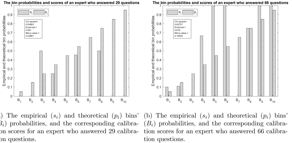
Figure 9: Examples of the empirical ( s_i ) and theoretical ( p_i ) bins' ( B_i ) probabilities and corresponding calibration scores.
