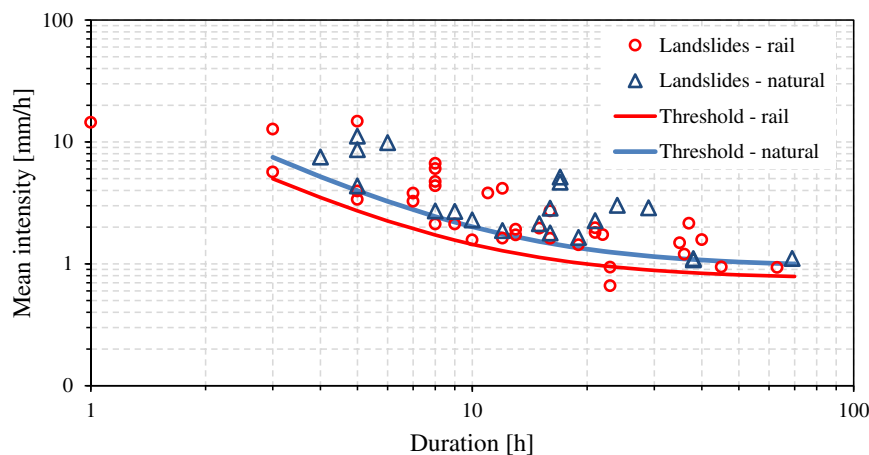
Fig. 7. I-D rainfall thresholds for engineered slopes for rail network (red line) and for landslides on natural terrain in Ireland (blue line).
