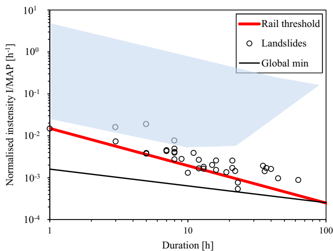
Fig. 10. I_{MAP} -D threshold for landslides on rail earthworks in Ireland. Shaded area – extent of I_{MAP} -D thresholds collated by Guzzetti et al. (2007). Global minimum I_{MAP} -D threshold – thin black line (Guzzetti et al., 2008).
