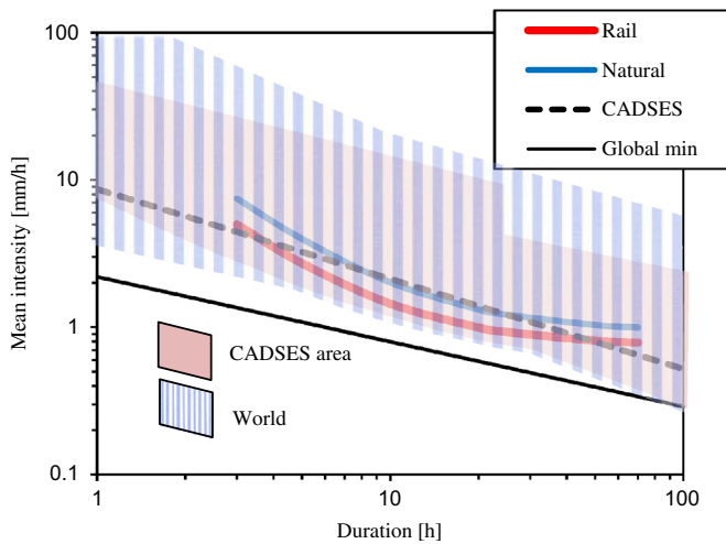
Fig. 9. Range of thresholds collated by Guzzetti et al. (2007) in a) CADSES area (red) and b) world (striped blue). Thresholds for rail earthworks (red line, thicker) and natural slopes (blue line, thinner); thresholds for CADSES area (Guzzetti et al., 2007, dashed black line) and global threshold (thin black line Guzzetti et al., 2008) superimposed.
