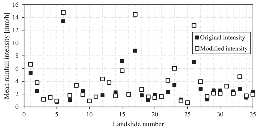
Fig. 4. Distribution of original rainfall intensities from synoptic stations ( I_{ss} ) and modified intensities ( I ).
