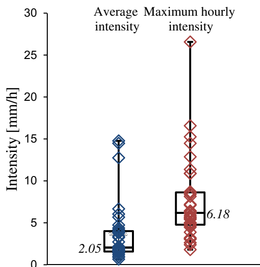
Fig. 3. Distribution of average and maximum hourly intensities for 35 landslides on Irish rail earthworks, with boxes denoting the median value (in text), first and third quartile.
