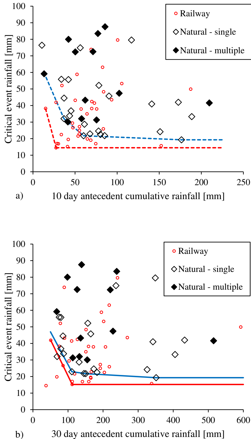
Fig. 8. Cumulative – antecedent rainfall thresholds for landslides on rail network (red line) and landslides on natural terrain (blue line): a) 10 day antecedent period and b) 30 day antecedent period. Landslide events on rail network in red circles. Landslide events on natural terrain in black diamonds. Empty diamond – single landslide event, full diamond – multiple (widespread) landslide event.
