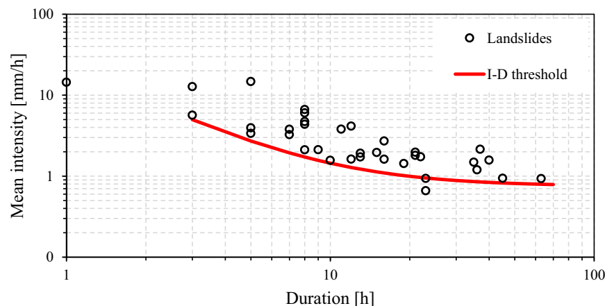
Fig. 5. I-D threshold for landslides on Irish Rail network.
