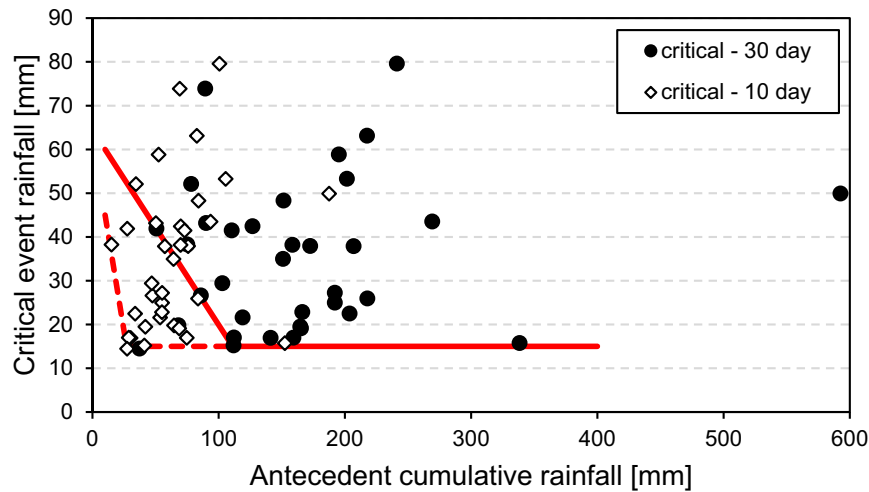
Fig. 6. Critical event rainfall – cumulative antecedent rainfall threshold. Threshold for 10 day antecedent rainfall in dashed red line, threshold for 30 day antecedent rainfall in solid red line.
