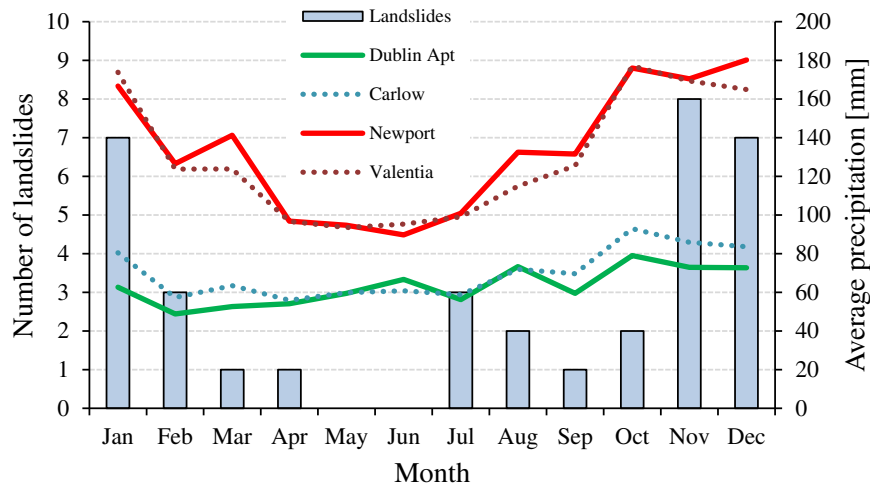
Fig. 2. Monthly distribution of landslides on railway earthworks and average monthly precipitation values for four synoptic station in Ireland.
