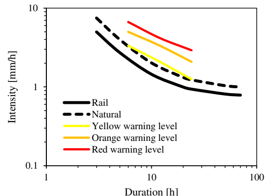
Fig. 11. I-D thresholds for landslides in Ireland and Met.ie rainfall warning levels.
