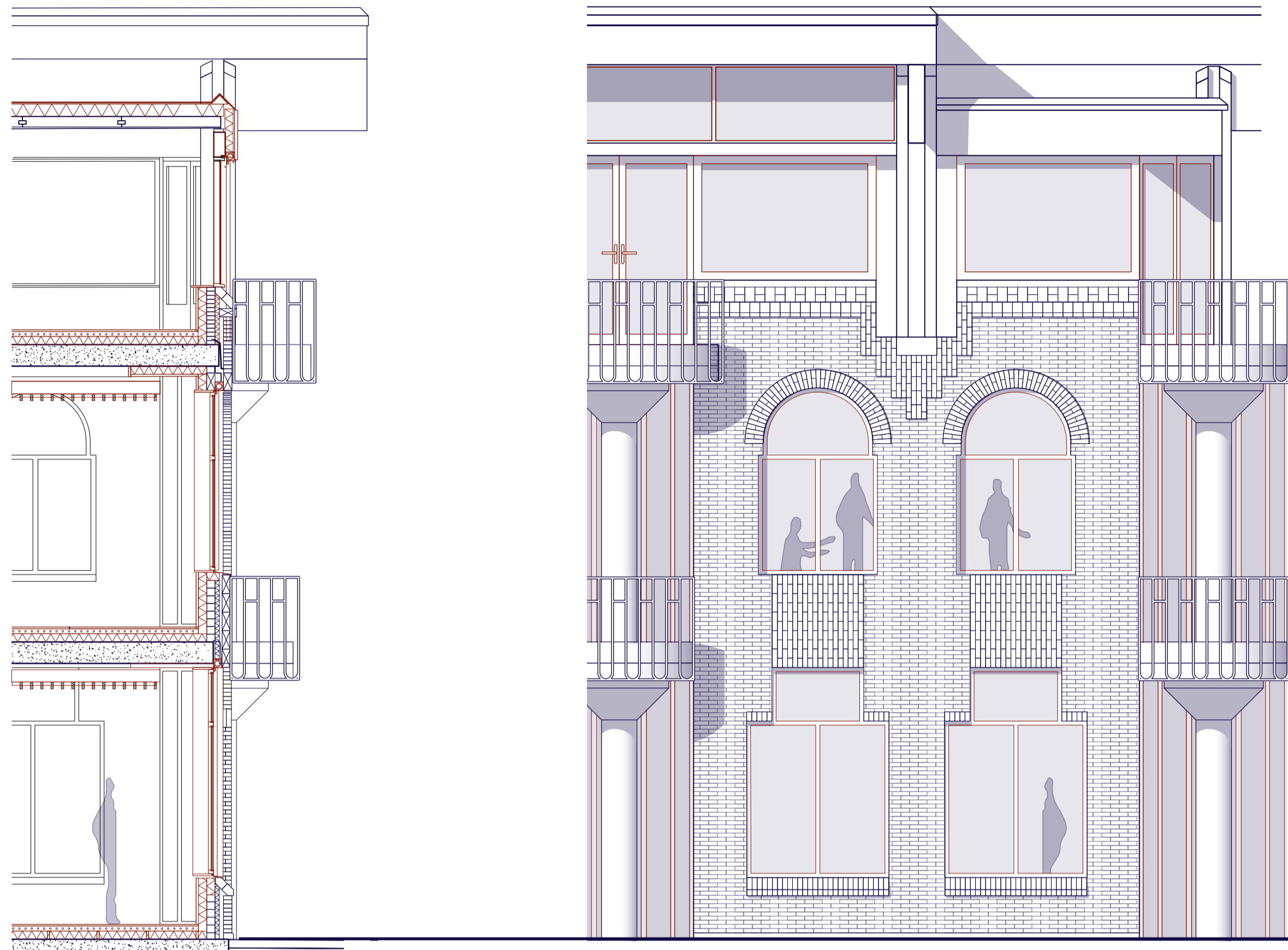
FACADE SECTION AND ELEVATION // 1:50
