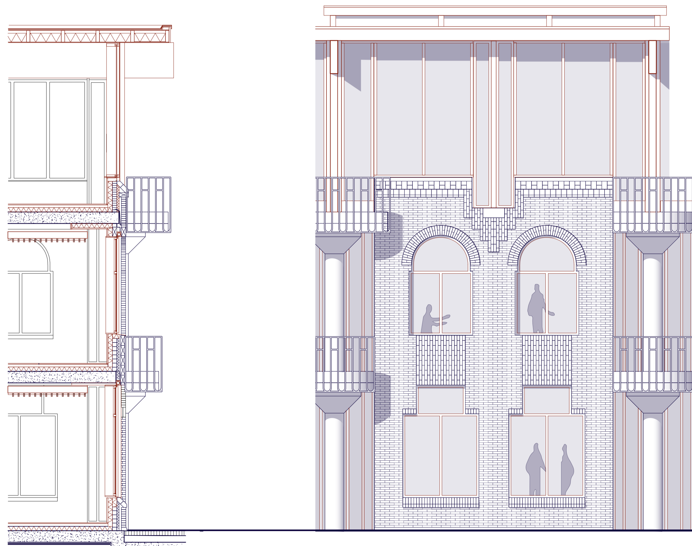
FACADE SECTION AND ELEVATION // 1:50
