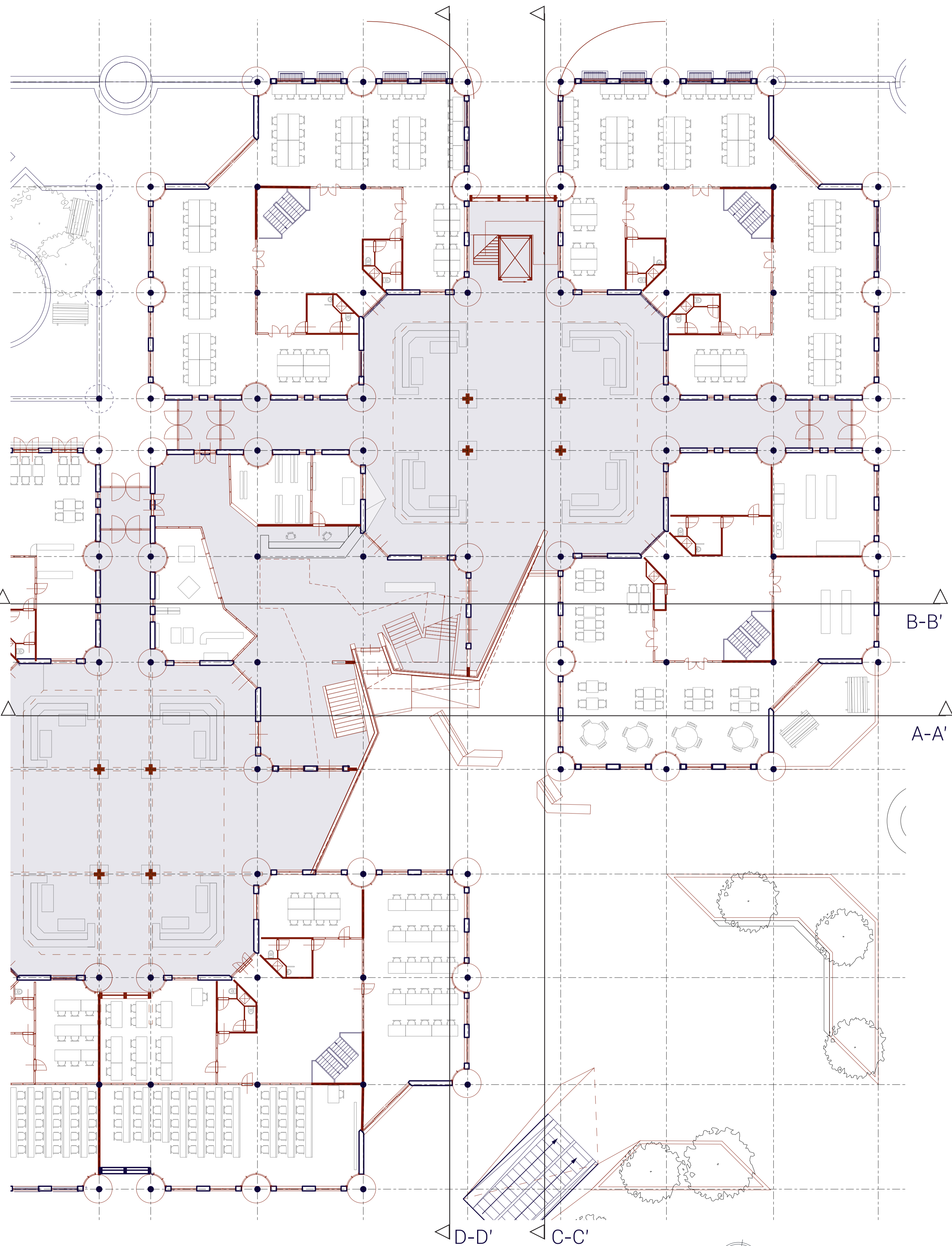
PLAN GROUND FLOOR SOUTH CLUSTER // 1:200
