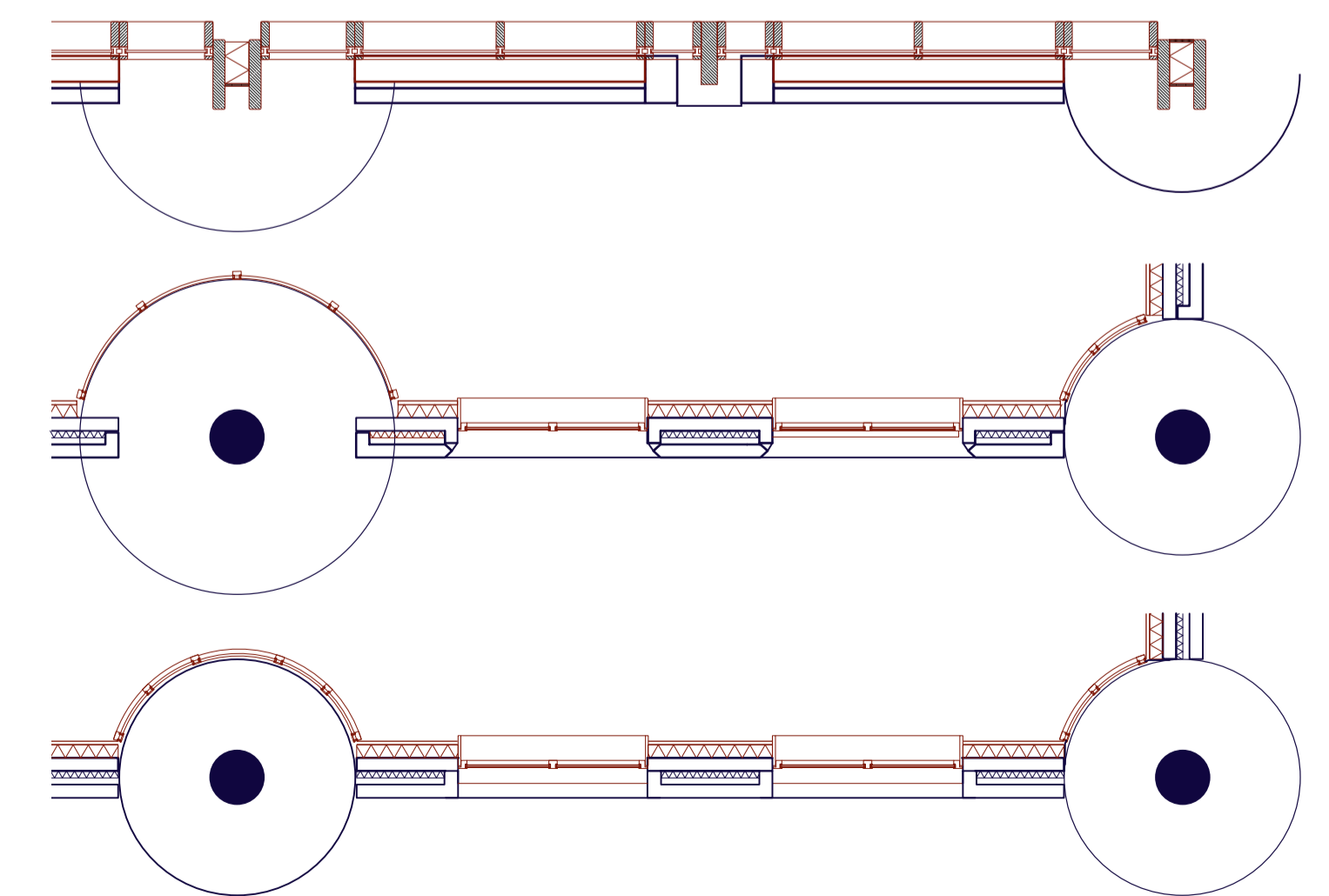
HORIZONTAL FACADE DETAIL // 1:50
