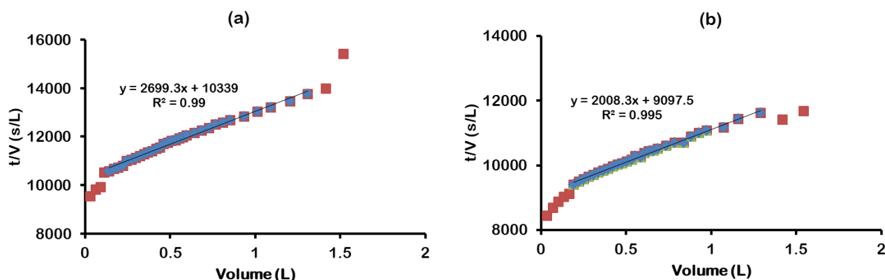
Fig. 8. Determination of MFI for (a) unfiltered, and (b) 0.45 µm filtered samples using best-fit regression lines.
