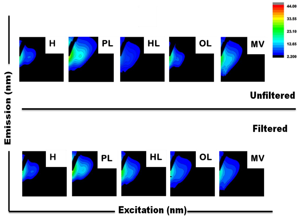
Fig. 3. Top panel shows EEMs for unfiltered water samples while the bottom panel shows EEMs for 0.45 \mu\text{m} filtered water samples.
