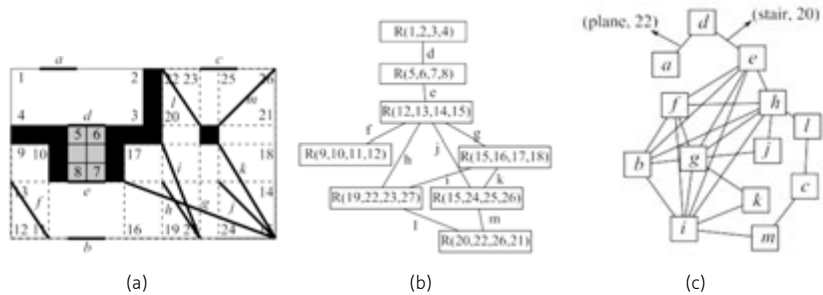
FIGURE 2.25 The LEGO graph. (a) Subdivided blocks of a floor; (b) The graph representing the connectivity of blocks; and (c) The resulting LEGO graph (from [YS11]).
