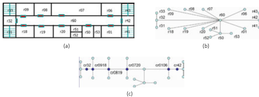
FIGURE 2.8 A 2D network created on the basis of Poincare Duality, Media Axis Transform and information about doors. (a) Floor plan; (b) The metric network based on connectivity of spaces; and (c) The metric network considering door locations (from [MZP05]). The nodes cr32, cr0918, cr0819, cr0720, cr0106, cr42 represent precise geometric locations in the space related to node r60 (in subfigure (b)).
