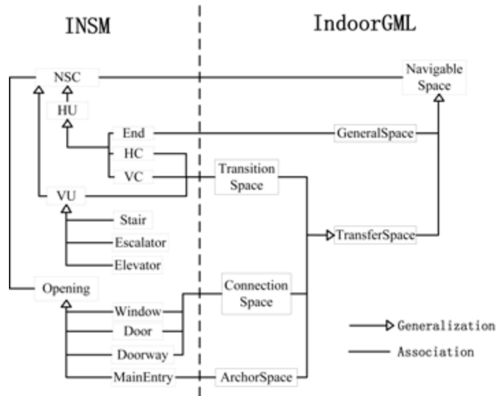
FIGURE 3.11 The associations of essential semantics of the INSM and the IndoorGML .
