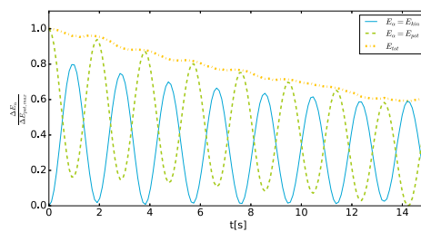
Fig. 4. Total, kinetic and potential energy in standing wave.
