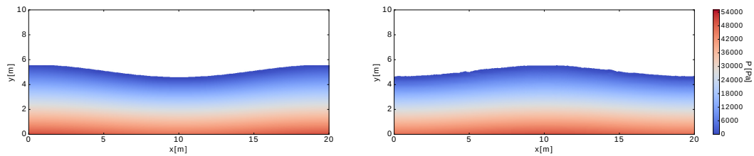
Fig. 2. Pressures in the water phase of a standing wave with H/d = 0.1 at t = 0 s (left panel) and t = 5.5 s (right panel).
