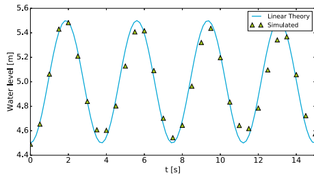
Fig. 3. Theoretical and simulated surface elevation at x = 0.5L .
