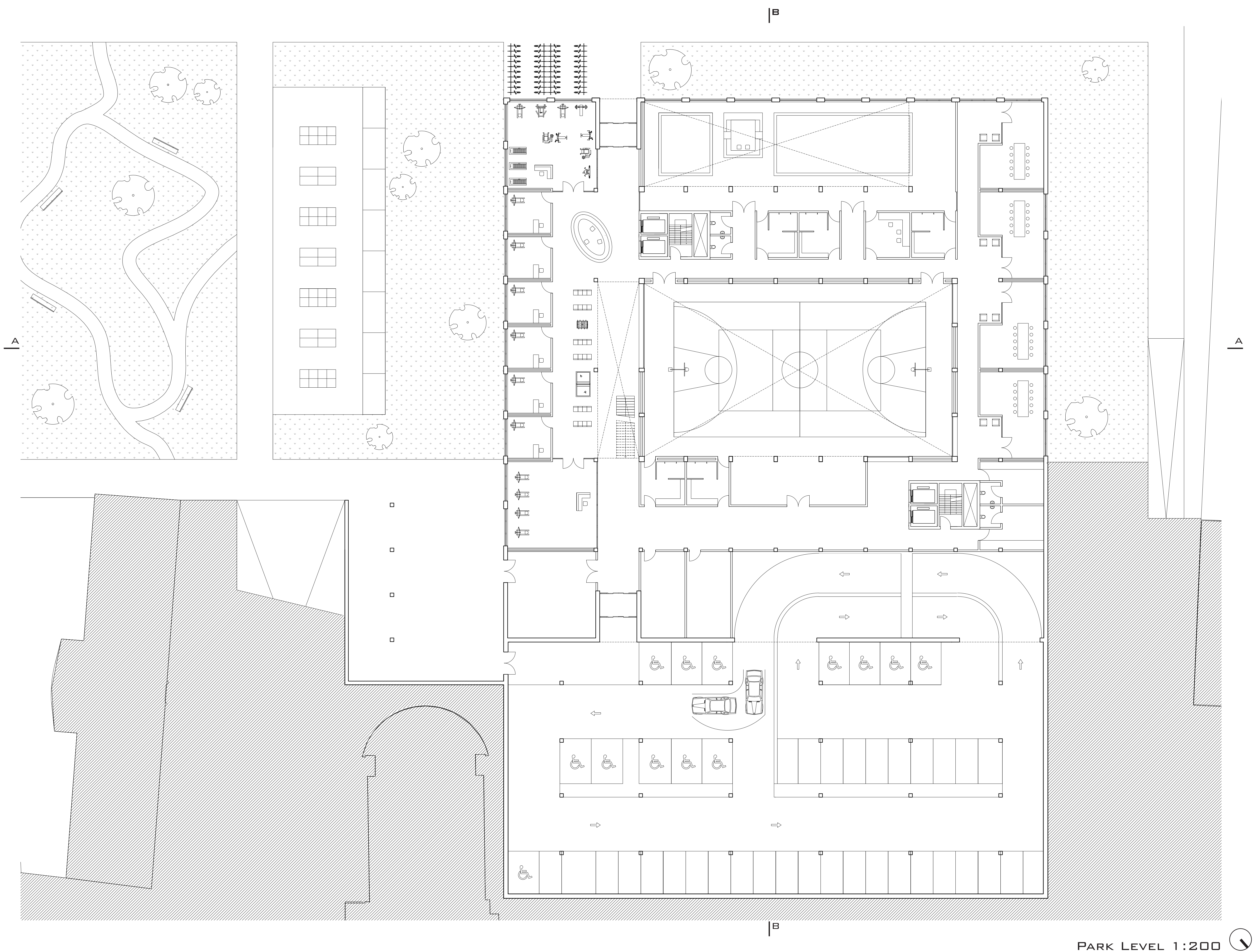
PARK LEVEL 1:200
