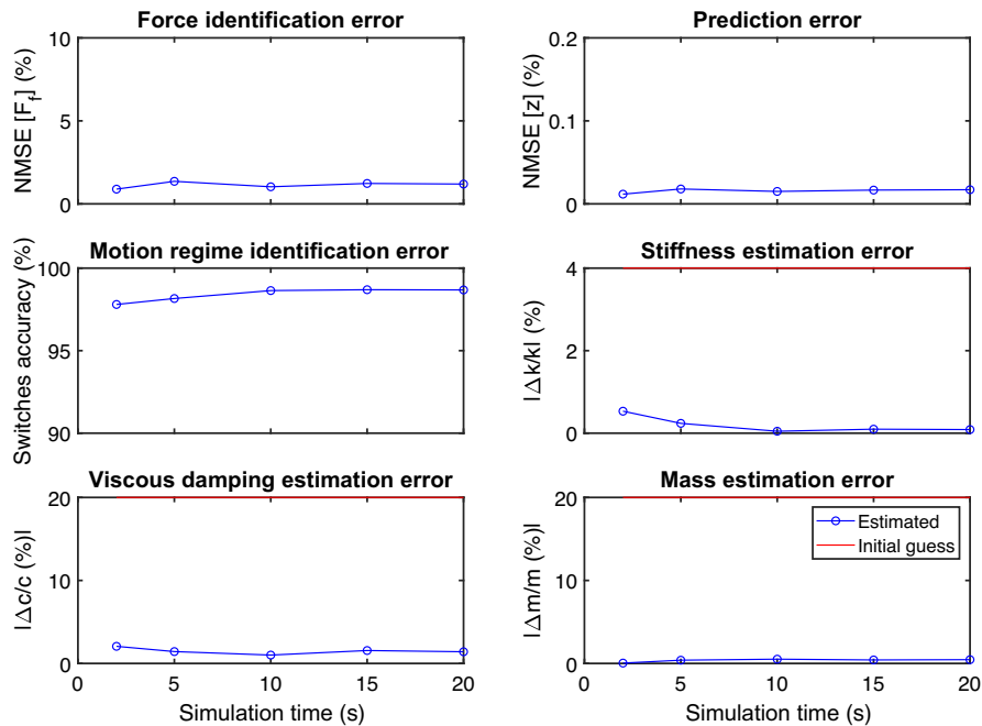
Figure 14. Nonlinear system identification performances of the switching GPLFM ( I=J=3 ) applied to the dry friction oscillator case-study for \text{SNR} = 80 dB, f_s = 500 Hz, and varying simulation times.
