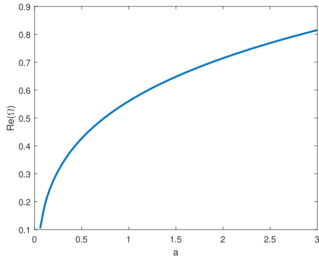
Fig. 3. This plot shows the real part of the oscillation frequency \Omega_0 as a function of the Winkler foundation coefficient a . The imaginary part of \Omega_0 is equal to zero. The parameter values are b_1 = 2 , and b_3 = 2 .
