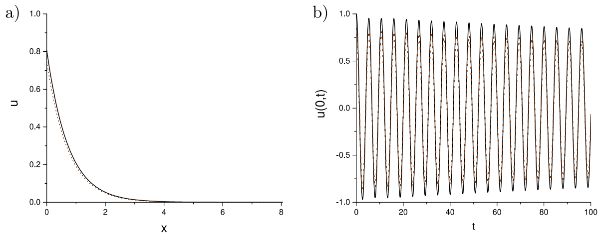
Fig. 11. This plot shows: (a) the shape, and (b) the time behavior of a localized mode for the case with damping. The solid line corresponds to the numerical results and the dotted line to the analytical results. The parameters are: b_3 = -2 , a = 6 , b_1 = 1 , \delta = 0.1 , b_2 = 0.01 .
