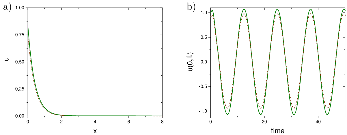
Fig. 9. This plot shows:(a) the shape, and (b) the time behavior at x = 0 of a localized mode for the case without damping. The solid line corresponds to the numerical results and the dotted line to the analytical results. The parameters are: b_3 = -2 , a = 6 , b_1 = 1 .
