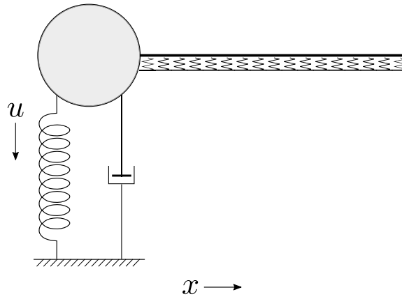
Fig. 1. String with an attached mass–spring–damper system at x = 0 .
