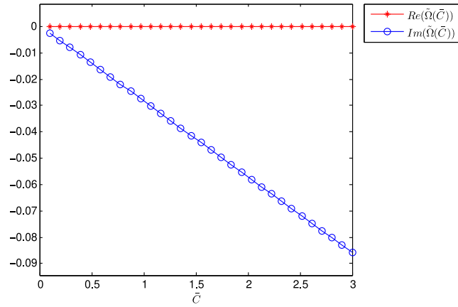
Fig. 7. This plot shows the results for the case with Kelvin–Voigt damping. The parameters are a = 0.3 , \bar{C} in the interval [0, 3] , and b_3 = 0.01 .
