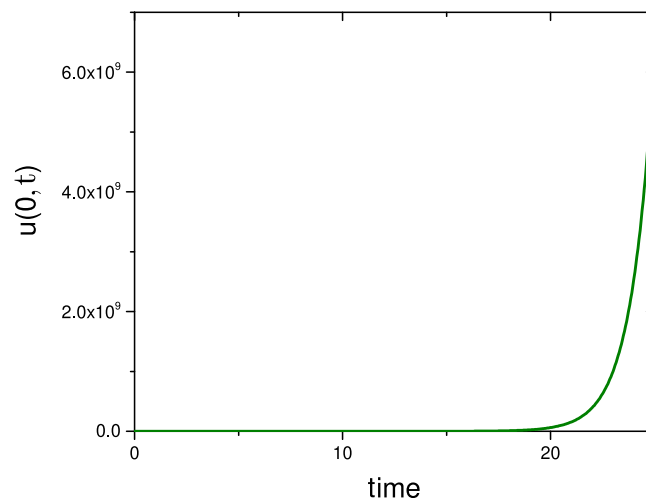
Fig. 10. This plot shows the increasing amplitude of a localized mode in time for the case without damping. The parameters are: b_3 = -2 , a = 0.3 , b_1 = 0.1 .
