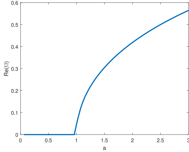
Fig. 4. This plot shows the real part of the oscillation frequency \Omega_0 as a function of the Winkler foundation coefficient a . The parameter values are b_1 = 2 , and b_3 = -1 .
