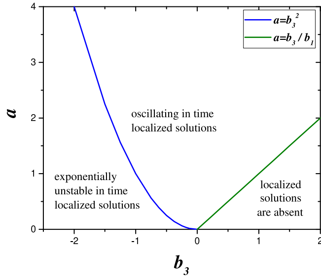
Fig. 2. This bifurcation diagram shows how the localized solutions depend on the two parameters a and b_3 , while b_1 = 1 is fixed (note that we can take b_1 = 1 by changing the variables x, t ; so, really we have two parameters). The whole parameter plane is divided into three regions, corresponding to the absence of solutions, stable oscillating solutions, and, in time exponentially increasing solutions.
