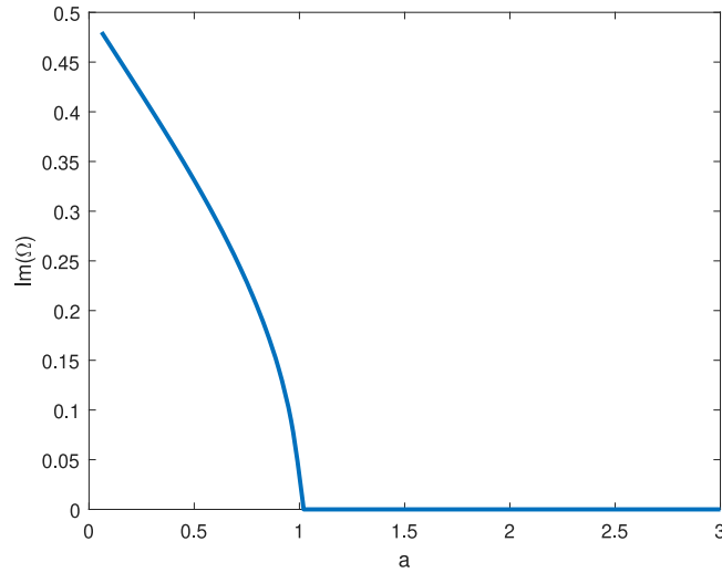
Fig. 5. This plot shows the imaginary part of the oscillation frequency \Omega_0 as a function of the Winkler foundation coefficient a . The parameter values are b_1 = 2 , and b_3 = -1 .
