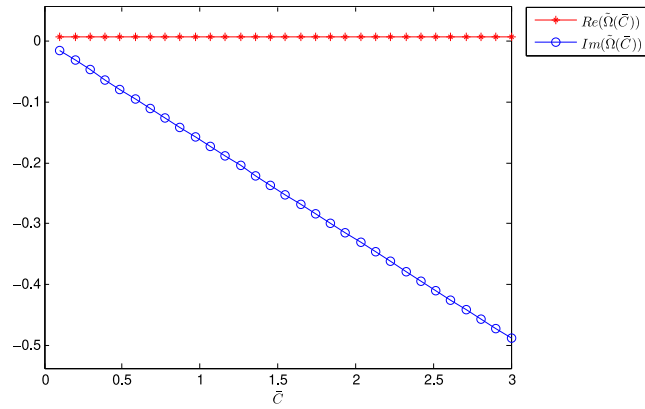
Fig. 8. This plot shows the results for the case with time hysteresis damping. The parameters are: a_1 = 0.3 , b_1 = 0.1 , b_3 = 0.01 .
