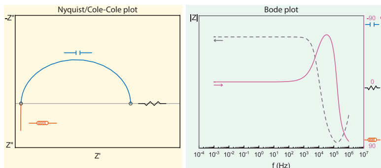
Figure 5.3: Examples of Nyquist/Cole-Cole and Bode plot representations of EIS data using an LR(RC) circuit. In a Nyquist plot, one can quickly identify if C, R, or L components are needed in the equivalent circuit model based on which quadrant the data is in. In a Bode plot, this is done based on the trends of \phi (solid pink line) and |Z| (dashed grey line) with frequency. While the L results in a +90^\circ value for \phi , C results in the opposite, -90^\circ . At lower frequencies, when the signal is dominated by R, \phi is 0.
