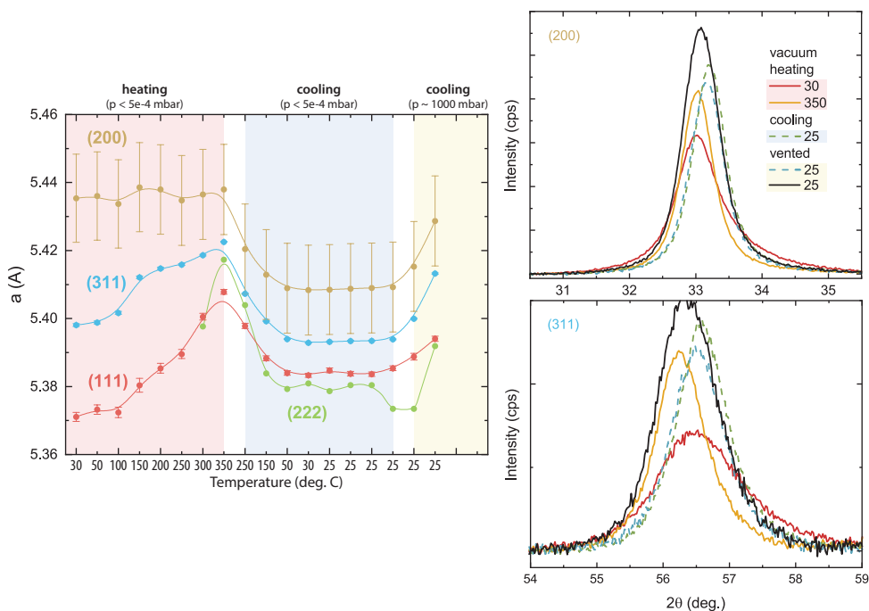
Figure 6.3: (left) In situ XRD was performed for the sample (on fused silica) described in Fig. 6.2. First, the sample was heated under vacuum ( <5 \times 10^{-4} mbar) from 30 to 350°C. Then it was cooled to 25°C under the same vacuum and measured four times at 25°C. Last, the cell was vented and the sample was measured twice in air at 25°C. This figure shows the lattice constant “ a ” derived from each visible reflection in the XRD patterns. (right) Changes in the (200) (top) and (311) (bottom) reflections from XRD at different points in the programme. Red and orange lines are during heating at 30 and 350°C, respectively. After cooling, the fourth measurement at 25°C is shown as a green dashed line. Then the cell was vented and the sample was measured twice, showed as a blue dashed line and a black solid line. The peak positions clearly change, indicated also by the changes in “ a ” in the left graph.
