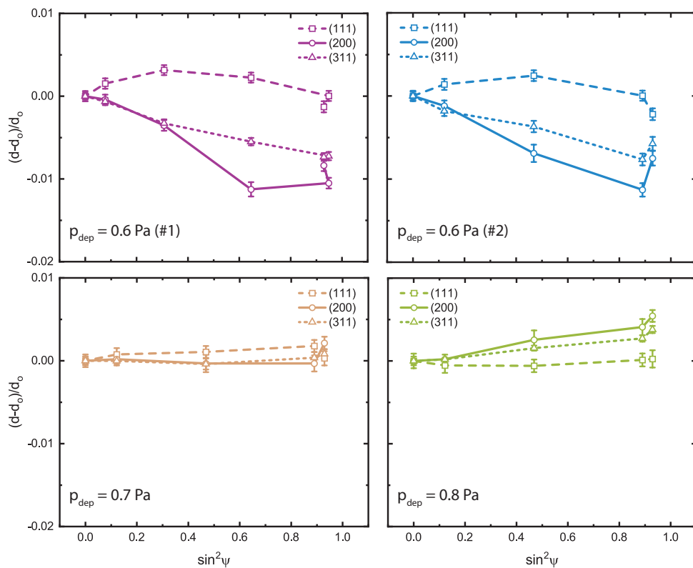
Figure 3.H.3: Analysis of macrostrain for 4 NdH 3-2x O x films. Dashed lines are derived from the (111) peak positions, solid lines from (200), and dotted lines from (311). The slopes of these lines are related to the macrostrain.
