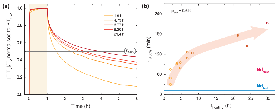
Figure 3.5: (a) Relative photochromic contrast normalised to the maximum contrast for annealed NdH_{3-2x}O_x films made at p_{dep} = 0.6 \text{ Pa} . Normalisation was done to better visualise the bleaching speeds of films made at progressively longer t_{heating} . (b) Bleaching time constants ( \tau_{B,50\%} ) for several NdH_{3-2x}O_x films made at p_{dep} = 0.6 \text{ Pa} with controlled heating times. Pink and blue lines indicate the “slow” and “fast” samples discussed in Fig. 3.4.
