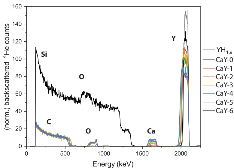
Figure 4.C.1: Rutherford backscattering (RBS) spectra for a series of samples with increasing Ca-content. All samples containing Ca ( \text{CaY-1} to \text{CaY-6} ) were measured on glassy carbon substrates, while the undoped Y-oxyhydride ( \text{CaY-0} ) was on a substrate of \text{SiO}_2/\text{Si} which not only obscured the O peak, but has a different background offset due to the underlying silicon.
