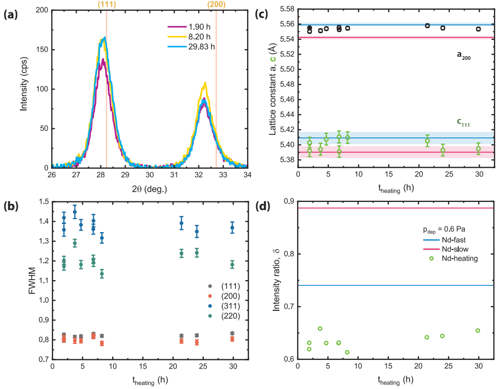
Figure 3.J.1: (a) GI-XRD patterns for three \text{NdH}_{3-2x}\text{O}_x films ( p_{\text{dep}} = 0.6 Pa) heated for various times at 87^\circ\text{C} in the ALD chamber ( p \sim 2 \mu\text{bar} ). Only the (111) and (200) reflections are shown. Red reference lines are for the fcc (cubic) \text{NdH}_{1.9+\delta} pattern from ICDD-PDF database # 00-89-4199. Several quantities can be derived from those XRD patterns such as (b) the full-width half-maxima of all the visible reflections, (c) the lattice constants a_{200} and c_{111} , and (d) the intensity ratio ( \delta = \frac{I_{111}}{I_{111}+I_{200}} ). None of these quantities change significantly during \sim 30 h of heating at 87^\circ\text{C} . The shaded pink and blue areas in (c) indicate the error associated with the lattice constant for slow and fast bleaching \text{NdH}_{3-2x}\text{O}_x films (0.6 Pa), respectively. As well, in (d), the pink and blue lines show the intensity ratios for the slow and fast bleaching samples, respectively.
