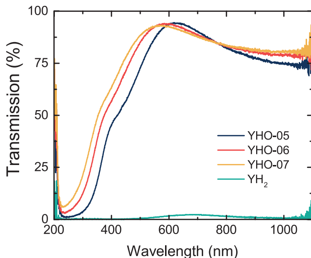
Figure 2.A.1: The final optical transmission spectra (day 10) for all of the thin-films studied here (day 10). YH 2 shows a transmission window, implying that its composition is sub-stoichiometric YH 1.9 . The YH 3-2x O x thin-films show high optical transparency until their band edge, which shifts to higher energy values as the p_{dep} increases and the O:H ratio increases. The transmission of the YH 3-2x O x thin-films is not flat due to thin-film interference which results in an oscillating pattern. Because this pattern is nearly identical for all the samples, they can be assumed to be of nearly identical thickness ( \sim 150 nm).
