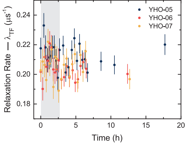
Figure 2.D.1: The three YH_{3-2x}O_x thin-films were in situ illuminated under TF conditions where the fitting parameters are the diamagnetic asymmetry ( A_{dia,TF} ) and the Lorentzian relaxation rate ( \lambda_{TF} ). The A_{dia,TF} is shown in the main text, increasing reversibly upon illumination with a UV LED. On the other hand, \lambda_{TF} does not change during illumination. This parameter is related to E_{A,\lambda} which was calculated to be \sim 15 meV under “dark” conditions. This is already a very low activation energy, only slightly higher than thermal energy at 50 K ( \sim 4 meV). Therefore, if the E_{A,\lambda} changed under illumination, the difference may be very small and not resolved well in our data. However, if we consider E_{A,\lambda} to be unaffected by illumination, that would mean polaron formation is neither enhanced nor impeded during photochromism, and local lattice changes are more responsible for the colour changing effect.
