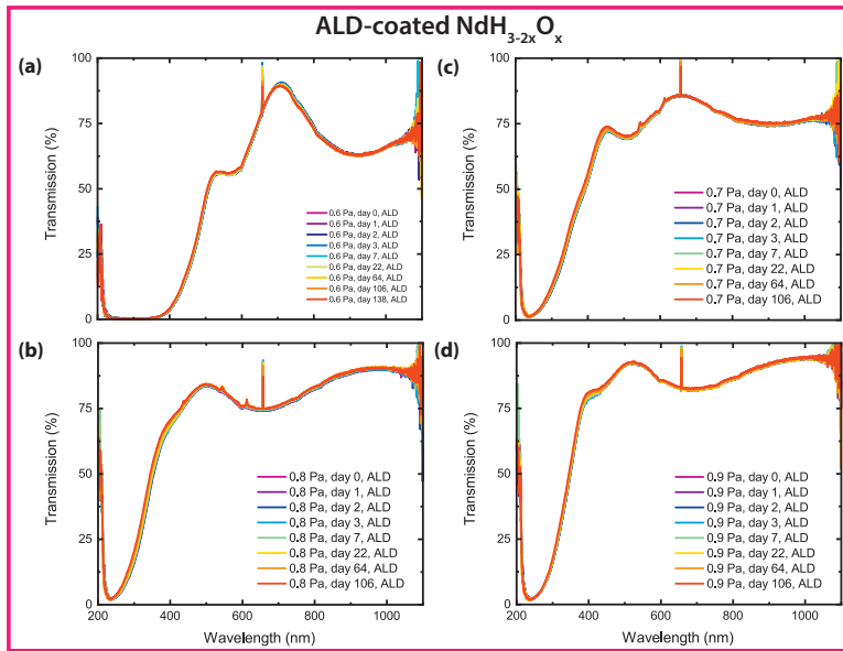
Figure 3.A.2: Optical transmission spectra for some Nd-oxyhydride thin films produced at different deposition pressures ( p_{dep} = 0.6 - 0.9 Pa) with a protective coating of \text{Al}_2\text{O}_3 deposited onto the films by ALD. Unlike the uncoated films, these Nd-oxyhydrides are stable in ambient air for at least 138 days since the absorption edge shows little-to-no shift over time. This implies that no significant oxidation occurs for these films, substantially extending their lifetime.
