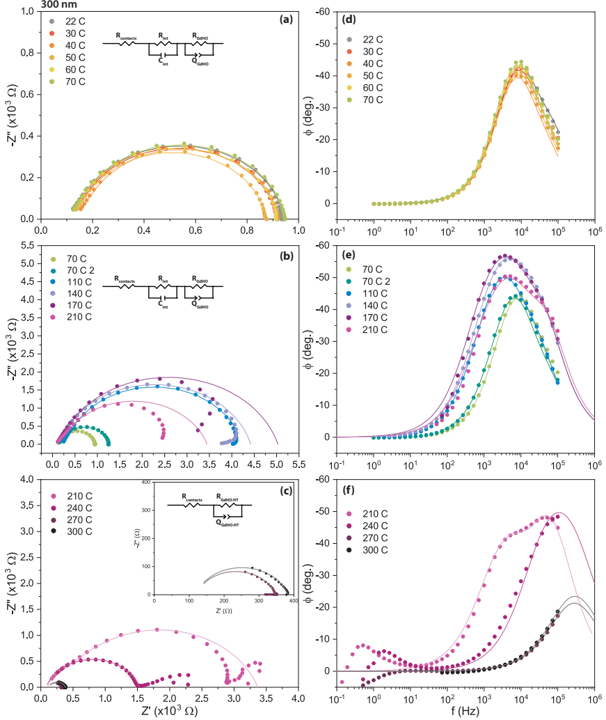
Figure 5.C.1: Nyquist plots for 300 nm Gd-oxyhydride (0.7 Pa) are shown for different temperature ranges: (a) 22–70°C, (b) 70–210°C, and (c) 210–300°C. The equivalent circuits used to fit the data are shown next to the legends. (d), (e), and (f) show the corresponding \phi angle change with frequency (half of the Bode plot). All the lines in these plots are the equivalent circuit fit. The same two components of the equivalent circuit model are used here as for the 25 nm thin film. As well, unreproducible behaviour is shown in the second temperature regime. At high temperatures, only the R(RQ) related to the contacts and the Gd-oxyhydride are visible. In the legend, when a “2” follows the temperature label, it indicates that two measurements were performed at this temperature this is the second one.
