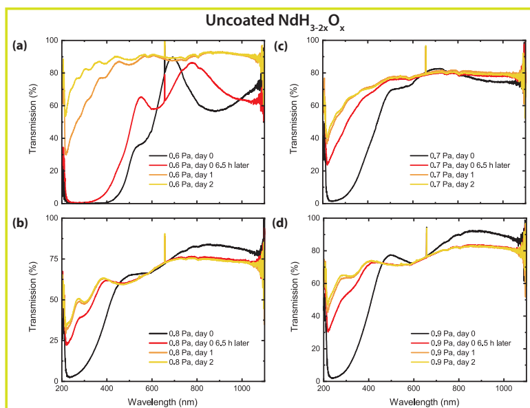
Figure 3.A.1: Optical transmission spectra for some Nd-oxyhydride thin films produced at different deposition pressures ( p_{\text{dep}} = 0.6 - 0.9 Pa) without a protective coating. Day 0 is the day of deposition and onset of air oxidation. The low transmission at short wavelengths is related to the band gap of the material. This absorption edge quickly shifts to the left (larger band gap), resulting in a completely oxidised (no \text{H}^- ) compound by day 2 for all deposition pressures.
