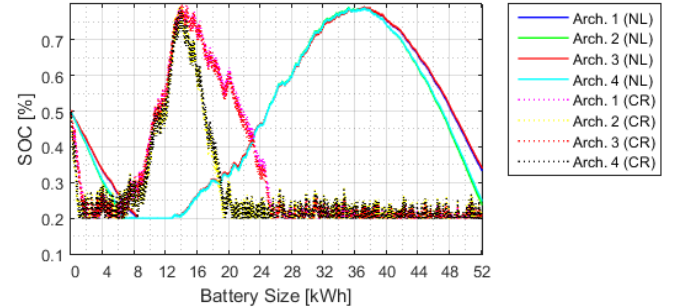
Figure 5. SOC 100% self-consumption for The Netherlands and Costa Rica
