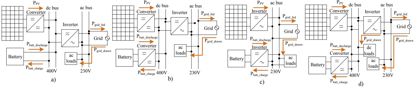
Figure 1. a) In line (1 st ), b) DC coupled architecture (2 nd ), c) AC coupled (3 rd ), and d) DC/AC coupled (4 th )
