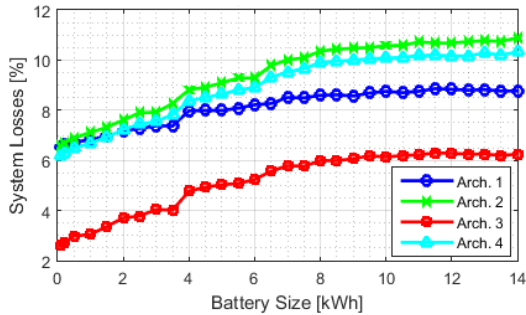
Figure 14. System Losses (the Netherlands)
