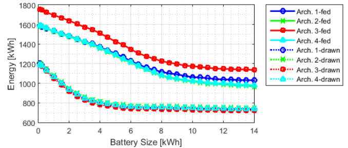
Figure 10. Energy exchange with the grid at base time (the Netherlands)
