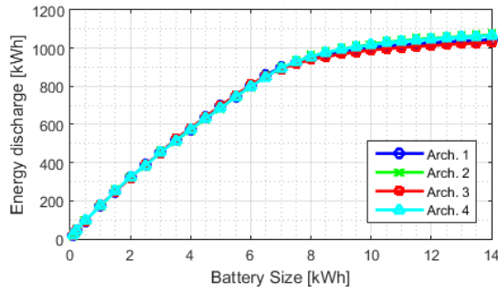
Figure 17. Energy discharge from battery
