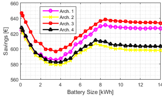
Figure 9. Savings (Costa Rica)
