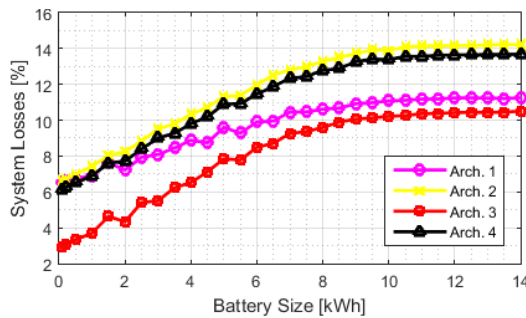
Figure 15. System Losses (Costa Rica)
