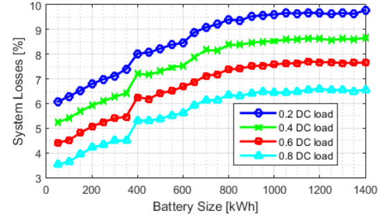
Figure 20. System losses
