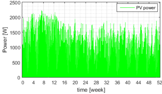
Figure 4. PV Generation (Costa Rica, 2014)
