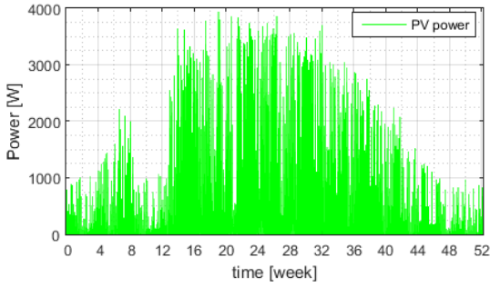
Figure 3. PV Generation (The Netherlands, 2014)
