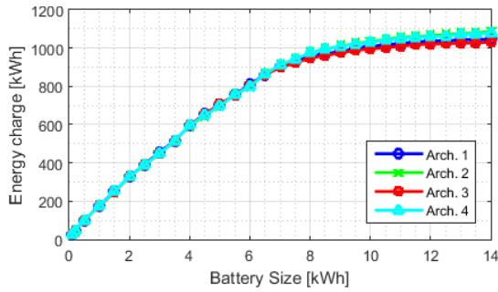
Figure 16. Energy charge to battery
