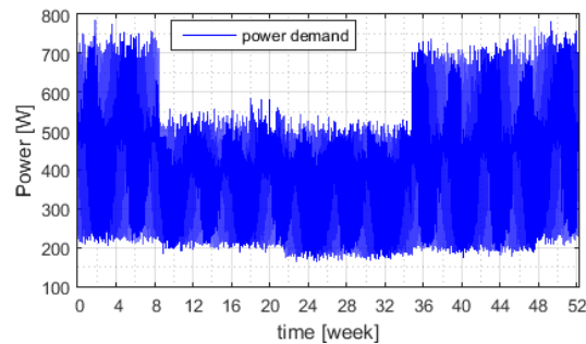
Figure 2. Load Profile
