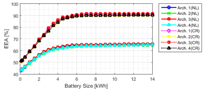
Figure 6. EEA Base the Netherlands and Costa Rica
