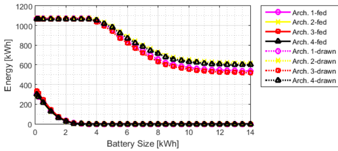
Figure 13. Energy exchange with the grid at off-peak time (Costa Rica)
