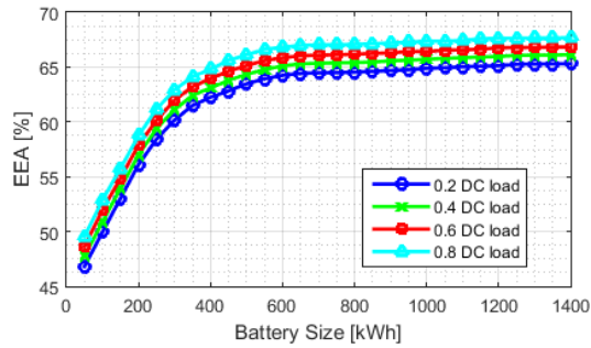
Figure 18. EEA base
