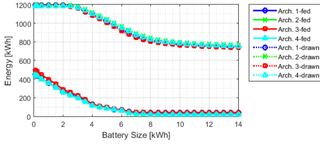
Figure 11. Energy exchange with the grid at off-peak time (the Netherlands)
