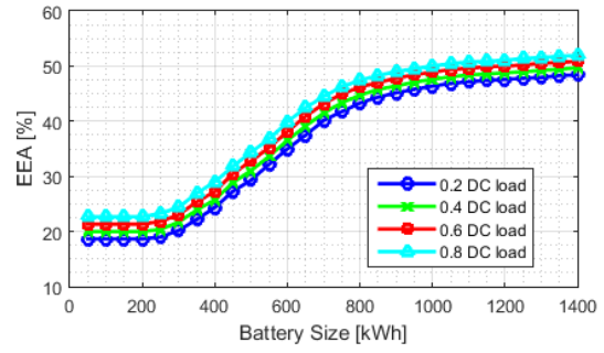
Figure 19. EEA off-peak
