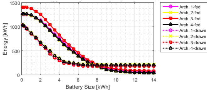
Figure 12. Energy exchange with the grid at base time (Costa Rica)
