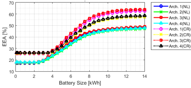
Figure 7. EEA off-peak the Netherlands and Costa Rica
