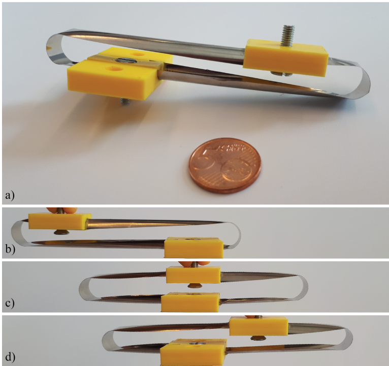
Figure 6.9.: A prototype of the concept was fabricated from a 50\mu\text{m} . thick stainless-steel sheet, with a diameter of 10 mm. Figures b, c and d show the prototype in three stances within the range of motion.
