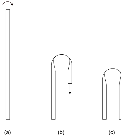
Figure 5.5.: FEM steps: a) end-point rotation of \pi , b) vertically displace end-points to same height, c) final deformed geometry
