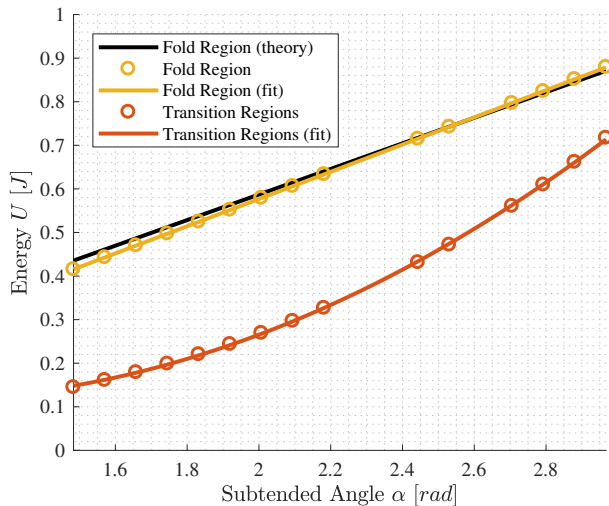
Figure 5.10.: Energy per region for different subtended angles
