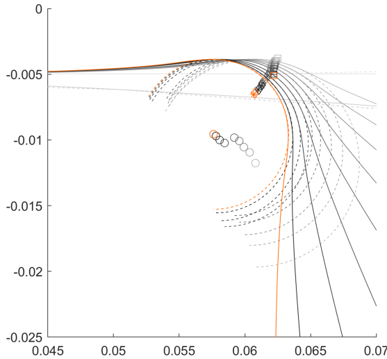
Figure 4.18.: Shape of tape spring during bending, seen at the plane x = 0 , the shape with the largest angle is shown in orange, the fitted folds are denoted by the dashed lines, the fitted fold centres are circles, the instant centres of rotation by squares, the incremental instant centres of rotation by diamonds and the location of the degree of freedom eigentwist by stars.
