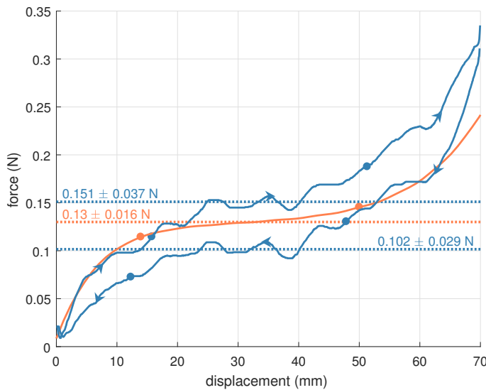
Figure 6.11.: The force-displacement graph shows the measured force in the forward and backward motion (blue) together with the numerical simulation results (orange) of a geometry with matching dimensions. The average values of the fairly constant force regions are denoted by the dotted lines. The markers denote the outermost positions of the range of motion. The deviation of these points to average is listed. This is done for the simulation, the forward and backward motions separately.
