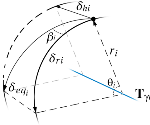
Figure 2.3.: Equivalent translation geometry
