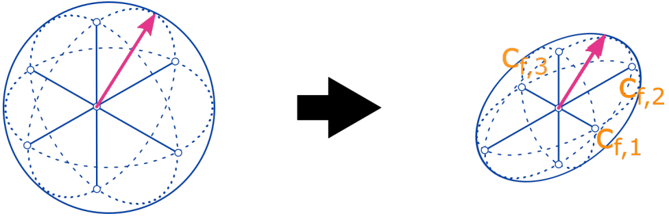
Figure 4.1.: Mapping of a linear combination of eigenwrenches to the corresponding linear combination of the induced twists; this linear combination is scaled by the eigencompliances. Visually a unit sphere is scaled to an ellipsoid.
