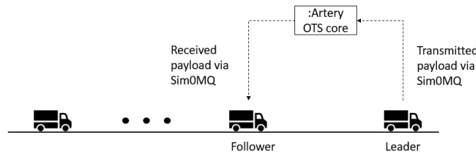
Figure 1: OTS-Artery architecture showing information exchange between a leader-follower pair. The leader transmits the payload (sender GTU id, receiver GTU id, signal strength, time stamp, speed, and acceleration) to the Artery OTS core. The follower then calls the core upon message reception and receives the payload if the follower id matches the receiver GTU id in the payload. A new payload is transmitted every 100 ms. More information about OTS-Artery is available at: https://github.com/salilrsharma/OTS-Artery .
