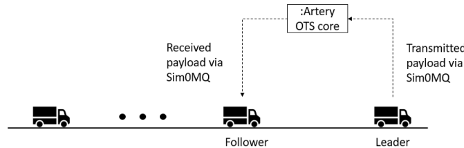
Figure 1: OTS-Artery architecture showing information exchange between a leader-follower pair (the leader transmits the payload (sender GTU id, receiver GTU id, signal strength, time stamp, speed, and acceleration) to the Artery OTS core. The follower then calls the core upon message reception and receives the payload if the follower id matches the receiver GTU id in the payload. A new payload is transmitted every 100 ms. More information about OTS-Artery is available at: https://github.com/salilrsharma/OTS-Artery .
