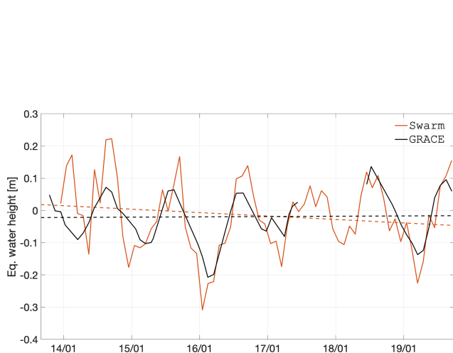
Figure E5. Time series of EWH for the Orinoco basin (latitude −3 to 12°, longitude −72 to −59°).
