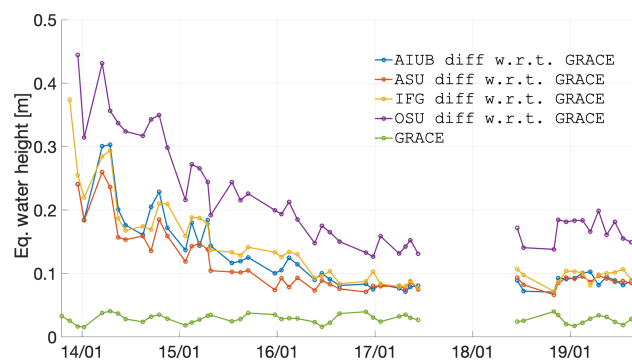
Figure 6. Time dependence between December 2013 and September 2019 of the epoch-wise cumulative degree amplitude (or global spatial rms) of the individual Swarm solutions, CSR RL06 GRACE, and their difference, considering 750 km smoothing.
