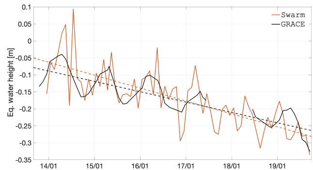
Figure E1. Time series of EWH for Alaska (latitude 56^{\circ} to 65^{\circ} , longitude -151^{\circ} to -129^{\circ} ).
