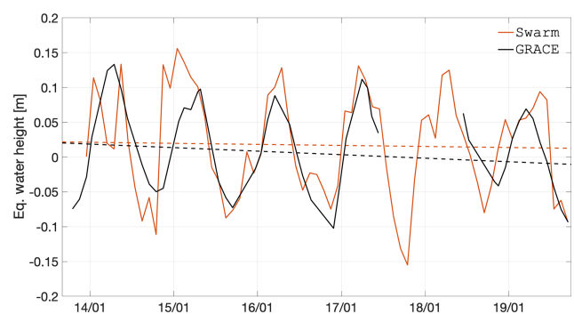
Figure E2. Time series of EWH for the Congo and Zambezi basins (latitude -23^{\circ} to -3^{\circ} , longitude 14^{\circ} to 38^{\circ} ).
