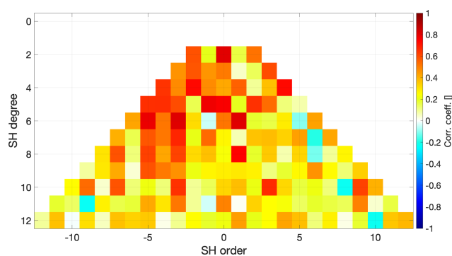
Figure 18. Per-coefficient correlation coefficient between the GRACE climatological model and Swarm.
