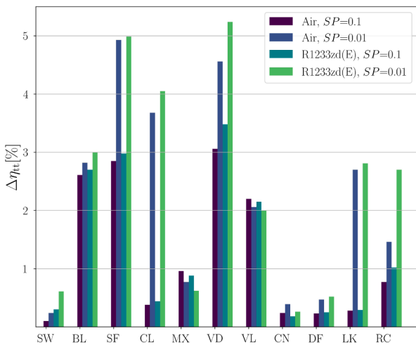
Fig. 11. Loss breakdown for compressor stages operating with air and refrigerant R1233zd(E), featuring \Phi_{t1} = 0.13 , \psi_{is} = 0.8 , \beta_{tt} = 3.5 , SP = 0.1 - 0.01 . The abbreviations displayed on the abscissa refer to the subscripts used to identify the loss components.
