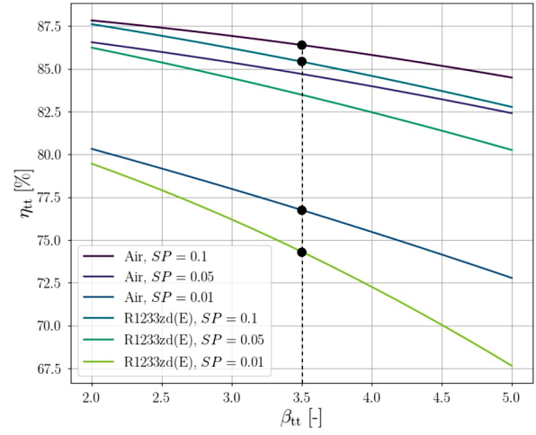
Fig. 10. Locus of optimal efficiency for compressors characterized by different size parameter. All the computations are performed at \psi_{is} = 0.8 , k = 0.9 , and at P_{t1} , T_{t1} specified in Tab. 1. The black dots correspond to the stage designs chosen for the loss breakdown analysis.
