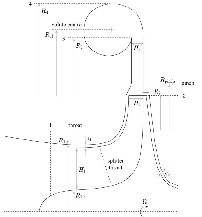
Fig. 2. Meridional view of a centrifugal compressor stage featuring splitter blades, pinched vaneless diffuser, overhung volute, and no inlet guide vanes.
