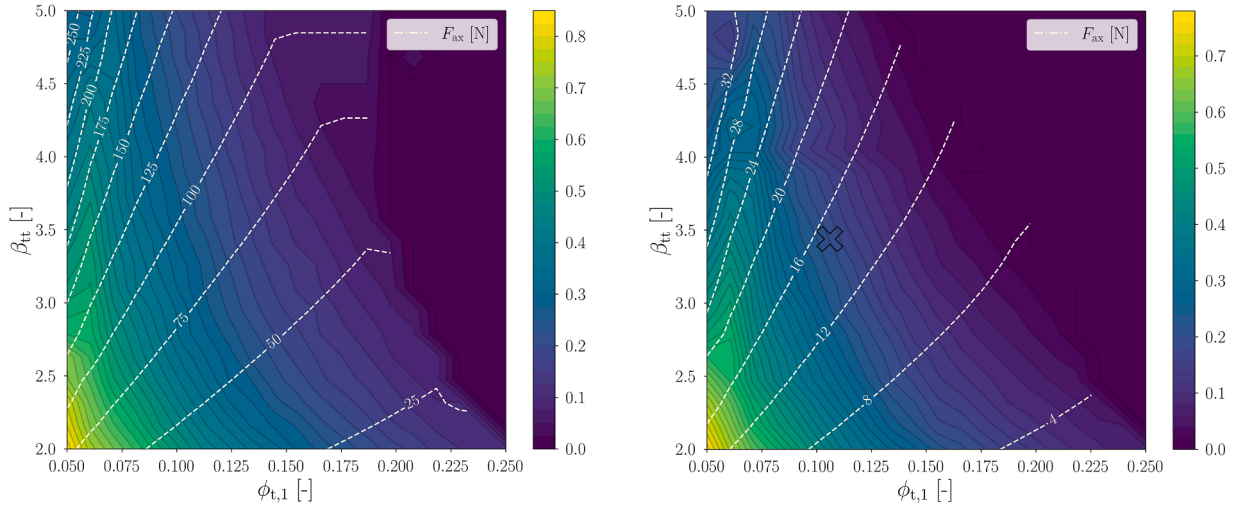
Fig. 7. Design maps of OR, and F_{ax} , computed for air and refrigerant R1233zd(E) at \psi_{is} = 0.8 , SP = 0.01 , k = 0.9 , and at P_{t1} , T_{t1} specified in Tab. 1. The cross indicates the design point resulting from the optimization study described in Section 5.
