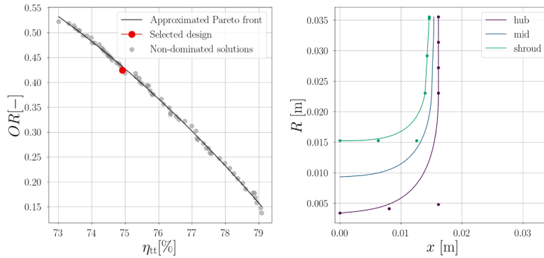
Fig. 12. Optimal design of the first compressor stage for the IRIS test rig. From left to right: Pareto front obtained with the multi-objective optimization framework, meridional flow path of the selected design, 3D impeller geometry and computational grid. The hub and shroud curves are defined as third order Bezier curves, whose control points are displayed in the central image.
