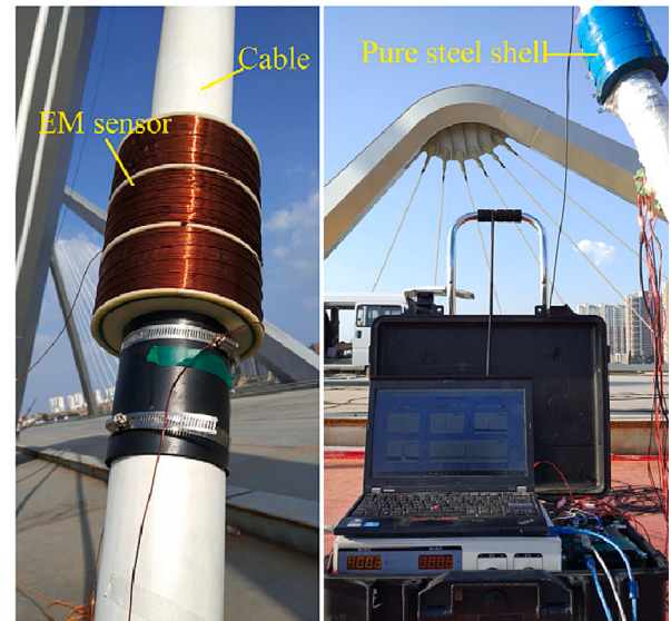
Fig. 20. The field test pictures of magnetoelastic sensor (taken from [60]).
