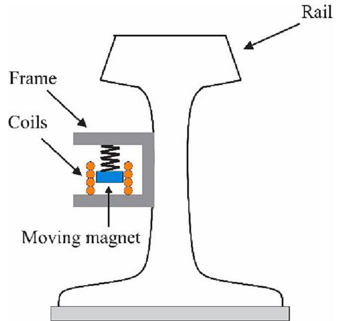
Fig. 37. The physical model of the energy harvester.
