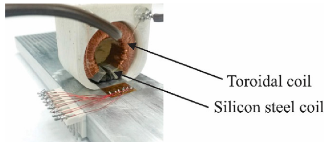
Fig. 27. The MCM sensor (taken from [88]).
