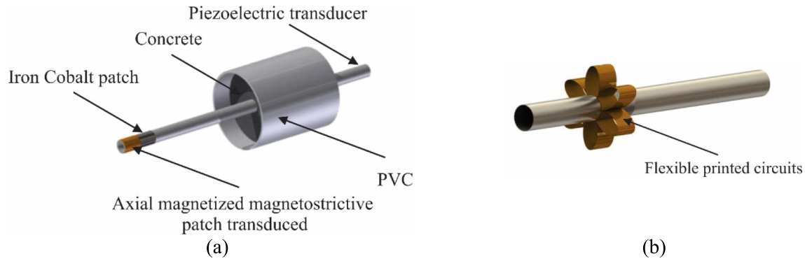
Fig. 28. Magnetostrictive patch transducers: (a) axial magnetized (b) segmented axially magnetized (taken from [89;90]).
