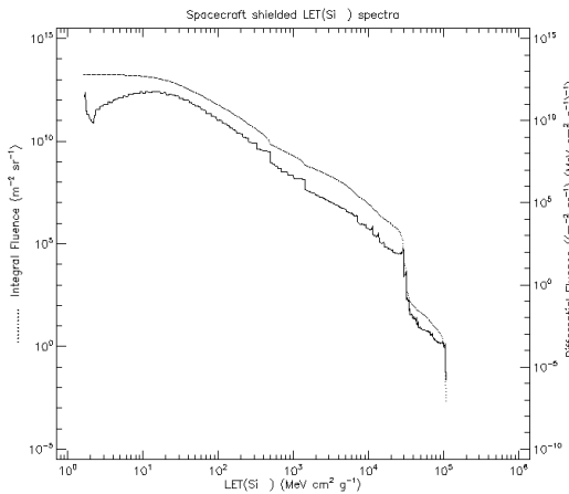
Fig. 7: The LET spectrum.
