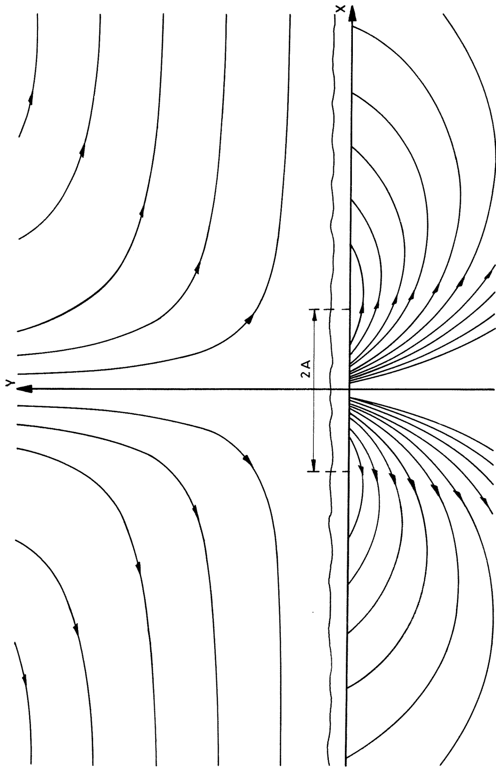
FIG. 18a STREAMLINE PATTERN OF AN EROSION FLOW ABOVE AND BELOW THE SURFACE OF A POROUS BED
