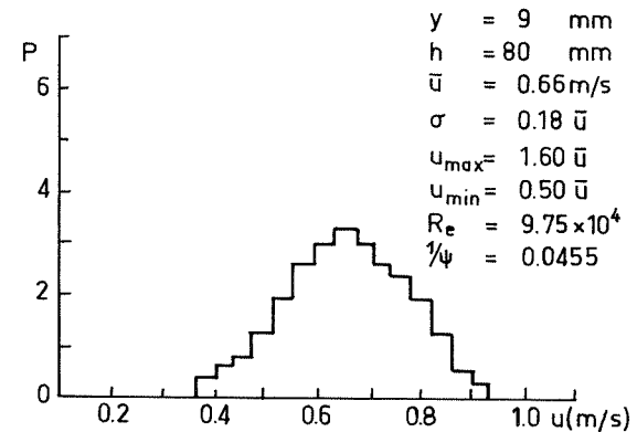
6c. MAGNETITE ( D_s=1.8\text{mm} ) Total sample size 246
