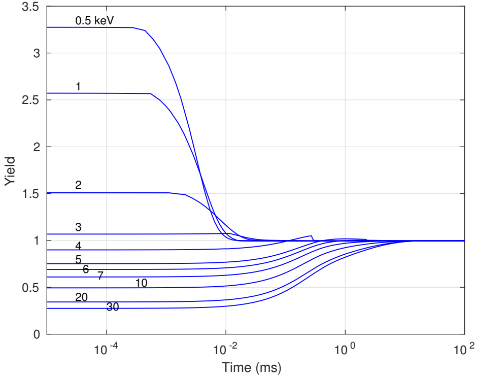
Figure 4.14: Time evolution of the yield from an amorphous alumina sample versus PE energy for a defocused beam with current density of 10^{-5} A/cm 2 . The distance between \Sigma_1 and \Sigma_2 is 1 mm.
