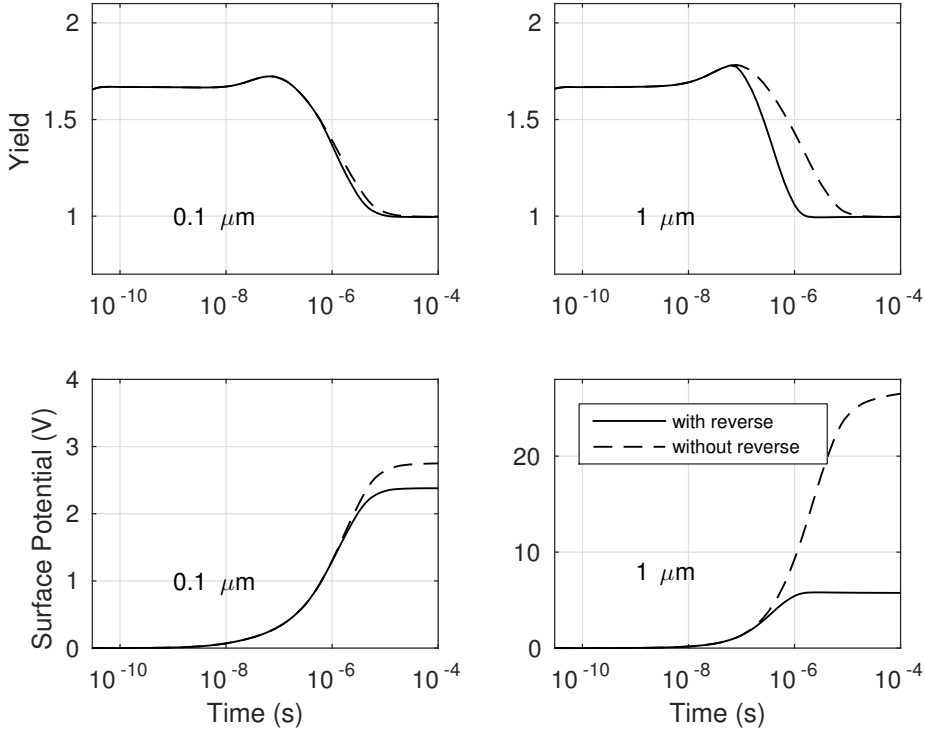
Figure 5.6: Yield and surface potential with and without the reverse current term \propto \frac{\partial V}{\partial \nu} for close (left) and remote (right) \Sigma_1 .
