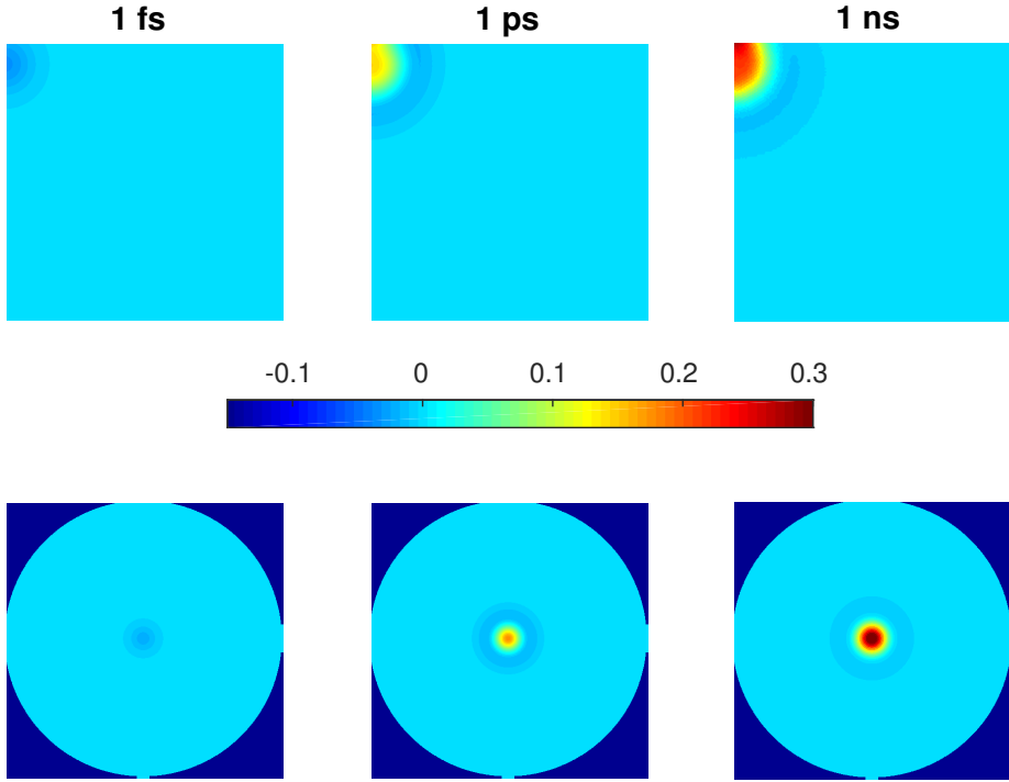
Figure 4.10: Evolution of the total charge (N_T/2 + p - n - n_T)q ( C cm^{-3} ) in sapphire ( Al_2O_3 ) after the impact of a single primary electron with the energy E_0 = 1 keV. Top row: vertical cross-section, side length is 100 nm; bottom row: top-view of the sample-vacuum interface, diameter is 200 nm.
