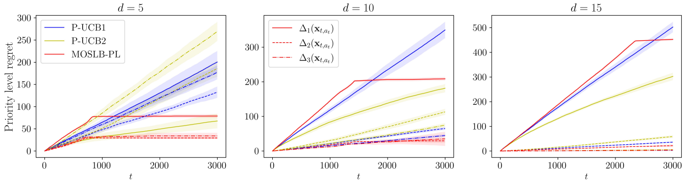
Figure 5: Pareto level regret of the compared methods for MPL-PL: \Delta_1(\mathbf{x}_{t,a_t}) + \Delta_2(\mathbf{x}_{t,a_t})\mathbb{I}^{-1} + \Delta_3(\mathbf{x}_{t,a_t})\mathbb{I}^{-2} .
