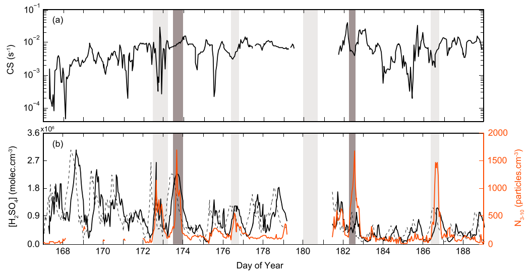
Figure 3. (a) Evolution of the hourly averaged condensation sink (CS) value. (b) The \text{H}_2\text{SO}_4 proxy concentration (black lines) and N_{3-10} concentration (red line) in the D_p = 3-10 nm range. Solid and dashed black lines correspond to hourly \text{H}_2\text{SO}_4 concentrations when shifted and not shifted by 6 h, respectively. Data for the \text{H}_2\text{SO}_4 proxy concentration calculations were provided by the Alfred Wegener Institute [Maturilli et al., 2012].
