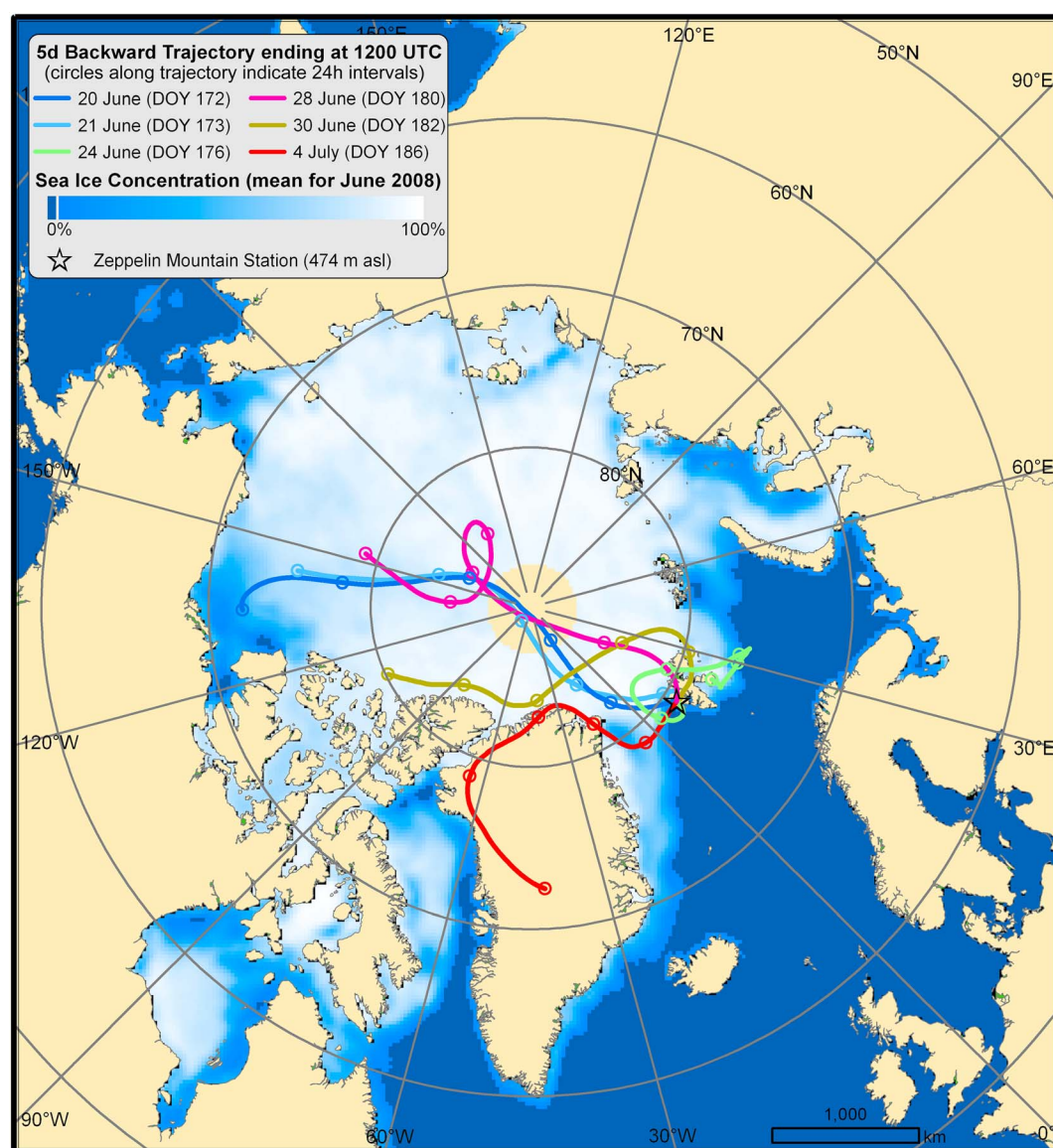
Figure 2. Air mass back-trajectories (5 days) arriving at the Zeppelin atmospheric research station (78.90°N, 11.88°E; 474 m asl) near Ny-Ålesund, Svalbard at 12:00 UTC on days when NPF events were observed. The trajectories were determined by the NOAA HYSPLIT model [Draxler and Rolph, 2015]. The sea ice concentration corresponds to the average June 2008 coverage [NSIDC, 2014].
