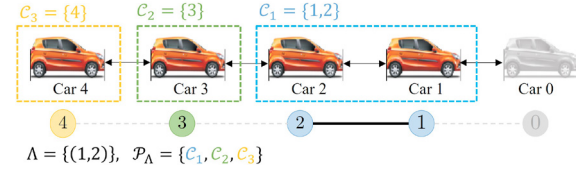
Fig. 1. Topology and resulting coalitions in a platoon with 4 vehicles following a leader.
