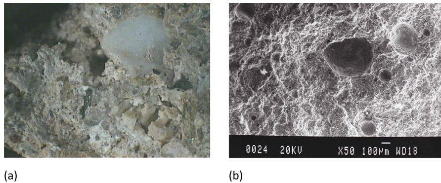
Fig. 23 (a) Macro-scale porosity in lime-based mortar and (b) micro-scale under SEM
