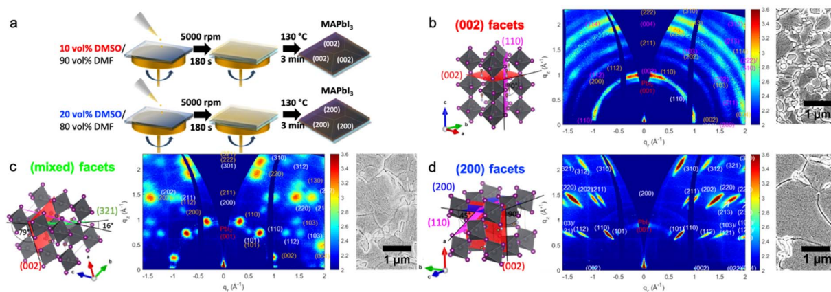
Fig. 1 (a) Schematic illustration of the synthesis process with varying DMSO concentrations to achieve either (002) or (200) facet alignment in a precursor solution containing 1.875 mmol mL -1 PbAc 2 and 5.625 mmol mL -1 MAI. (b–d) Schematic illustrations (left) of the different crystal facets parallel to the substrate, representing the main orientation deduced from 2D GIWAXS data (middle) and the SEM images of the respective films (right). (b) Perovskite film with the (002) facet parallel to the substrate; (c) perovskite film with (200) and (321) facets parallel to the substrate; (d) perovskite film with the (200) facet parallel to the substrate.
