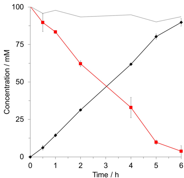
Figure 4. Scale up of the oxidative decarboxylation of sodium glutamate (♦) to CPA (◆), (---) mole balance. [sodium glutamate] = 100 mM, [NaBr] = 0.5 mM, [CVCPO] = 55 nM, \text{H}_2\text{O}_2 -dosage: 39 \text{ mM h}^{-1} from a 1 M stock solution, 20 mM sodium citrate buffer (pH 5.6), room temperature ( 22^\circ\text{C} ). The error bars represent the range of duplicate experiments.
