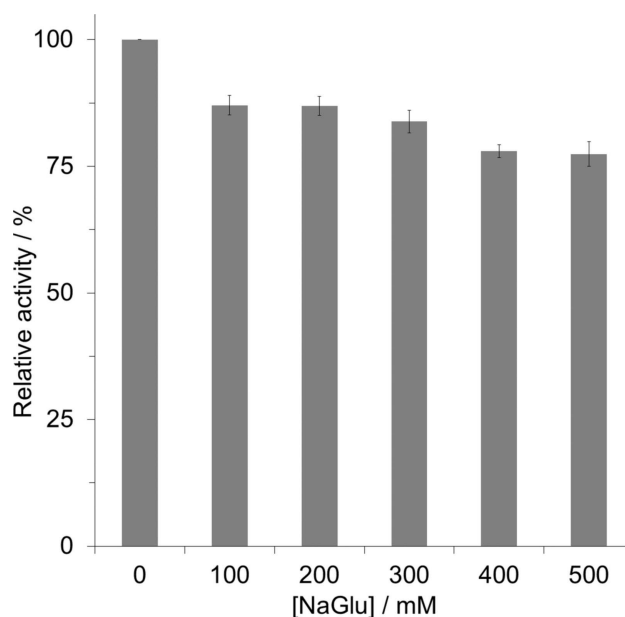
Figure 5. Influence of sodium glutamate (NaGlu) on the activity of CVCPO. Assay conditions: [MCD] = 50 \mu\text{M} , [\text{H}_2\text{O}_2] = 1 \text{ mM} , [NaBr] = 0.5 \text{ mM} , [\text{Na}_3\text{VO}_4] = 100 \mu\text{M} , 50 mM sodium citrate buffer (pH 5), T = 25^\circ\text{C} , 290 nm. The reaction was started with addition of 0.8 \text{ nM} CVCPO that was pre-incubated for 5 min with different amounts of NaGlu. The error bars represent the standard deviation of triplicate experiments.
