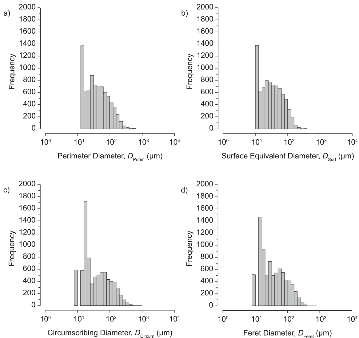
Fig. 4. Floc size distribution based on 3D data using equivalent floc diameter; (a) the D_{\text{Perim}} , (b) the D_{\text{Surf}} , (c) the D_{\text{Circum}} and (d) the D_{\text{Feret}} .
