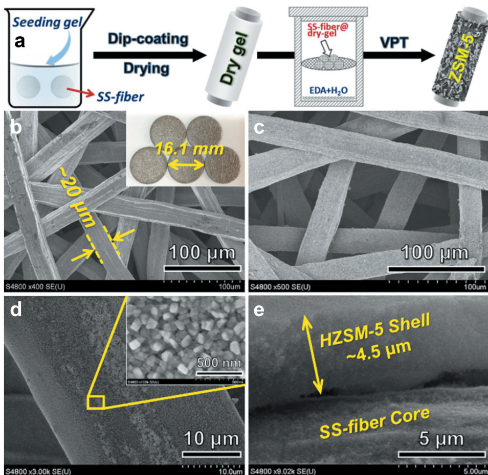
Figure 8. (A) Schematic illustration for the top-down fabrication strategy of coupling dip-coating with seed-assisted VPT method. (B) Photograph and SEM images of the SS-fiber substrate. (C-E) SEM images of the representative HZSM-5/SS-fiber catalyst with 23.0 wt% HZSM-5, showing the monolithic and surface structures (Reprinted with permission from ref. [83] Copyright 2018 Elsevier).
