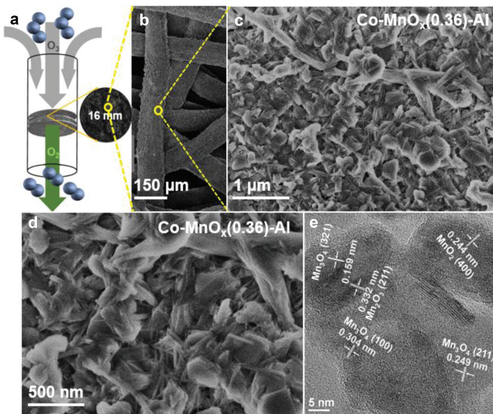
Figure 26. Geometry, morphology and structure features of the representative Co-MnO x /ns-Al 2 O 3 /Al-fiber catalyst from nano- to macro-scale: (a) optical photograph, (b-d) SEM and (e) TEM images (Reprinted with permission from ref. [227] Copyright 2015 Wiley and Sons).
