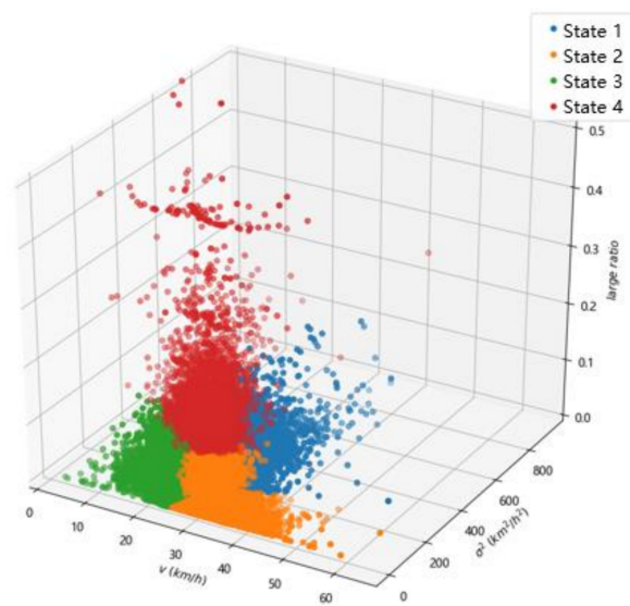
Figure 6. Clustering results of k = 4
