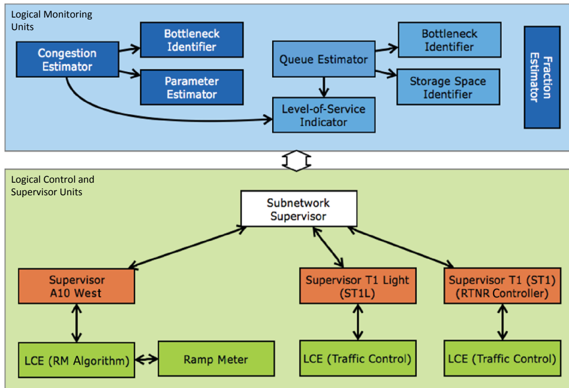
FIGURE 2 Functional architecture of APT control approach, indicator of logical monitoring units and logical control units (LCE = logical control unit (translated from Dutch); RM = ramp metering; RTNR = real-time network regulator; ST1L = urban arterial supervisor (translated from Dutch abbreviation).
