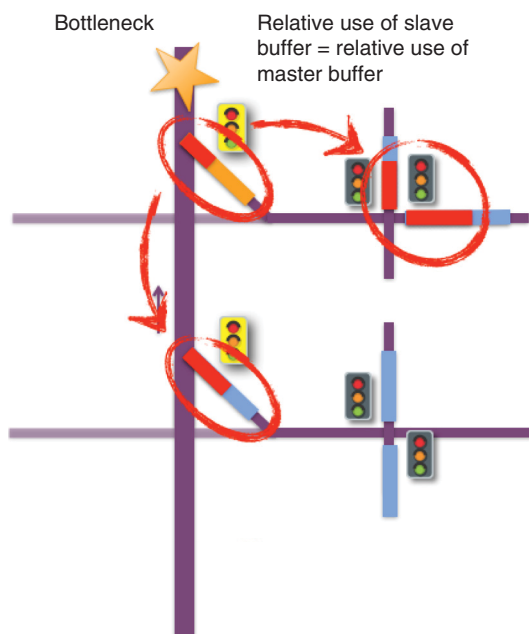
FIGURE 3 Illustration of control approach for freeway bottleneck controlled with on-ramp and supported by slave ramp meter and slave intersection controller.
