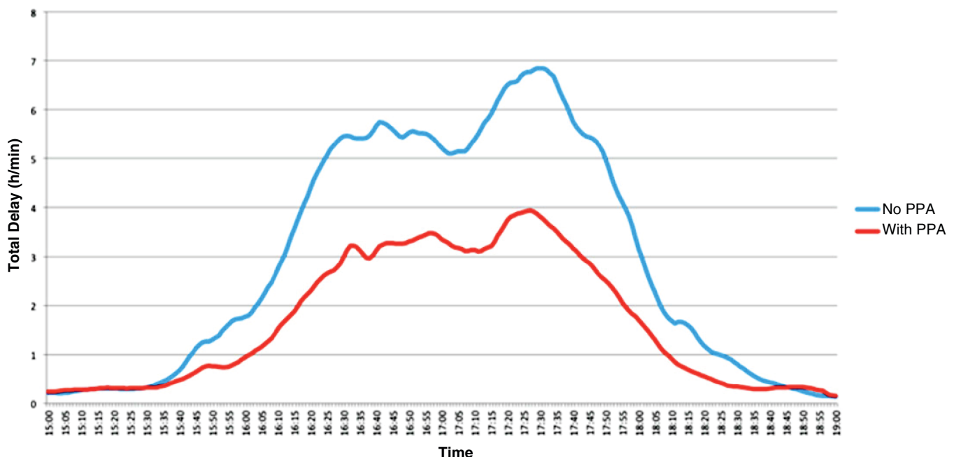
FIGURE 4 Average evolution of collective delays on A10 freeway [PPA = Praktijkproef Amsterdam (Practical Pilot Amsterdam)].
