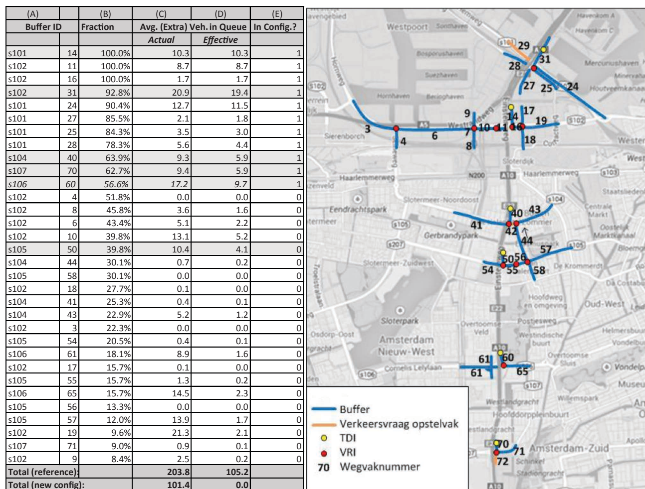
FIGURE 5 Calculation of effectively queued vehicles and estimation of effect of changing buffer configuration, based on collective delays computed per buffer in Beenker et al. (6). Buffers are shown in picture (only buffers directed toward A10 are considered and only in northbound direction) [veh. = vehicle; config. = configuration; VRI = intersection controller (translated from Dutch); TDI = ramp-metering installation (translated from Dutch)].
