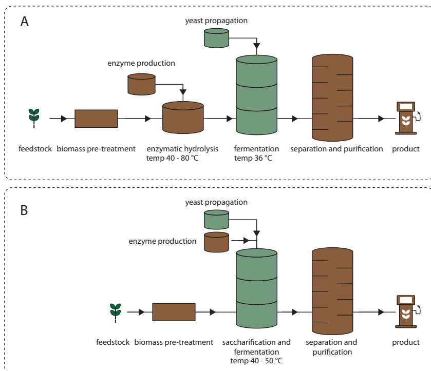
Figure 6. Schematic outline of yeast-based bioethanol production process. (A) separate enzymatic hydrolysis and fermentation or (B) simultaneous saccharification and fermentation (SSF).
