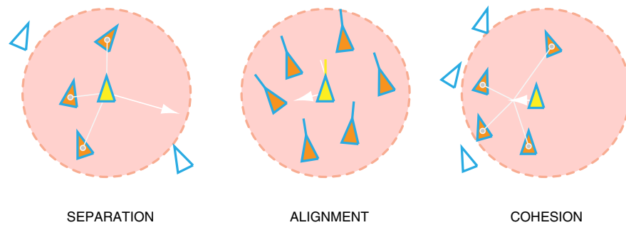
FIGURE 6.17 Diagrams of Craig Reynold's swarm behavior principles for the flocking simulation; separation, alignment, and cohesion. ( http://www.red3d.com/cwr/boids/ ).
