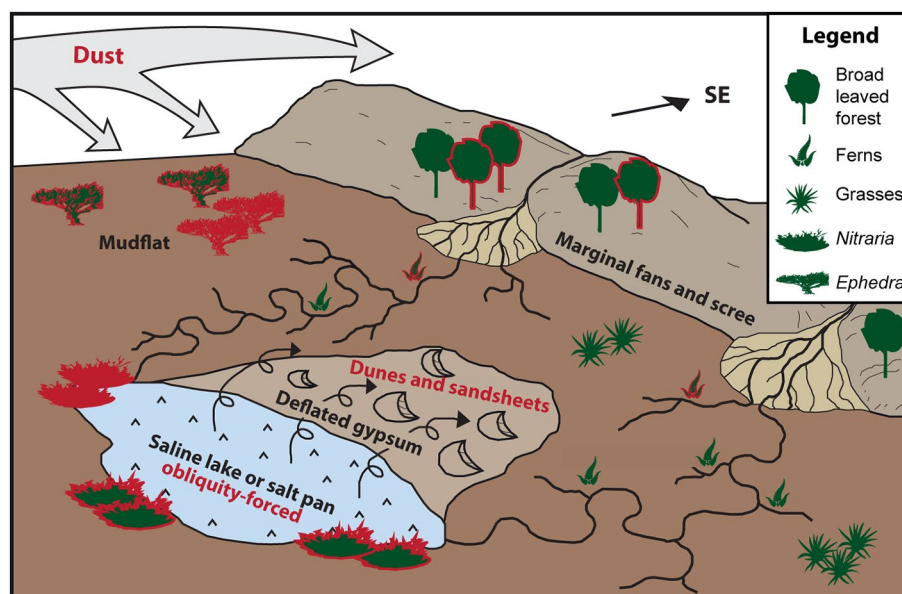
Figure 7. Depositional environment and paleovegetation of the Xining Basin during the Eocene (modified from Meijer et al., 2020). Dominant vegetation before 40 Ma is indicated in green, and after 40 Ma, in red (vegetation present throughout is colored in green with red outline). Sedimentary features appearing after 40 Ma are also indicated in red.
