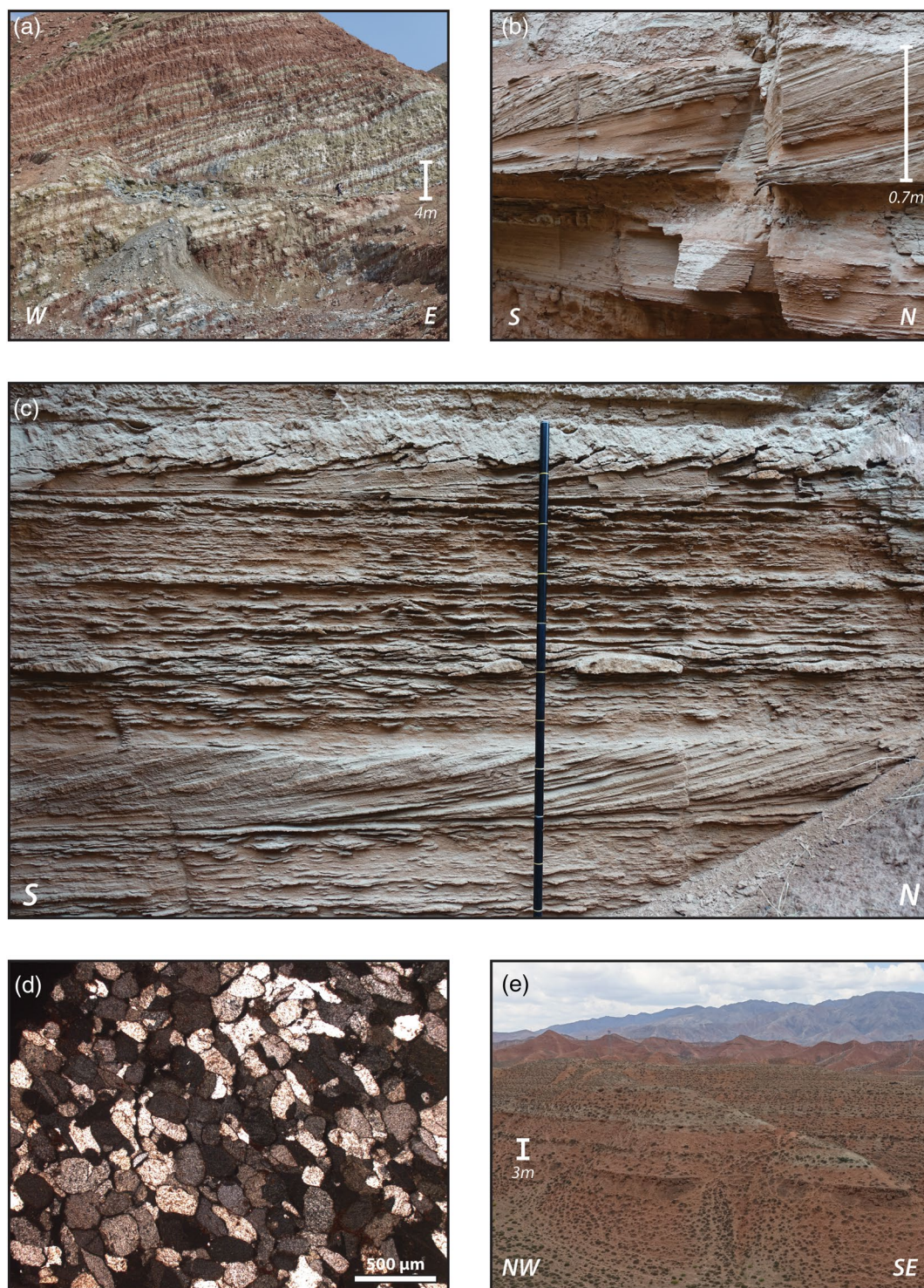
Figure 2. Pictures showing: (a) Cyclic alternations between red mudrocks and gypsum beds at the Xiejia section. (b) and (c) gypsarenites at the Baimasi section showing planar cross-bedding and horizontal bedding interpreted as eolian dunes and sand sheets respectively. (b) is at the 27 m-level and (c) at the 20 m-level with 10 cm markings on the Jacob's staff for scale. (d) thin section under plain-polarized light of the cross-bedded gypsarenite at the 27 m-level of the Baimasi section showing rounded and well-sorted grains of gypsum; (e) top of the Baimasi section showing regular ~3 m alternations between gypsum beds and red mudrocks characteristic of the upper Mahalagou Formation followed by brownish-red mudrocks characteristic of the Xiejia Formation.
