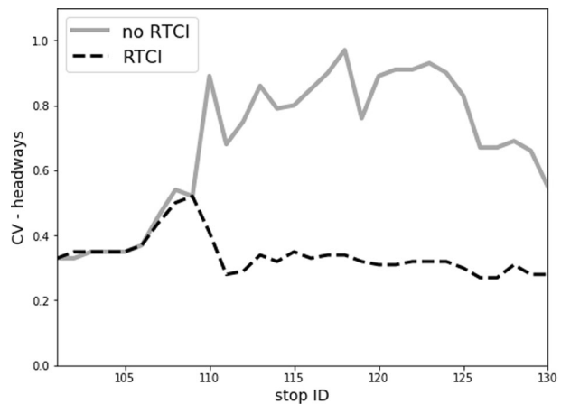
Fig. 5 The coefficient of bus headway variation along the line route in the no RTCI vs. RTCI scenarios, evaluated for peak (intermediate) trips
