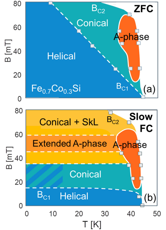
FIG. 4. Proposed phase diagrams of \text{Fe}_{0.7}\text{Co}_{0.3}\text{Si} deduced from the SANS patterns and intensities for (a) zero field cooling (ZFC) and (b) slow field cooling (Slow FC) showing the helical, conical, and A phases. The slow FC diagram of panel (b) also shows the extended A phase as well as the B - T areas where helical or skyrmion lattice correlations coexist with the conical phase.
