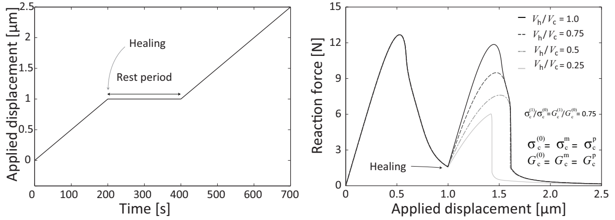
(a) Time history of the specified displacement. (b) Reaction force for vs. applied displacement
