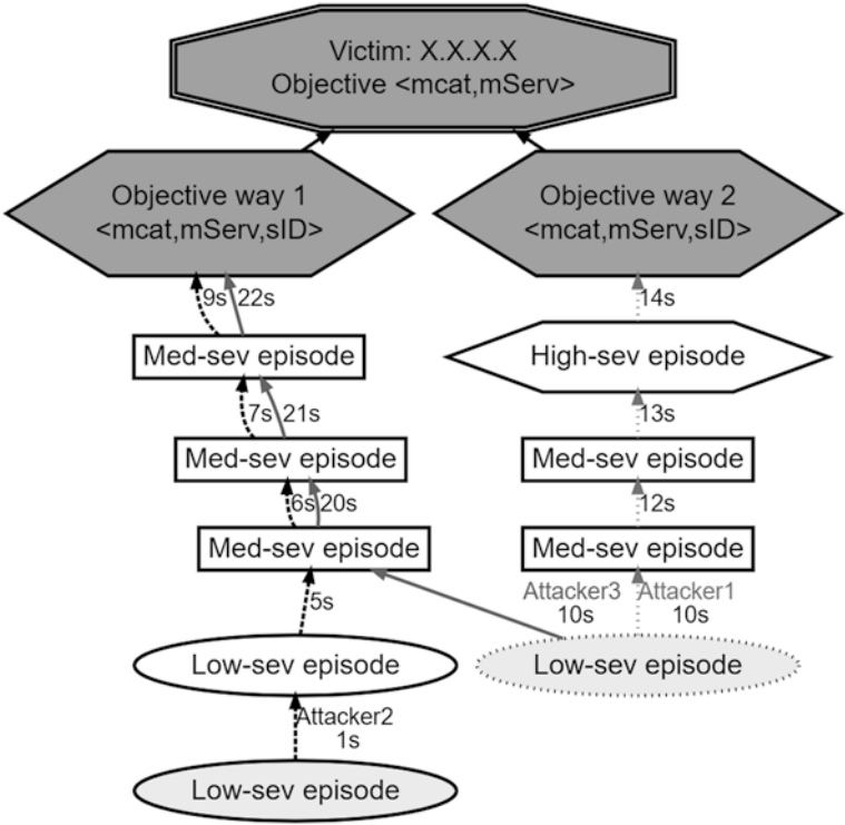
Fig. 6.8 A notional alert-driven attack graph showing paths towards an objective. Each vertex represents an episode. The vertex labels are <mcats, mServ, sID>, reflecting the AIF attack stage, targeted service, and state identifier from S-PDFA. The vertex shape indicates the episode severity. The root nodes reflect the attacker’s objective and the victim host. The dotted vertices reflect the sink states. The edges show attack progression and are annotated with the time since the first alert was captured. The attacker’s IP address is stated next to the first action in an attack path. (Adapted from Nadeem et al., 2021c)
