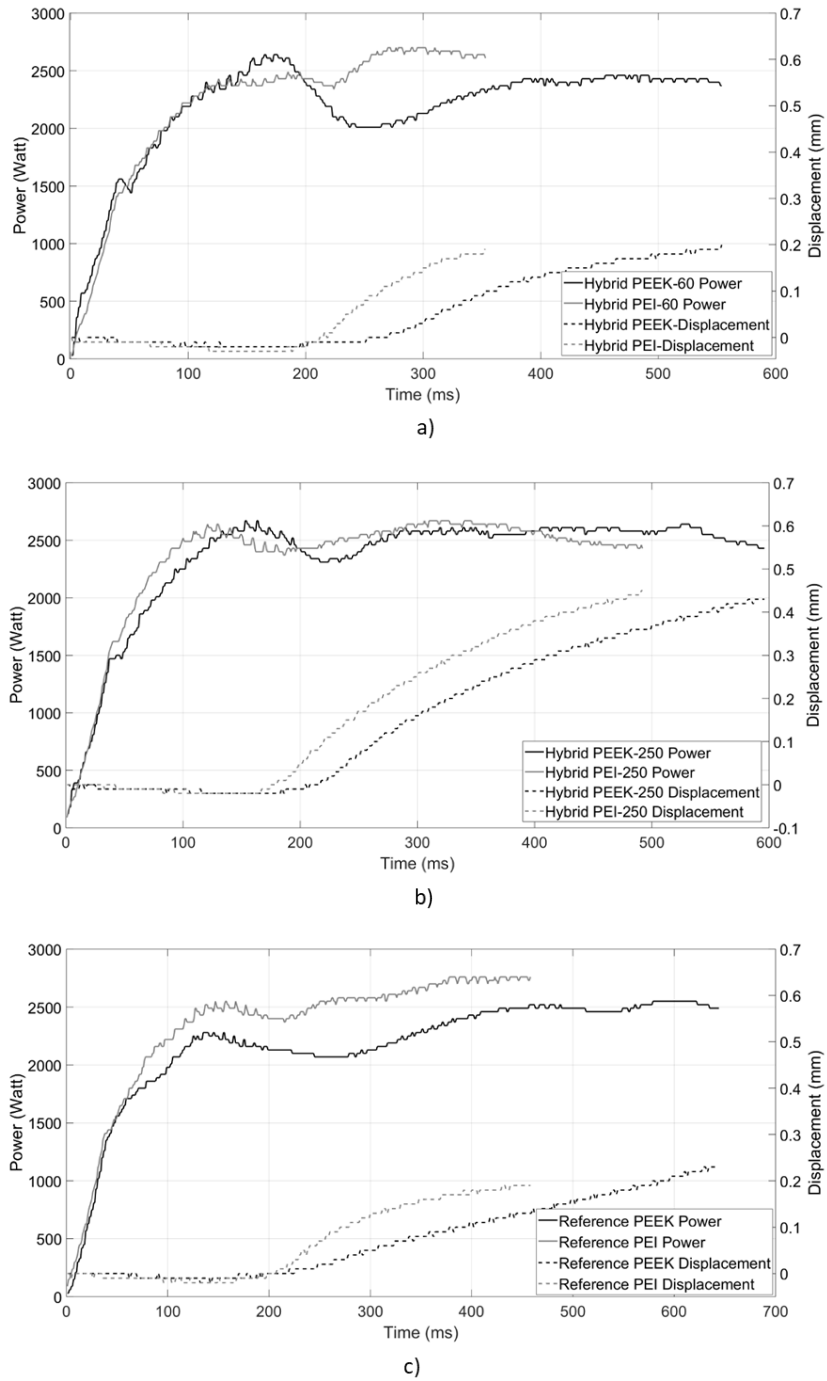
Figure 3.8: Power (solid line) and displacement (dotted line) curves of the a) hybrid-60 b) hybrid-250 and c) reference configurations.
