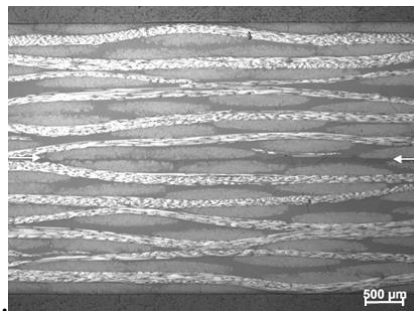
Figure 3.15: Cross-sectional micrograph a reference PEI sample. The weld line thickness is similar to that of the resin-rich areas in the composites. White arrows indicate the weld line. A similar micrograph was obtained with the reference PEEK samples.
