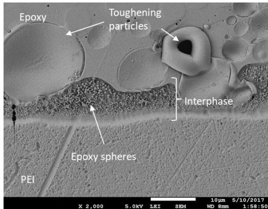
Figure 3.2: Morphology of the interphase formed between the epoxy and PEI materials.
