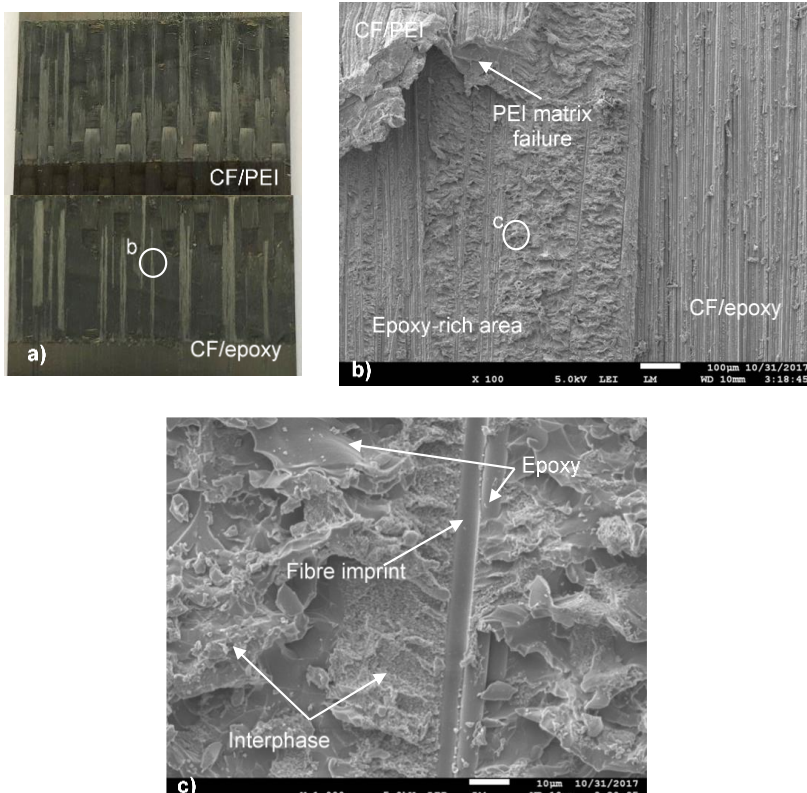
Figure 2.17: a) Representative fracture surfaces of a reference co-cured sample, showing failure in the two composites adherends characterised by exposed fibers and resin failure, b) SEM image corresponding in the circled area in (a), matrix failure in the CF/PEI adherend, exposed fibres in the CF/epoxy adherend and matrix failure, and c) a more detailed SEM image showing failure in the interphase and epoxy matrix.
