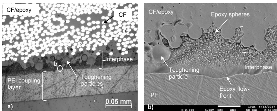
Figure 2.4: Cross-section images of an etched sample cut from the CF/epoxy/PEI laminate obtained via a) optical microscopy, in which the interphase can be seen as a dark grey area between the epoxy and the PEI resin (both with lighter grey colours) and b) SEM, which shows an interphase with a gradient morphology.
