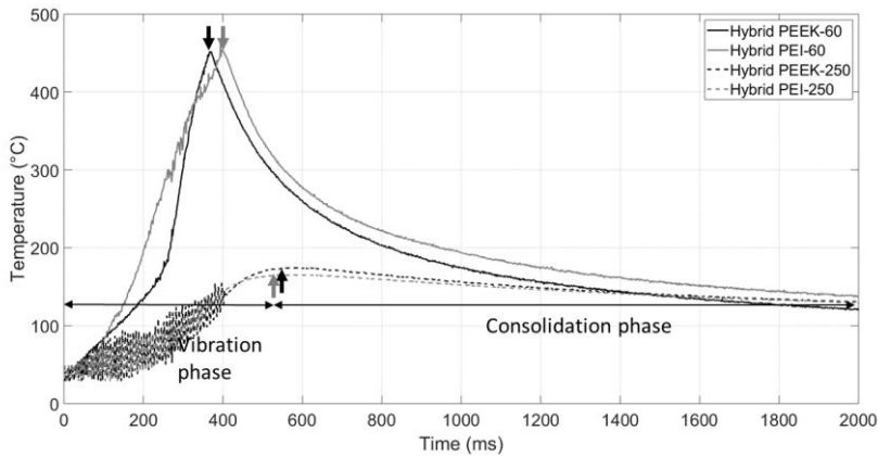
Figure 3.10: Temperature evolution between the coupling layer and the CF/epoxy adherend (see schematic in Figure 5b). The vertical arrows indicate when the vibration phase was stopped.
