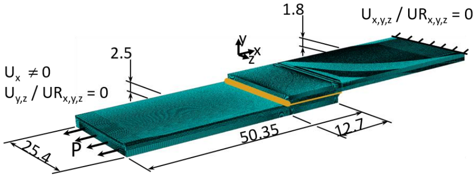
Figure A.1: 3D FE-model of the epoxy-PEEK 250 sample in a single-lap configuration, with boundary conditions. Dimensions are in [mm].
