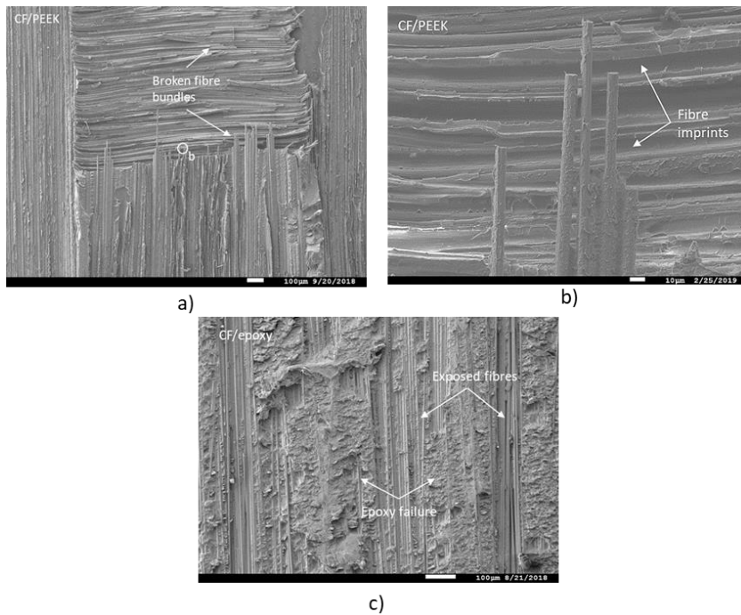
Figure 3.17: a) SEM detail of the circled area “a” in Figure 3.16b, showing broken fibre bundles of the CF/PEEK adherend attached on the CF/epoxy adherend, b) SEM detail of the circled area “b” in (a) showing fibres covered in PEEK resin and fibre imprints and c) SEM detail of the circled area “c” in Figure 3.16b showing failure in the CF/epoxy characterized by epoxy resin failure and exposed fibres. Note that the above-mentioned SEM micrographs also apply to the hybrid PEI-250 configuration.
