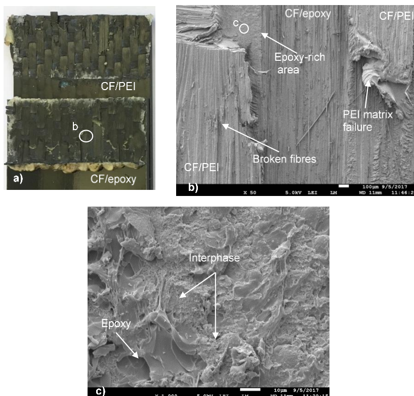
Figure 2.16: a) Representative fracture surfaces of a reference ED sample welded at 0.13 mm displacement, showing failure mostly in the CF/PEI adherend, with only partial failure in the CF/epoxy adherend. b) SEM image corresponding to the circled area in (a), showing broken CF/PEI bundles and exposed fibres in the CF/epoxy adherend, c) SEM image showing failure in the epoxy and interphase.
