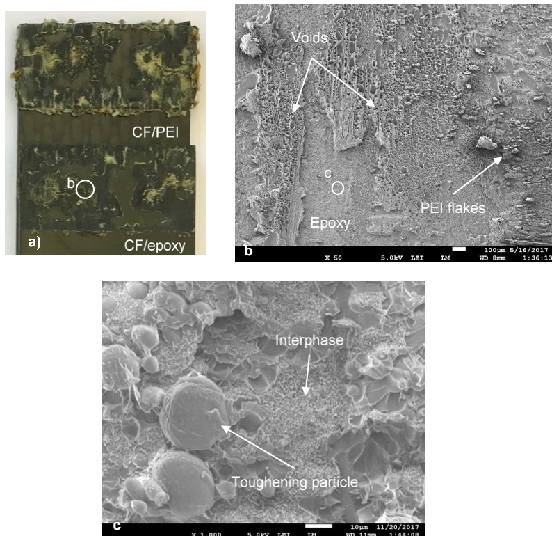
Figure 2.13: a) Representative fracture surfaces of an ED-less-60 case sample showing large unwelded areas and signs of thermal degradation of the PEI resin. b) SEM image corresponding to the circled area in (a), depicting voids in the PEI resin and PEI resin flakes, both features associated with thermal degradation and c) is a detailed SEM image showing failure in the interphase.
