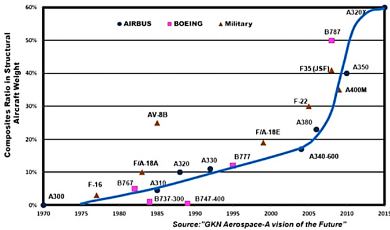
Figure 1.1: Use of composites in commercial and military aircraft in the last decade. Image adapted from [6]
