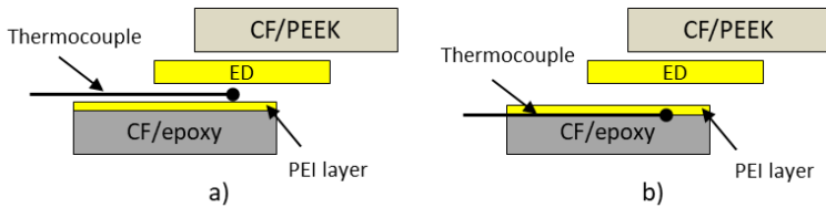
Figure 3.5: Schematic representation of the temperature measurements. a) thermocouple at the welding interface between the ED and the CF/epoxy/PEI adherend and b) thermocouple between the PEI coupling layer and the CF/epoxy adherend.
