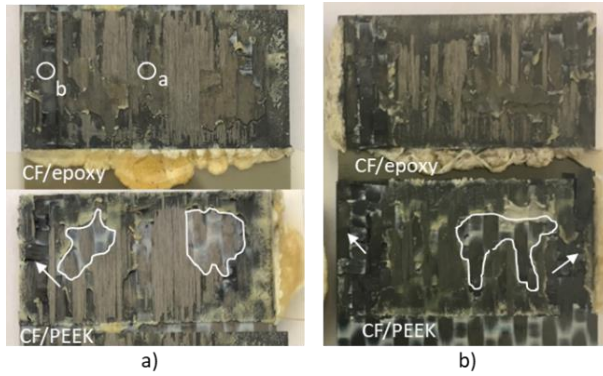
Figure 3.18: Fracture surfaces of a) a hybrid PEI-60 sample and b) a hybrid PEEK-60 sample. The unwelded areas are highlighted by the white lines. The locations where failure in the CF/PEEK adherend occurred is indicated by the white arrows.
