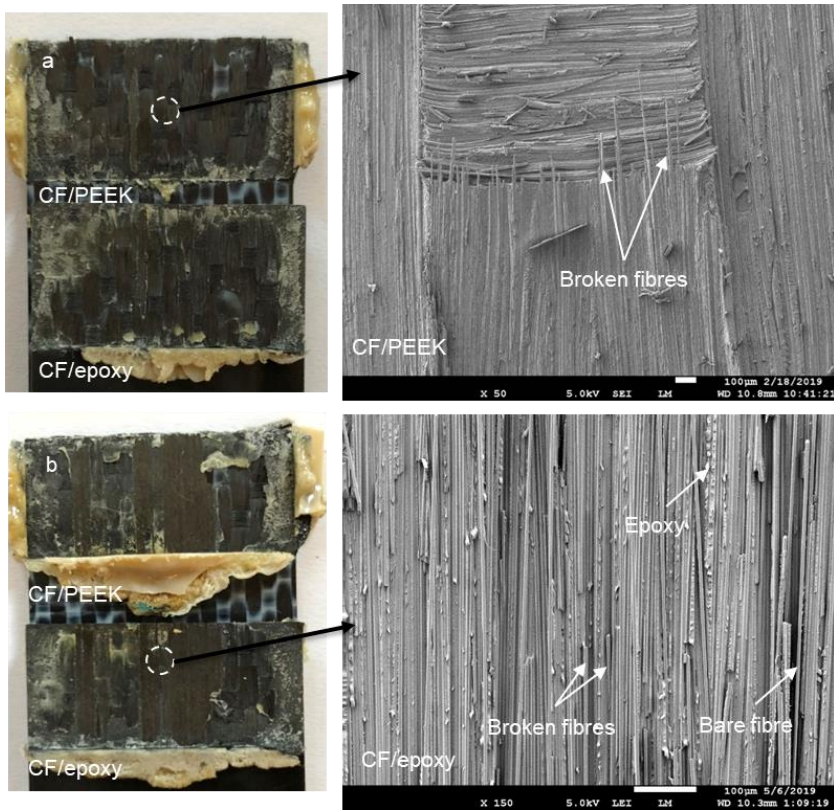
Figure 4.3: Closer inspection of the fracture surfaces of epoxy-PEEK 250 joints welded at a) d_{opt} , showing failure in the CF/PEEK adherend, characterized by ruptured resin and broken fibres and b) at 0.38 mm, i.e. right above d_{high} , depicting failure in both adherends with failure in the CF/epoxy adherend characterized by exposed and broken fibres.
