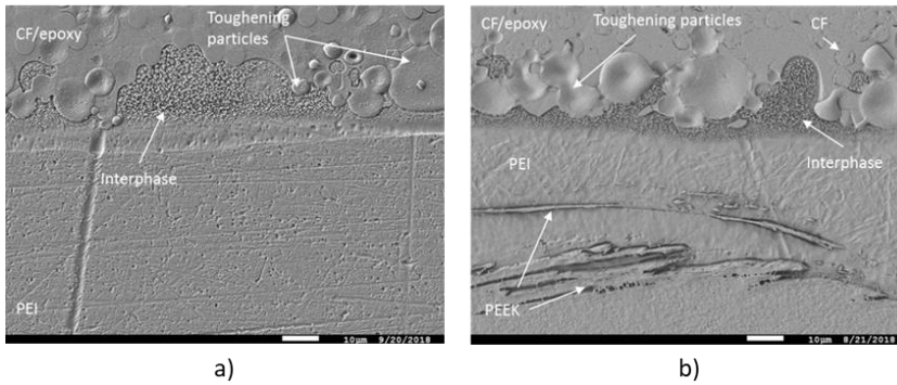
Figure 3.14: SEM micrographs of the cross-sections of a) a hybrid PEI 250 sample and b,c) a hybrid PEEK-250 sample. For both configurations, the interphase seems intact after the welding process.
