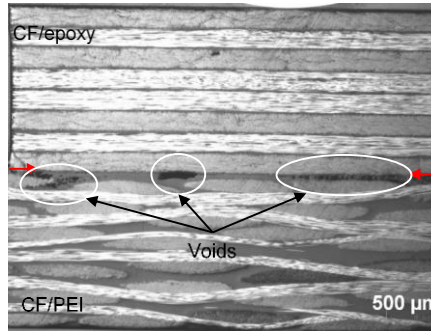
Figure 2.7: Cross-sectional micrograph close to the edge of an ED-less-60 sample welded at 500 J. Porosity can be seen within the weld line. Red arrows indicate the weld line.
