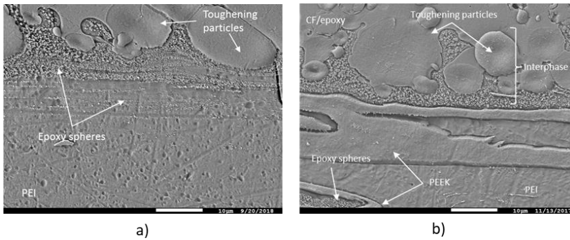
Figure 3.13: SEM micrographs of the cross-sections of a) a hybrid PEI 60 sample and b) a hybrid PEEK-60 sample. The interphase was affected by the welding process for both configurations
