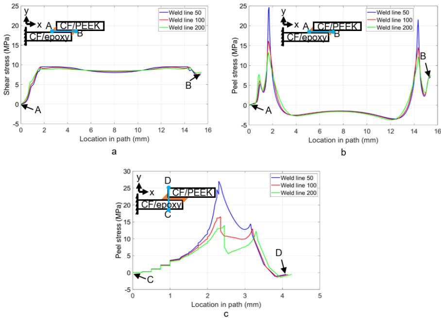
Figure 4.9: Stresses obtained from the FE-model. a) Shear stresses along the AB path, b) peel stresses along the AB path and c) peel stresses along the CD path.
