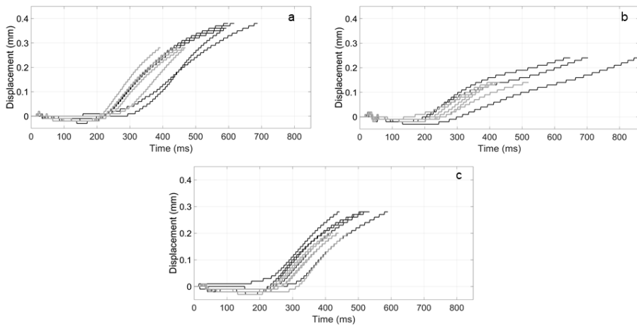
Figure 4.12: Displacement of the sonotrode during the welding process in the a) epoxy-PEEK 250, b) reference PEEK-PEEK and c) epoxy-PEEK 175 configurations. Note: grey curves correspond to specimens welded up to d_{low} ; black curves correspond to specimens welded up to d_{high} (see Table 4.2 and Table 4.3).
