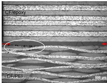
Figure 2.8: Cross-sectional micrograph close to the edge of an ED-less-250 case sample welded at 600 J. A thick weld line and porosity in the weld line can be observed. Red arrows indicate the weld line.
