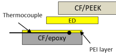
Figure 5.1: Schematic representation of thermocouple location in CF/epoxy adherends.
