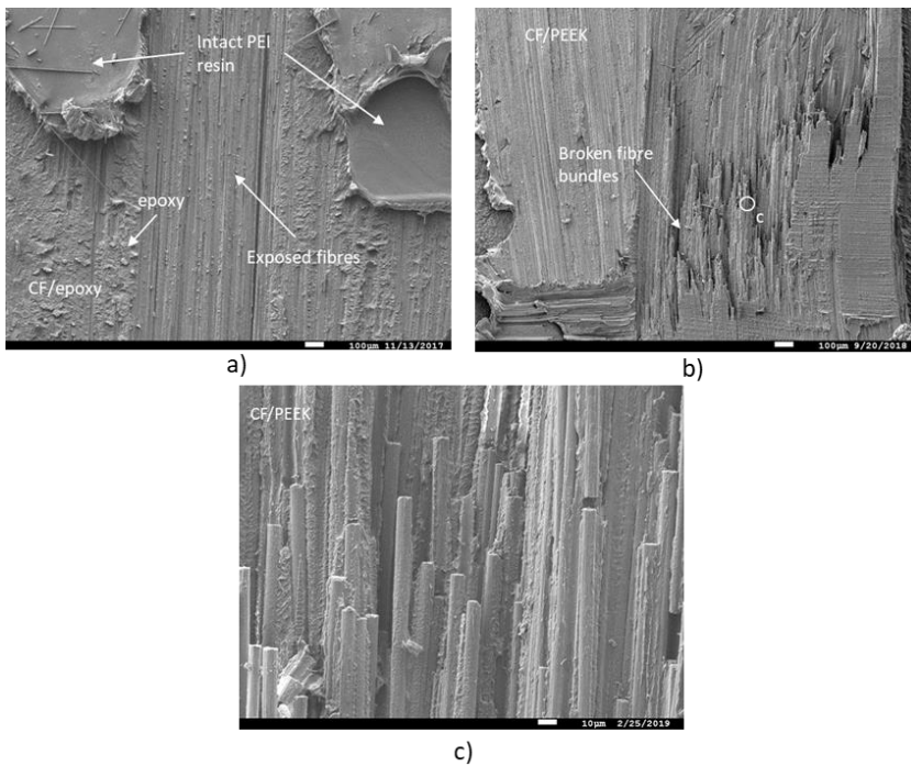
Figure 3.19: a) SEM detail of the corresponding circled area in Figure 3.18a, showing failure in the CF/epoxy characterized by epoxy resin failure exposed fibres and intact PEI resin, b) SEM detail of the corresponding circled area in Figure 3.18a showing broken fibre bundles of the CF/PEEK adherend attached on the CF/epoxy adherend and c) SEM detail of the corresponding circled area in (b) showing broken fibres covered in PEEK resin. Note that the SEM micrographs of the fracture surfaces were similar for both configurations, hence the micrographs apply to both hybrid-60 configurations.
