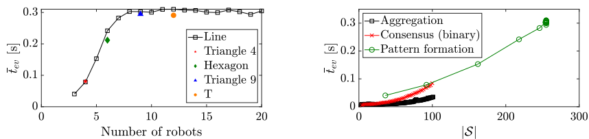
(a) Change in wall-clock time with the number of robots for the pattern formation task. Once the swarm reaches 9 or more robots (such that the local neighborhood of a robot could be entirely filled with 8 other robots) the wall-clock time does not scale.
