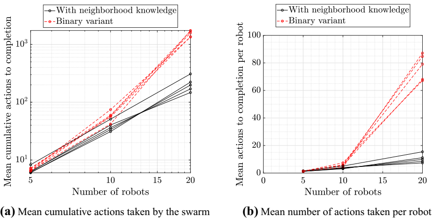
Fig. 7 Comparison of mean performance of the evolved policies for both variants of the consensus task for the case where M = 2
