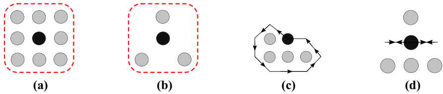
Fig. 10 Examples of: a a state s \in \mathcal{S}_{\text{blocked}} , due to it being surrounded; b a state s \in \mathcal{S}_{\text{blocked}} , because any motion will cause the swarm to locally disconnect; c a state s \in \mathcal{S}_{\text{active}} \cap \mathcal{S}_{\text{simplicial}} , because it can travel around all its neighbors; d a state s \in \mathcal{S}_{\text{active}} but s \notin \mathcal{S}_{\text{simplicial}} , because it can move but it cannot travel around all its neighbors or else it might disconnect the swarm
