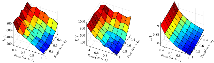
(a) Global performance of the solution space for a swarm of 20 robots in a 30\text{ m} \times 30\text{ m} arena. \bar{t}_c is the mean time taken before the task is completed.
