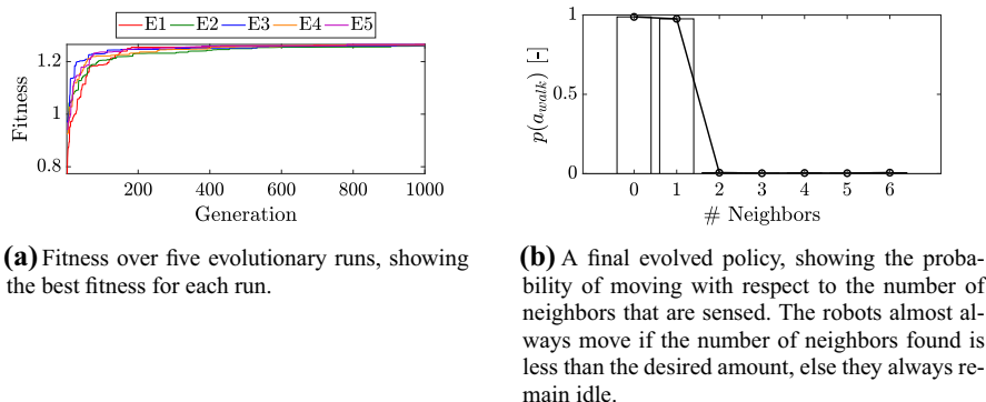
Fig. 21 Details of the evolution of the policy for the aggregation task, showing the increase in fitness a final evolved policy
