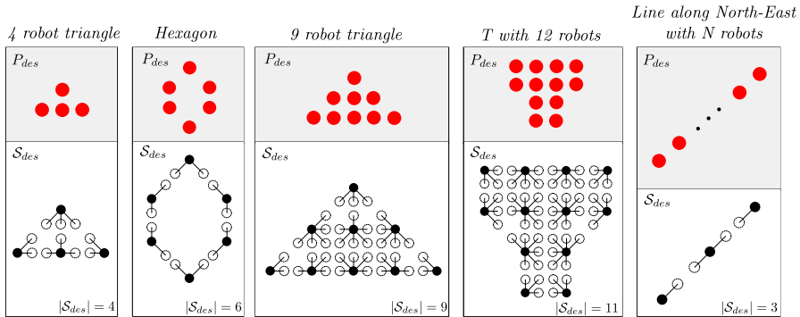
Fig. 9 Set of desired states S_{des} for the exemplary patterns treated in this paper, featuring patterns of increasing complexity and/or size. The set S_{des} can be intuitively extracted for each pattern as the “puzzle pieces” that compose it. Note that the T with 12 robots has 11 states in S_{des} . This is because the top state repeats. Also note that the line always only has three states in S_{des} , because the center state can repeat indefinitely
