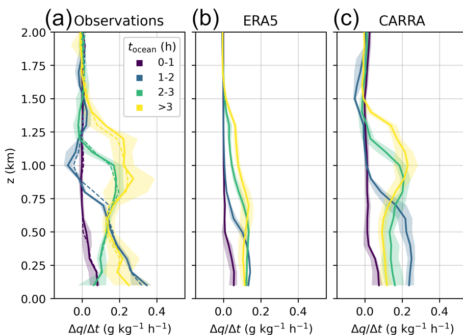
Figure 8. Moistening rates expressed as the change of specific humidity q per hour as a function of the time air masses spent over the ice-free ocean. Lines depict the mean values and shading the 25th–75th percentiles. (a) Moistening rates based on the quasi-Lagrangian drosonde observations. Solid lines are from ERA5 trajectories, and the dashed lines are from CARRA trajectories. (b) Corresponding moistening rates extracted from ERA5. (c) Corresponding moistening rates extracted from CARRA.
