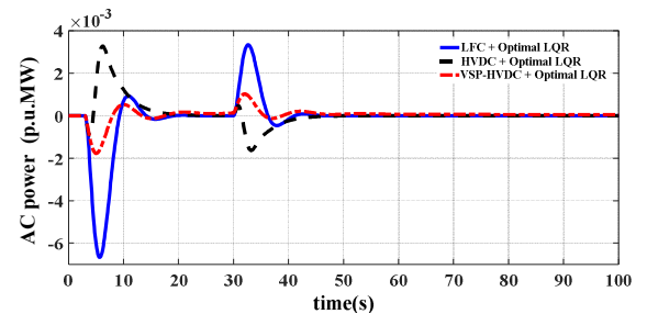
Fig. 9. AC power deviation: comparison between mathematical models (LFC, HVDC, VSP-HVDC) in the third scenario.
