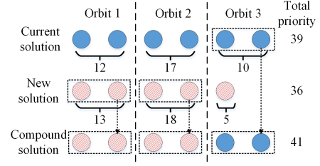
Figure 1: An example of partial sequence dominance
