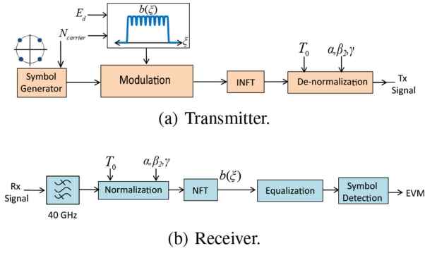
Fig. 7. Simulation setup of NFDm system with continuous spectrum modulation. The transmission link is the same as described before in Fig. 2(b), (c).
