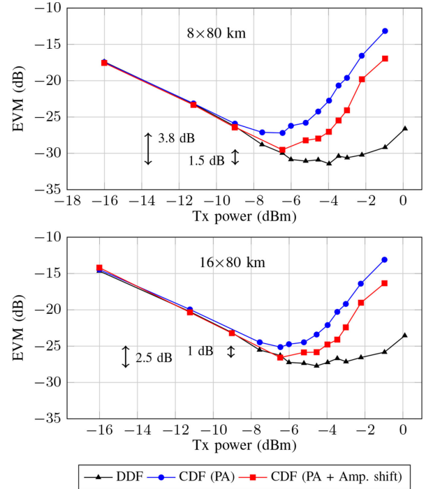
Fig. 9. Continuous spectrum modulation : EVM over transmit power for different transmission distances.
