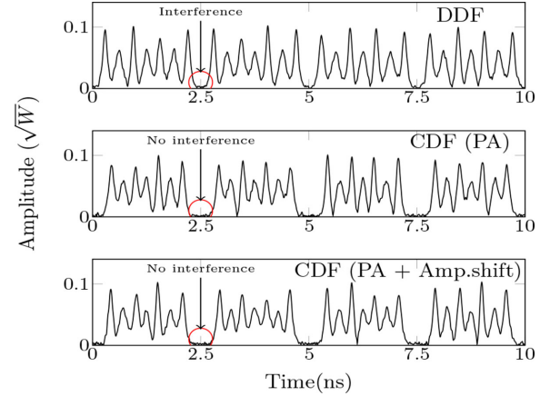
Fig. 5. Signal after 16 \times 80 km transmission over different link-configurations (at transmit power of 2.8 dBm). The pulses spread more for the case of DDF, resulting into interference among them.
