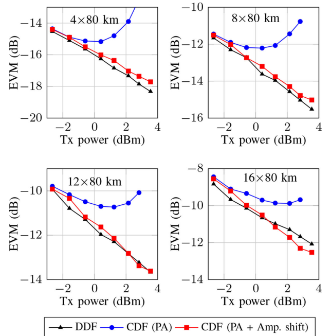
Fig. 6. Discrete spectrum modulation : EVM over transmit power for different transmission distances.
