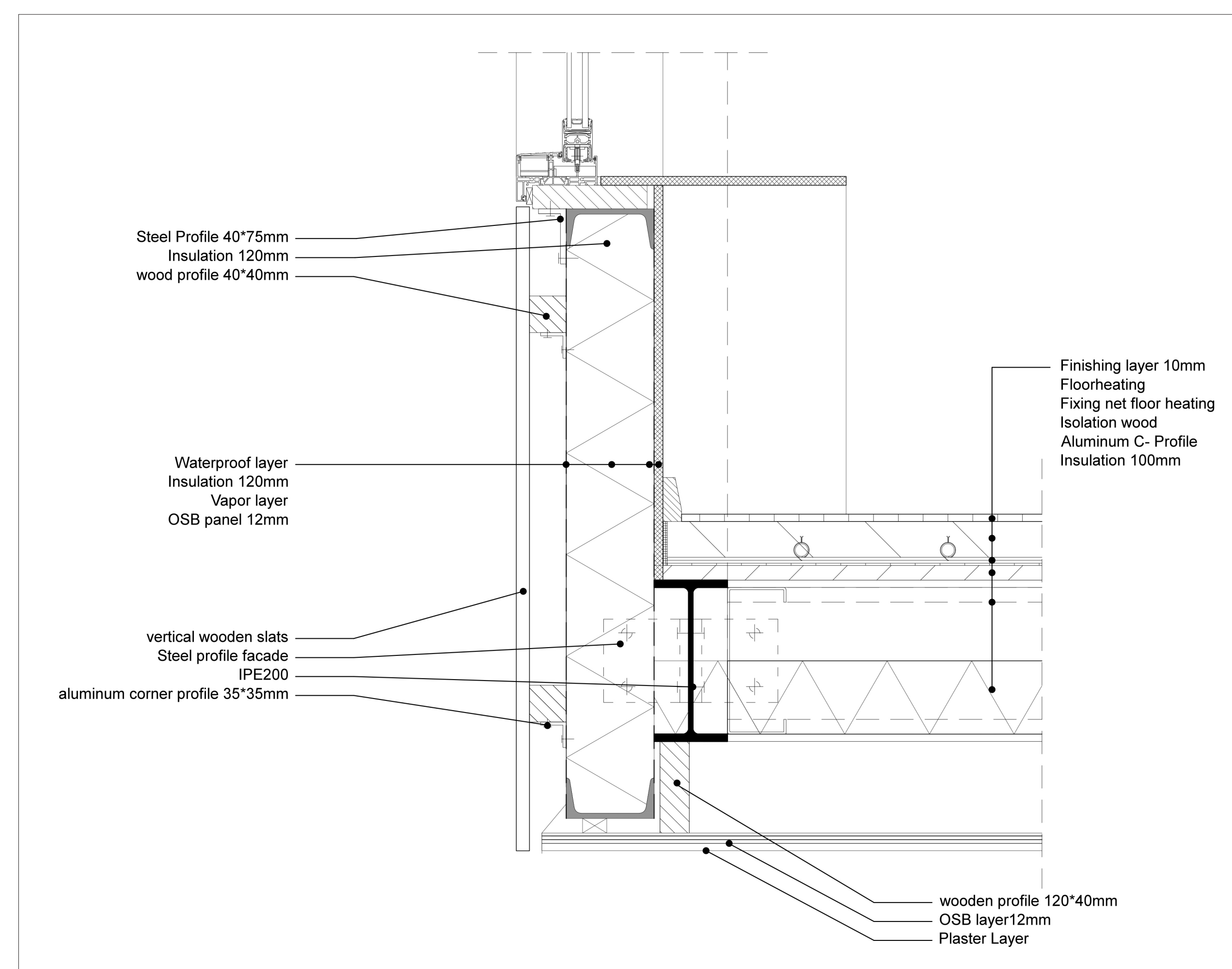
Detail 04 1:5
