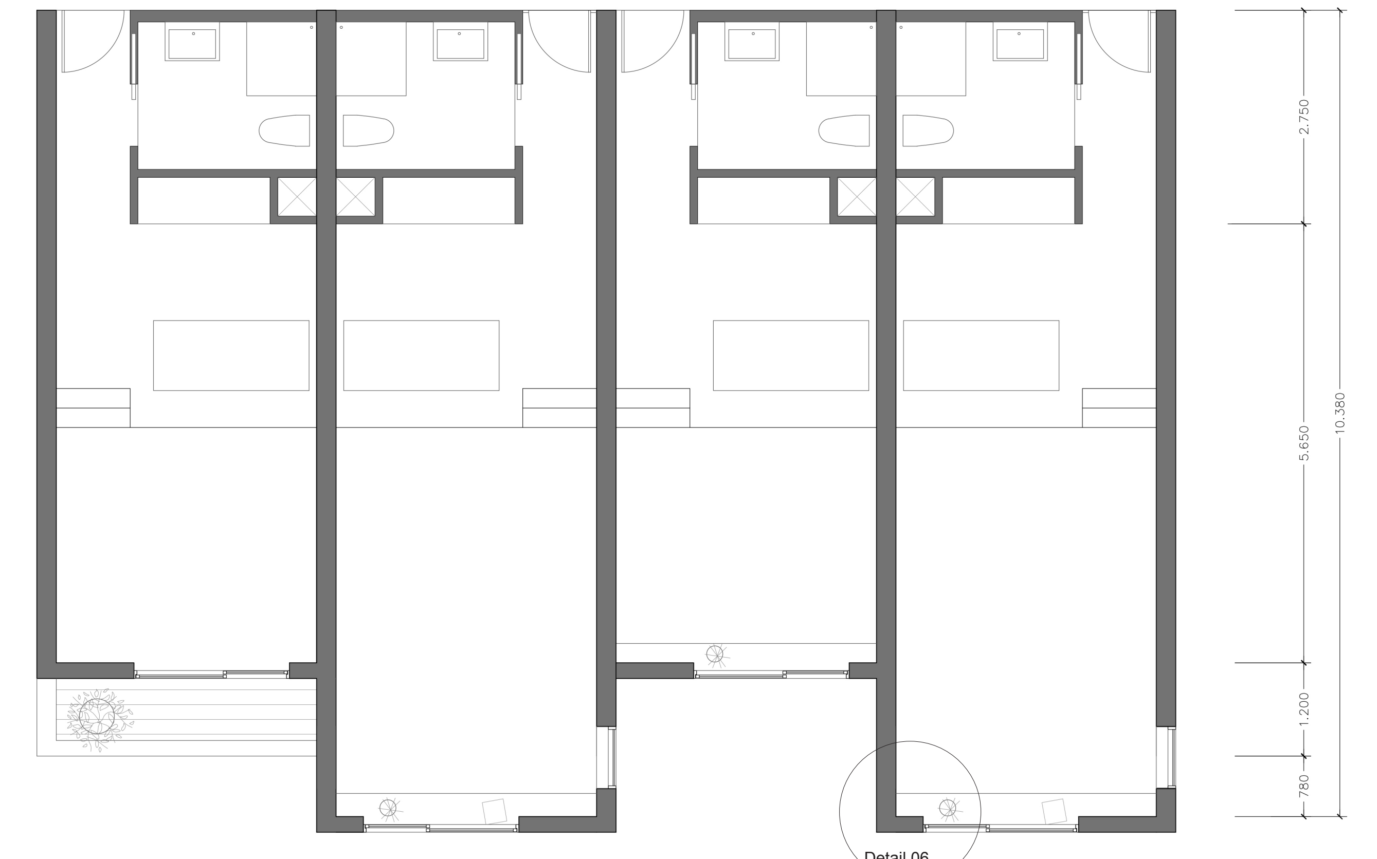
Third Floor plan 1:50
