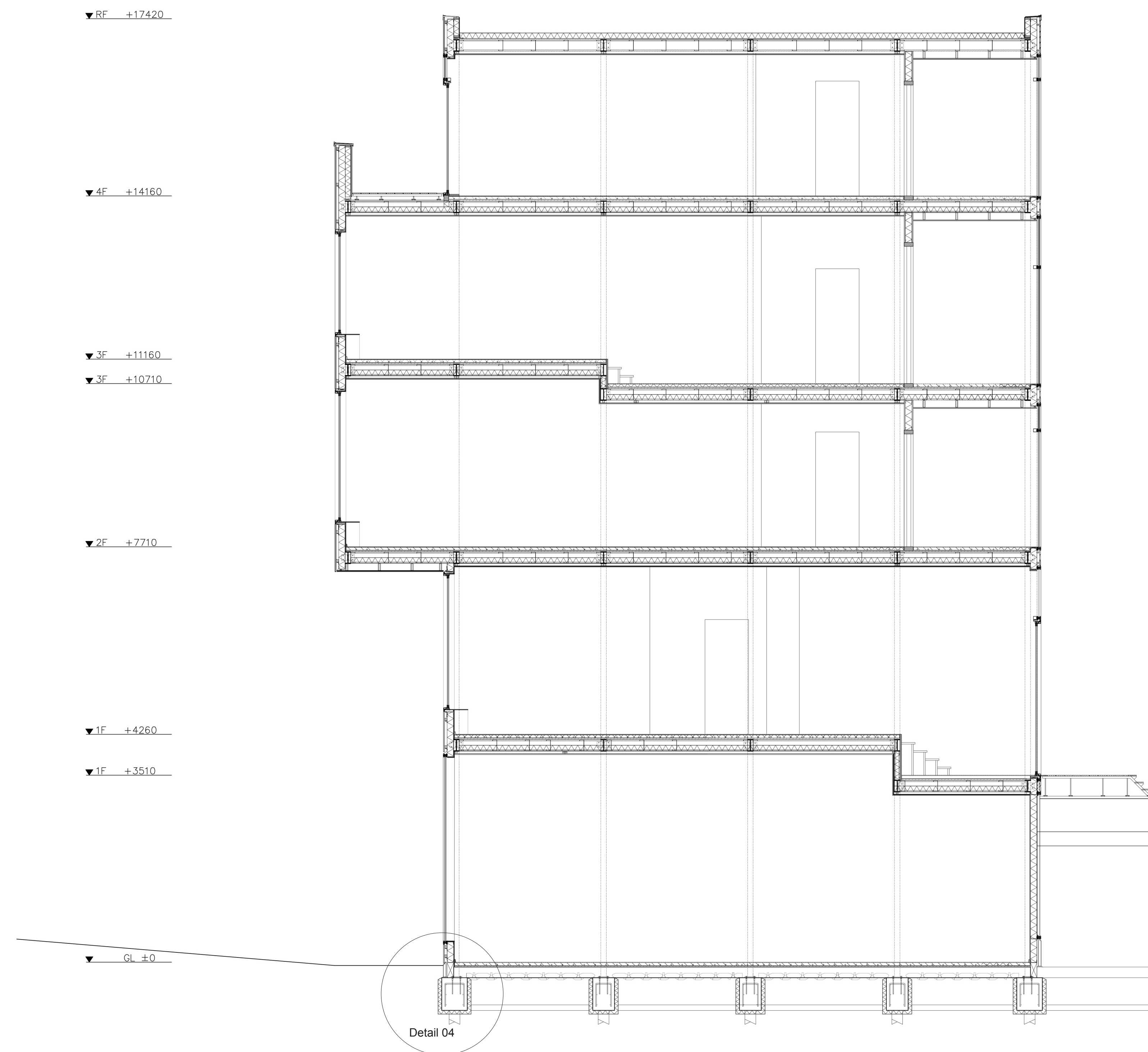
Section 1:50
