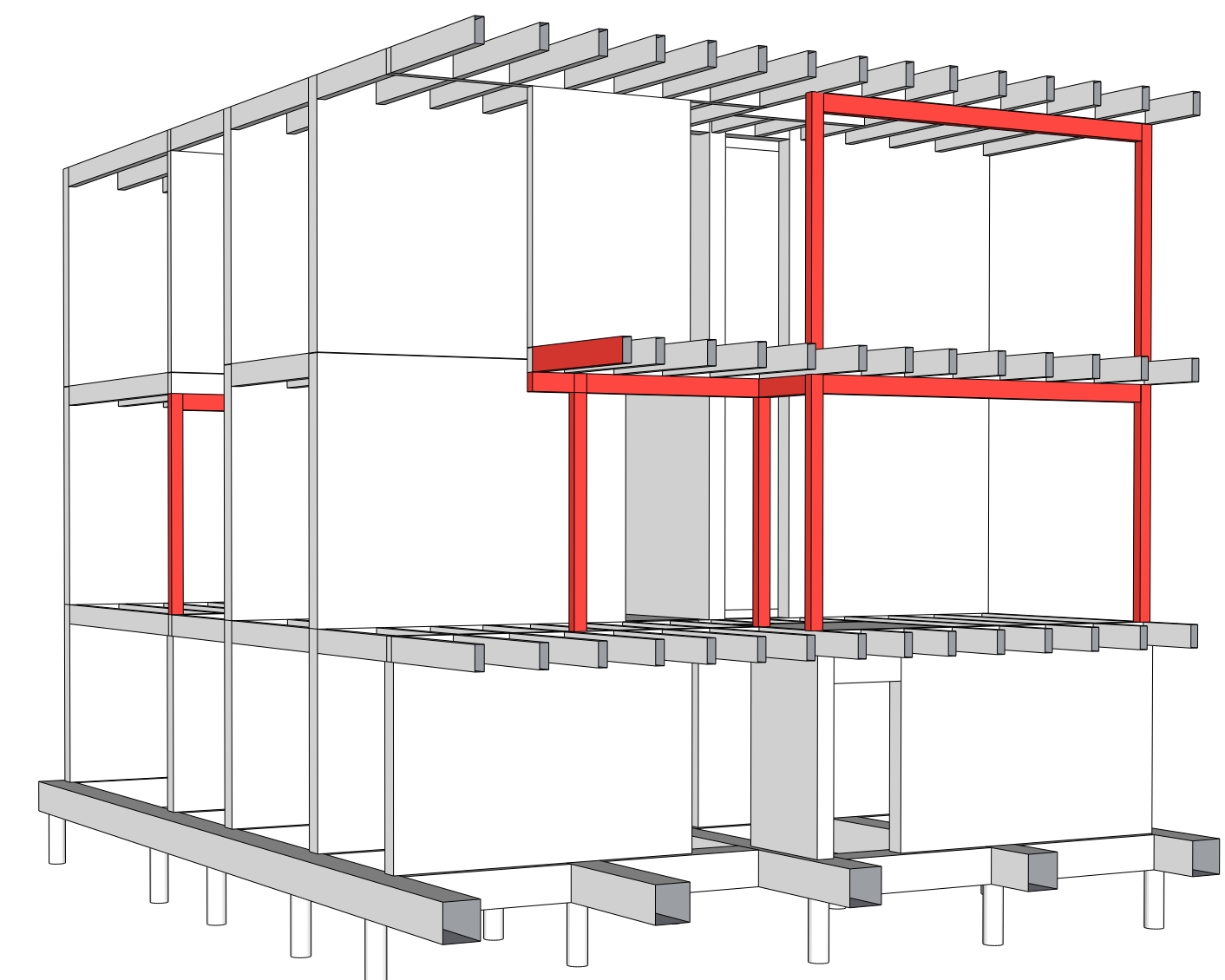
Construction Scheme
