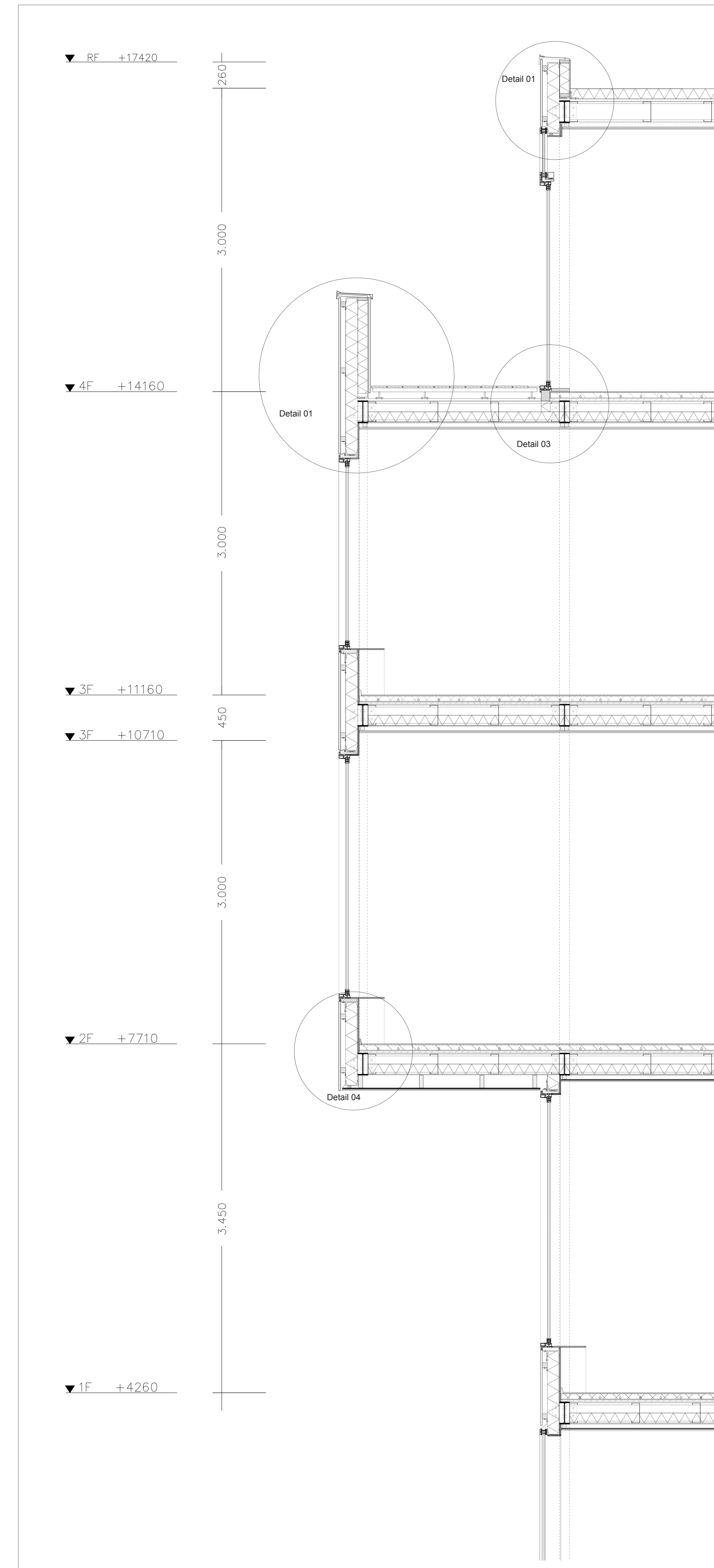
Single housing section 1:20
