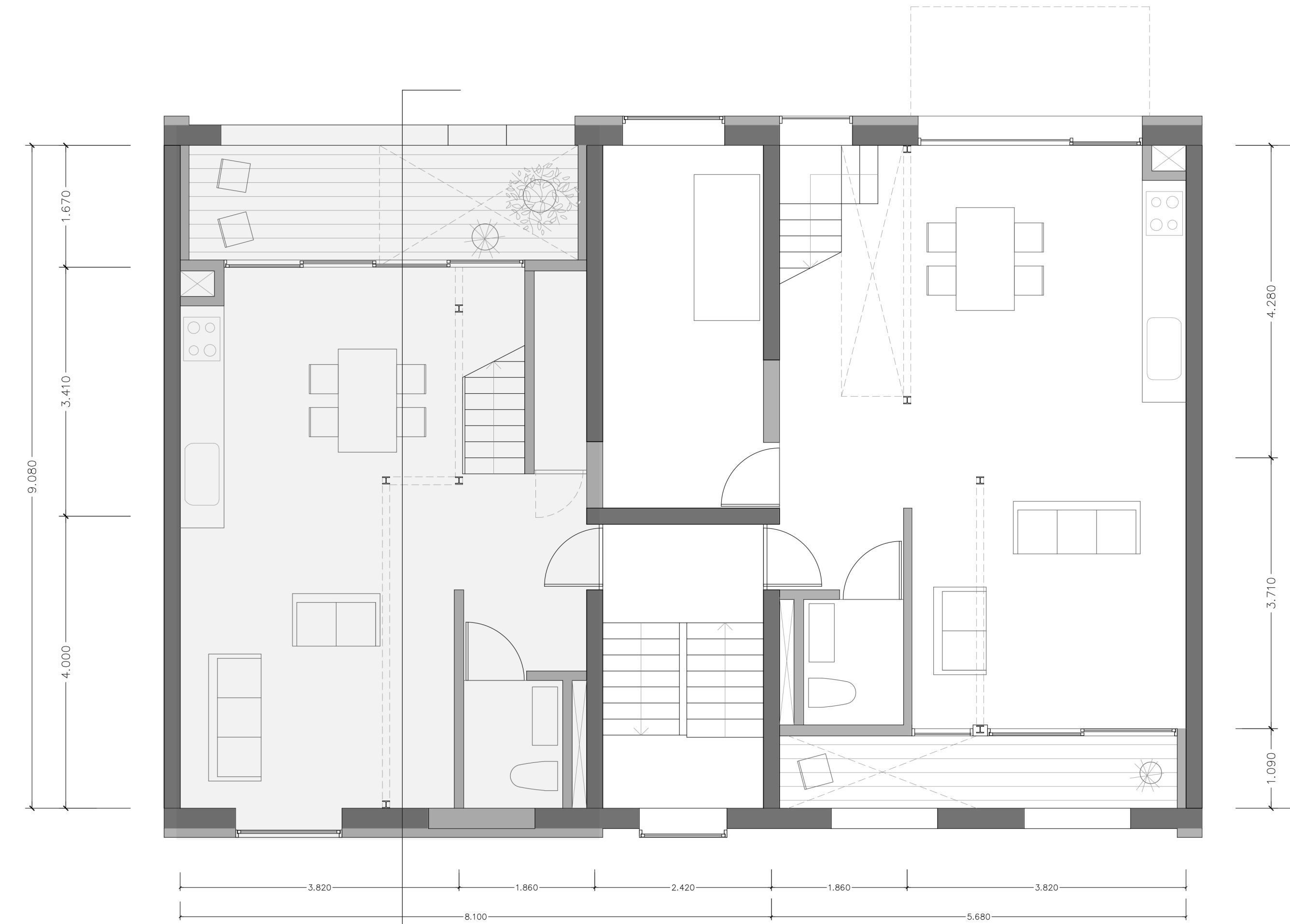
First Floor Plan 1:50
