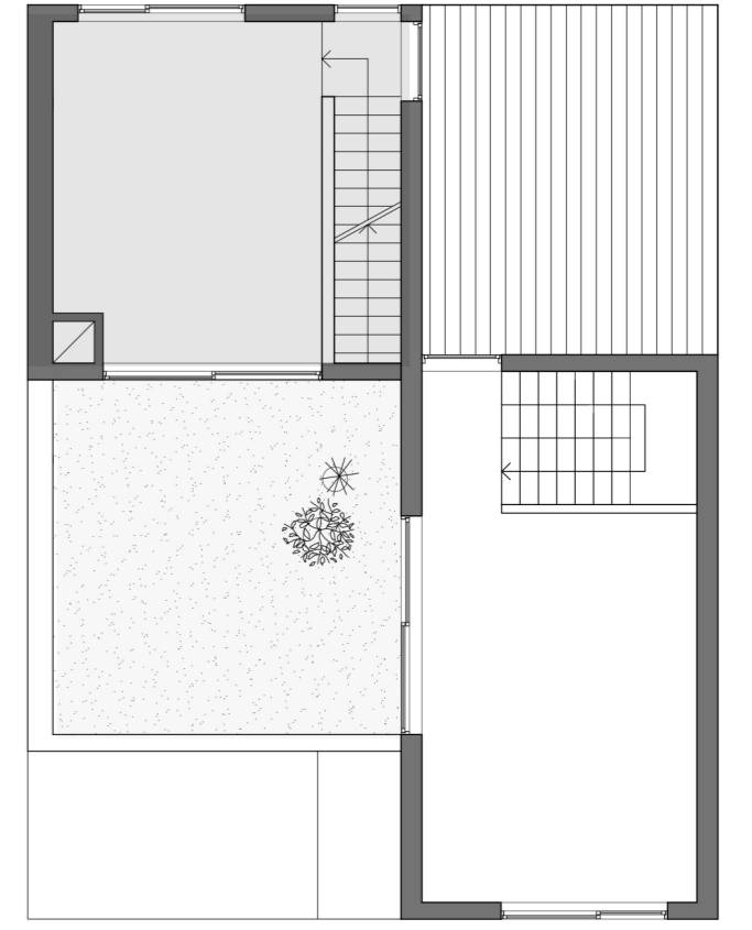
Fifth Floor Plan 1:100
