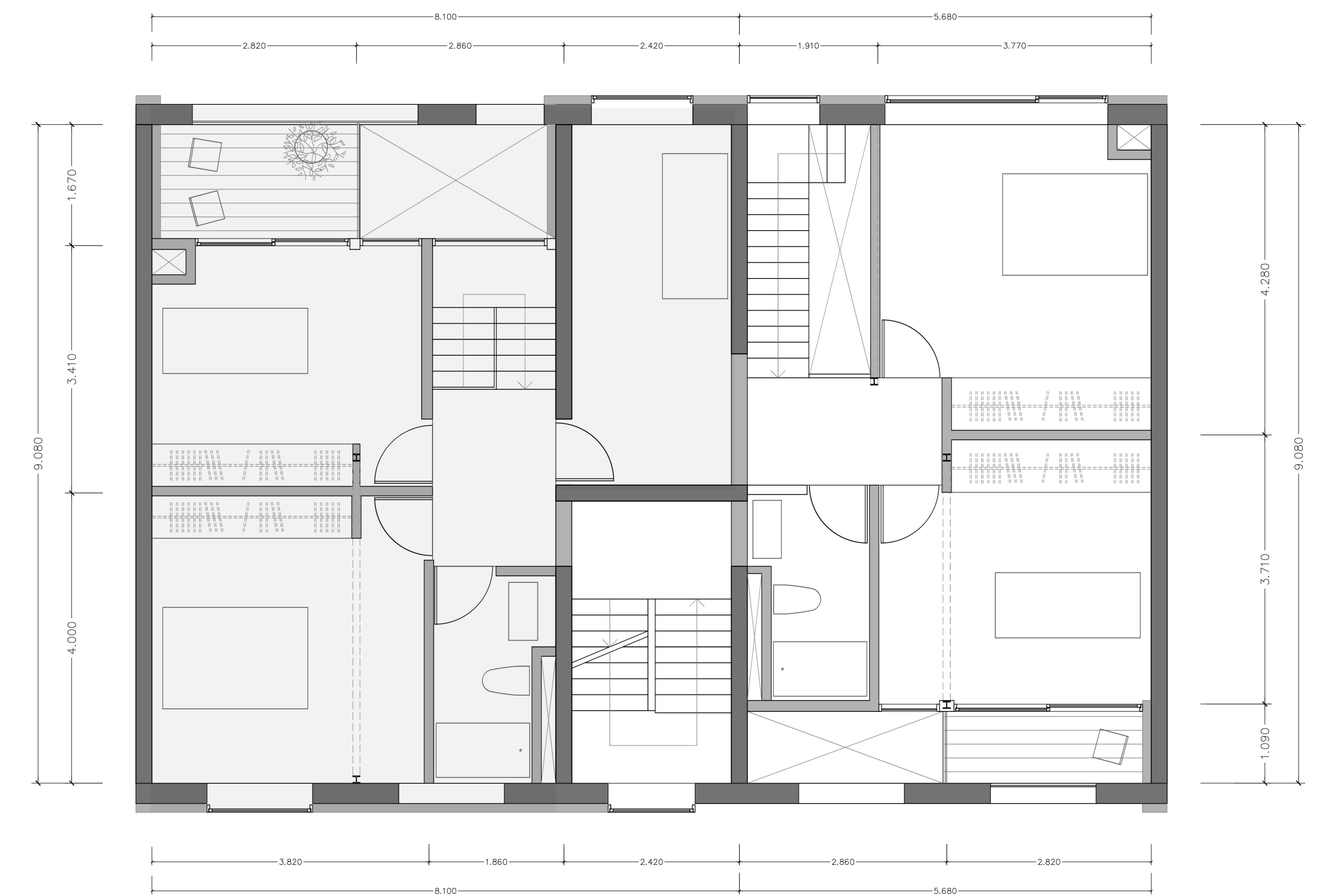
Second Floor Plan 1:50
