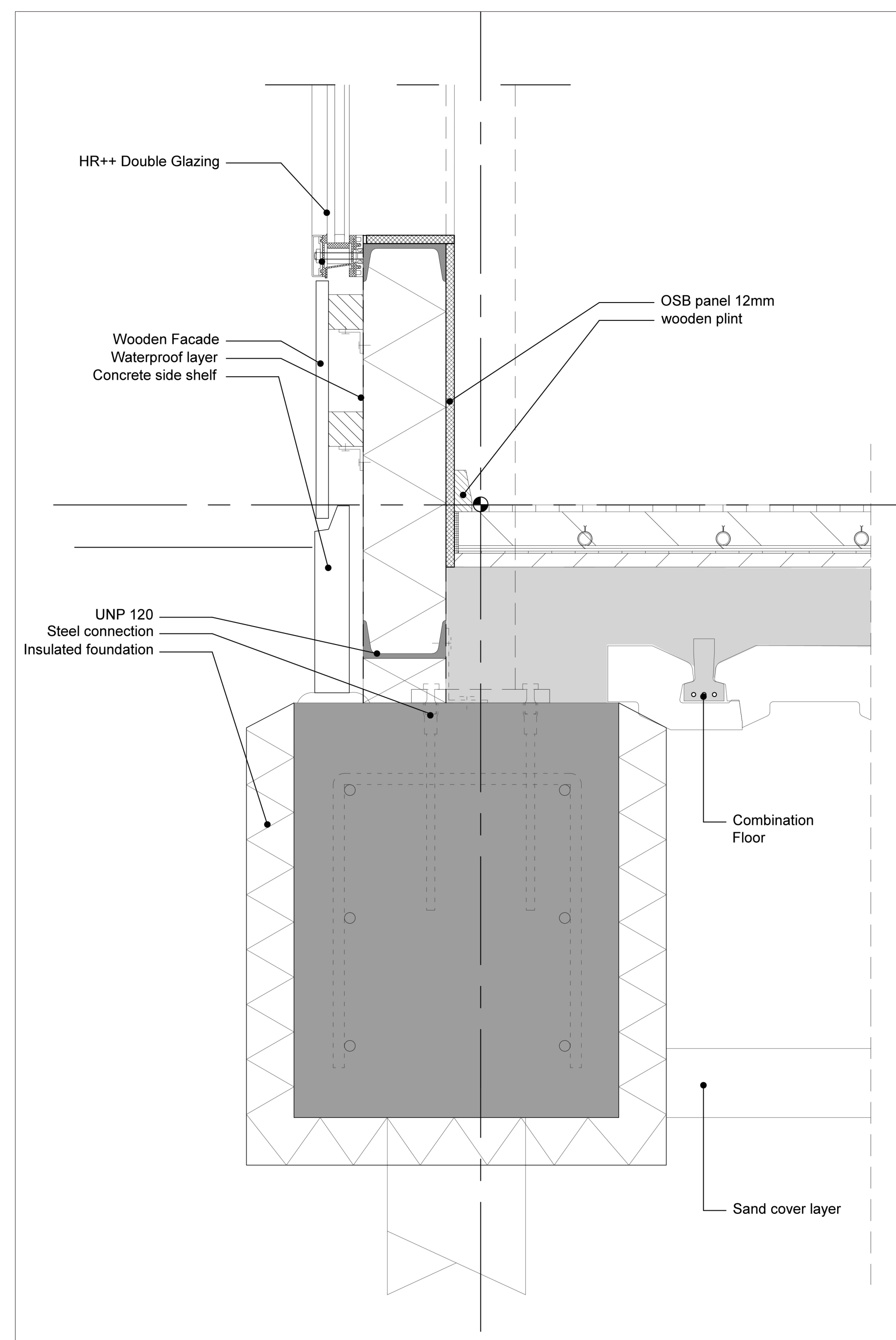
Detail 05 1:5
