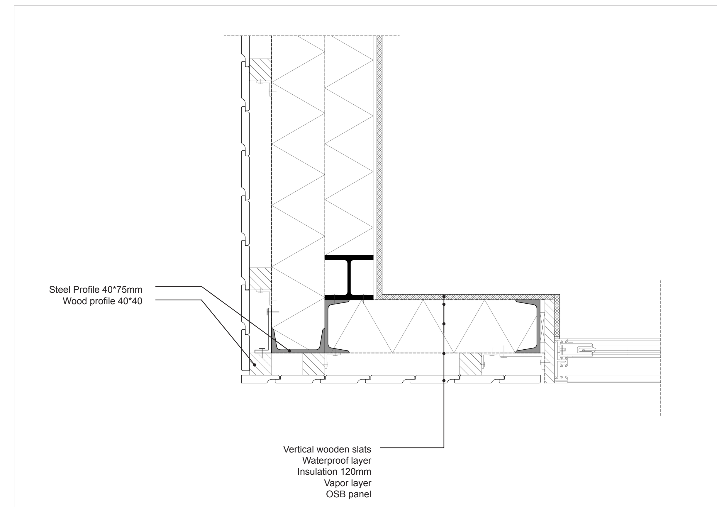
Detail 06 1:5
