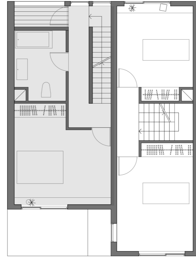
Fourth Floor Plan 1:100
