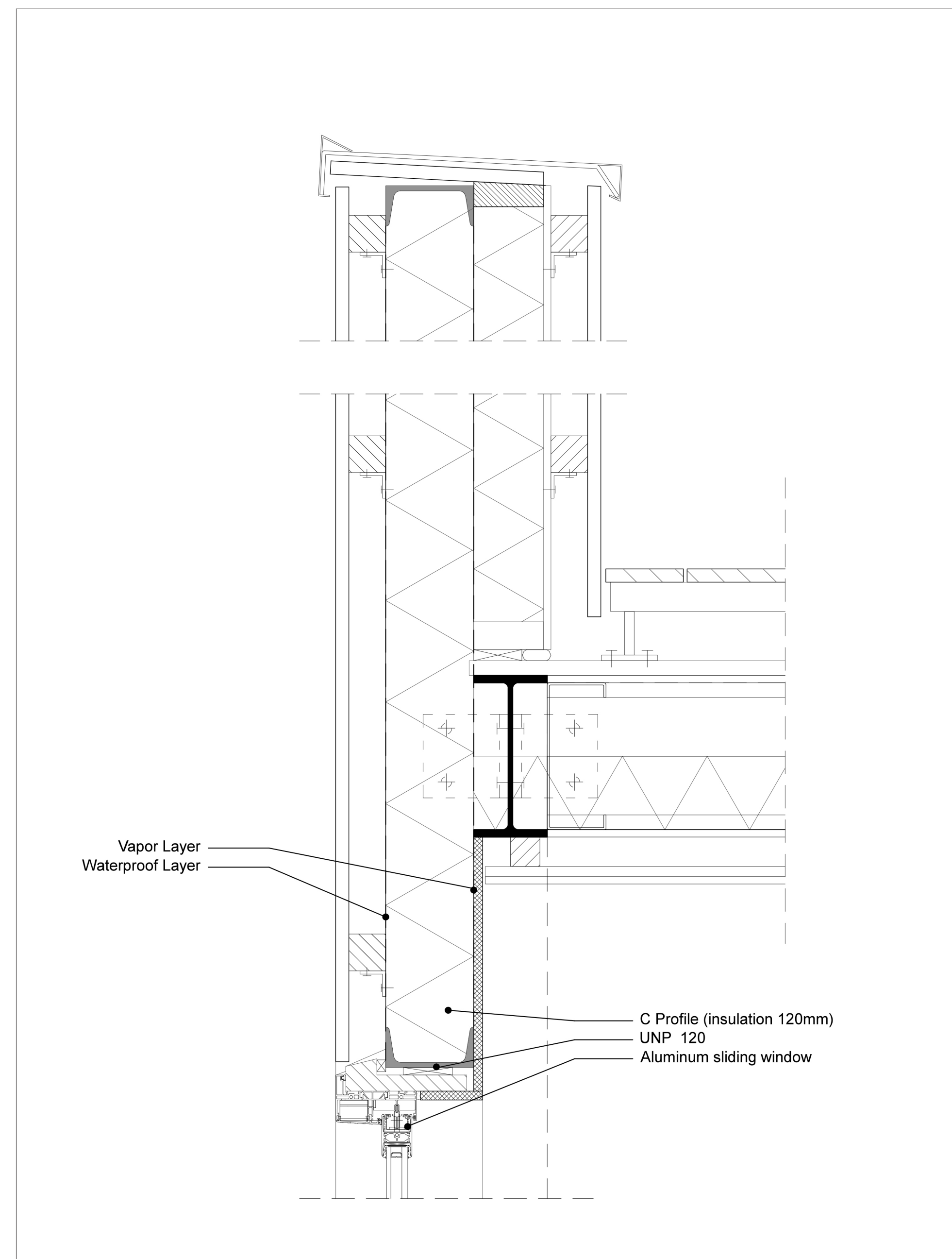
Detail 01 1:5
