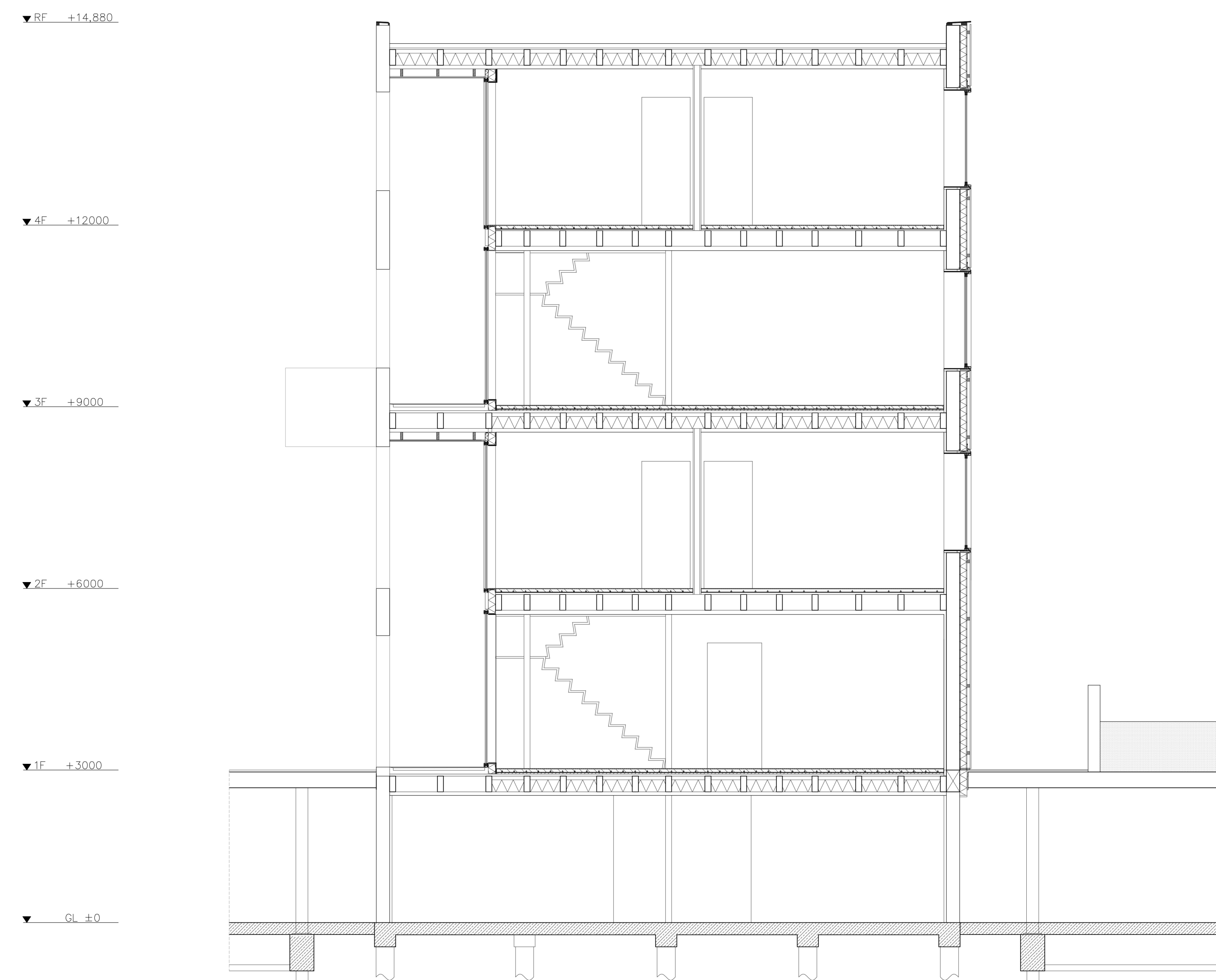
Section 1:50
