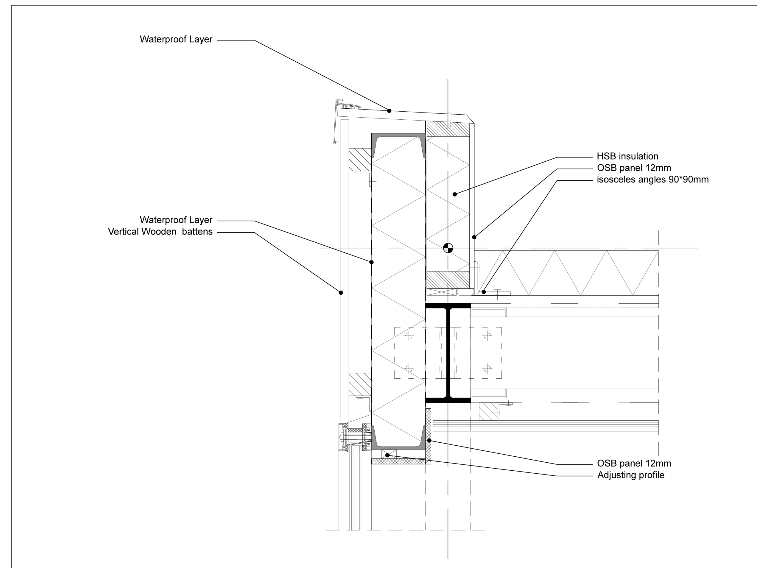
Detail 02 1:5
