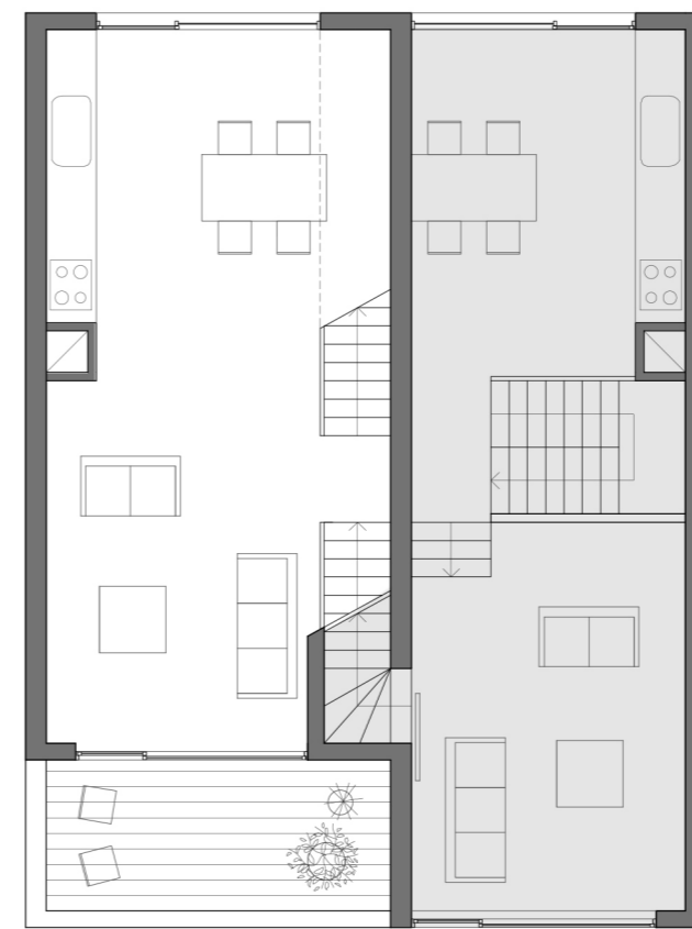
Second Floor Plan 1:100
