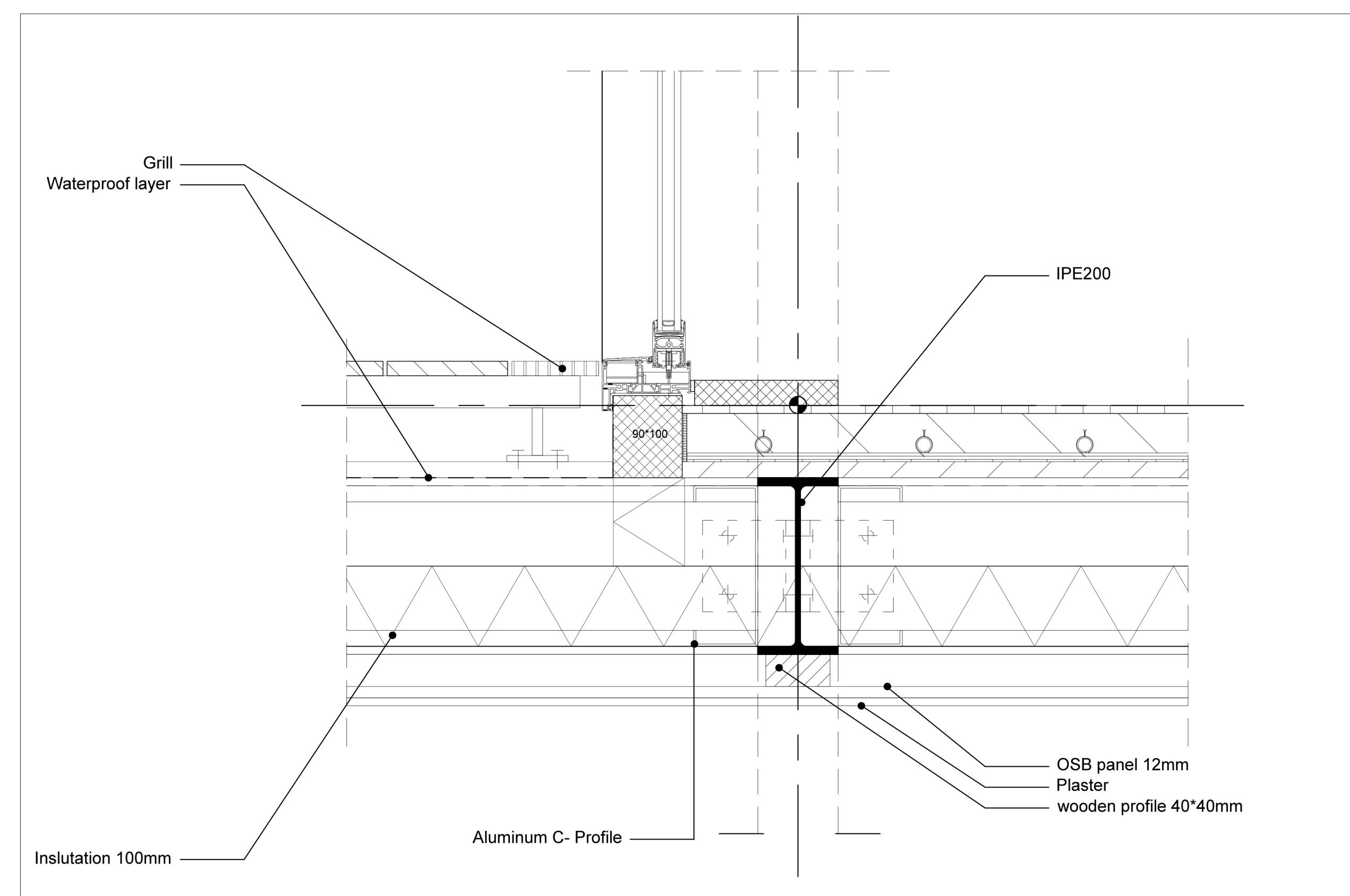
Detail 03 1:5
